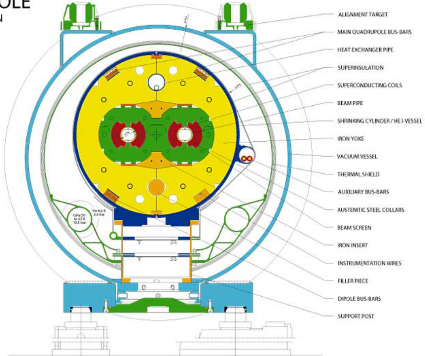
Figure 31: LHC dipole cross-section (note two pipes for proton beams)
