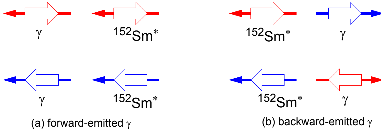
Figure 81: Forward-emitted \gamma has the same helicity as v_e
