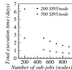
Figure 4: Execution time for full simulation at the Tier1.
