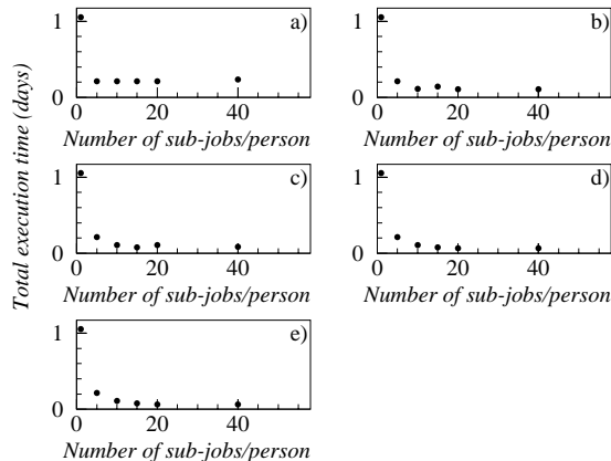
Figure 2: Total execution time for the analysis of AOD data at Tier2, configured with different amount of nodes: a) 100 nodes, b) 200 nodes, c) 300 nodes, d) 400 nodes and e) 800 nodes.
