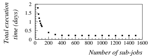
Figure 1: Total execution time for the reconstruction of the data at CERN.
