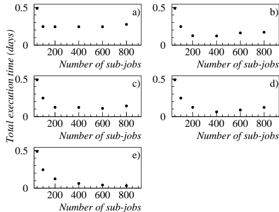
Figure 3: Total execution time for the fast simulation of AOD data at Tier2, configured with different amount of nodes: a) 100 nodes, b) 200 nodes, c) 300 nodes, d) 400 nodes and e) 800 nodes.
