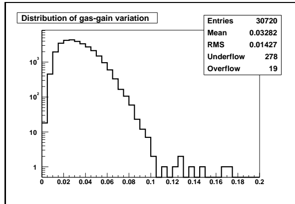
Fig. 10. For all straws of the first five assembled 8-plane end-cap wheels, distribution of the relative variation of gas-gain along each straw. The entries in the underflow bin correspond to dead or unstable channels, which are still under investigation.
