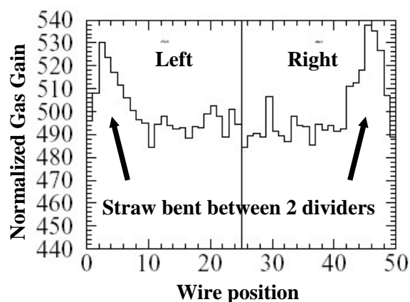
Fig. 7. Results from the X-ray gain mapping for two abnormal straws. One straw (top) has its left-hand wire segment hung at the central wire support. The second straw (bottom) is bent between two dividers.
