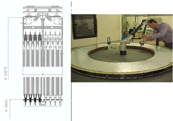
Fig. 8. Drawing of the detailed layout of a type-A 8-plane wheel (left) and photograph of one of the wheels assembled in Russia and under tests at CERN.
