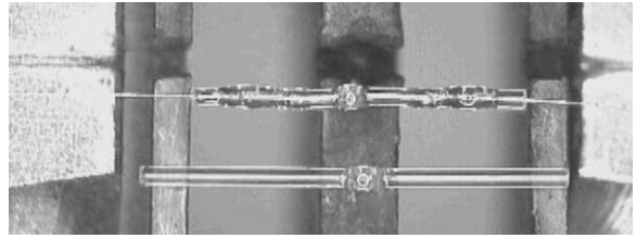
Fig. 6. Photographs of a glass tube melted in its centre and used to make the wire-joints (bottom) and of a finished glass wire-joint (top).
