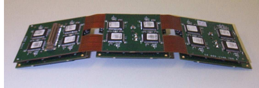
Fig. 12. TRT end-cap front-end electronics printed-circuit boards. Shown is one set of three analogue boards and one digital board, which handles 192 channels.
