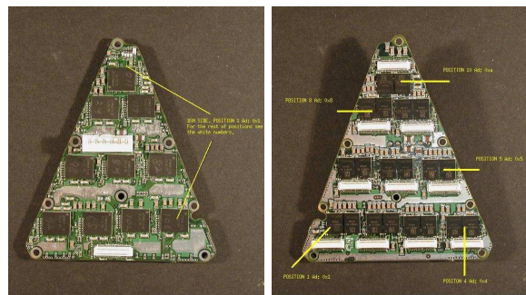
Fig. 13. TRT barrel front-end electronics printed-circuit board.
