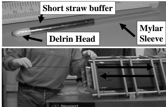
Fig. 5. Photograph of straw insertion bullet (top) and of the insertion of a straw (bottom). The arrows indicate the insertion sequence.
