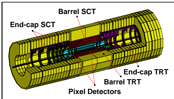
Fig. 1. Perspective view of the ATLAS Inner Detector with its three sub-systems: the Pixel detector at the innermost radii, the Semi-Conductor Tracker (SCT) at the intermediate radii, and the TRT at the outermost radii. The barrel TRT contains 52,544 axial straws of 144 cm length and each end-cap TRT contains 159,744 straws of 37 to 53 cm length.
