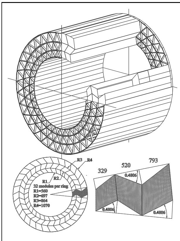
Fig. 2. Layout of the barrel TRT with its three concentric rings of 32 identical modules each. Also shown at one end is the barrel support structure, which will hold all the modules in place within the ATLAS barrel cryostat.
