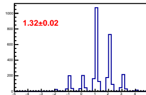
Cross-talk distribution in channel 5
