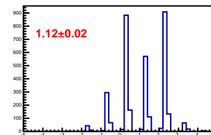
Cross-talk distribution in channel 15
