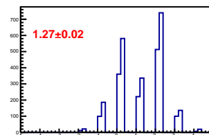
Cross-talk distribution in channel 21
