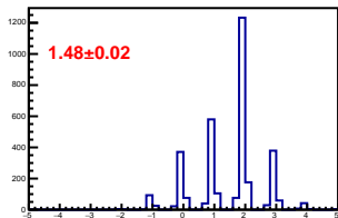
Cross-talk distribution in channel 1
