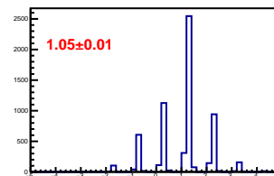
Cross-talk distribution in channel 31
