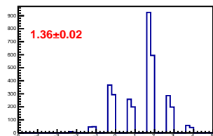
Cross-talk distribution in channel 25
