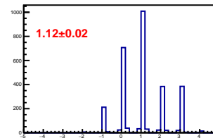
Cross-talk distribution in channel 7
