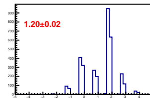
Cross-talk distribution in channel 14
