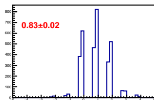
Cross-talk distribution in channel 16
