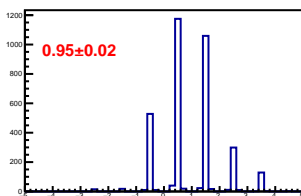
Cross-talk distribution in channel 24
