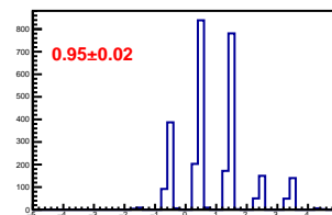
Cross-talk distribution in channel 20
