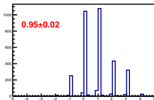
Cross-talk distribution in channel 0
