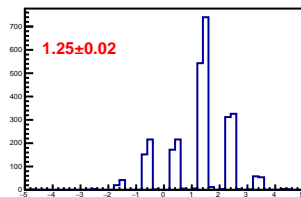
Cross-talk distribution in channel 8
