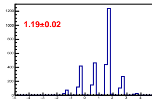
Cross-talk distribution in channel 4
