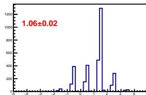
Cross-talk distribution in channel 10
