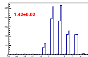
Cross-talk distribution in channel 6
