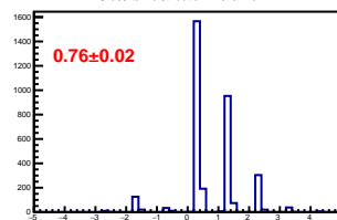
Cross-talk distribution in channel 14
