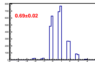
Cross-talk distribution in channel 22
