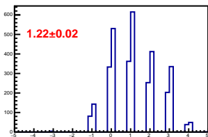
Cross-talk distribution in channel 9
