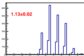
Cross-talk distribution in channel 21
