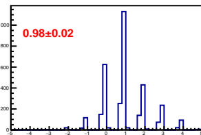
Cross-talk distribution in channel 3
