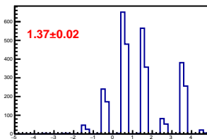
Cross-talk distribution in channel 13
