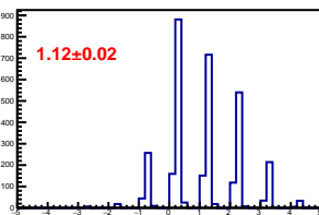
Cross-talk distribution in channel 27
