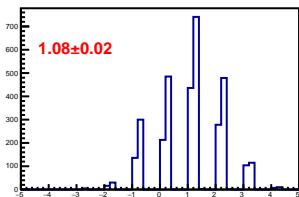
Cross-talk distribution in channel 1
