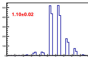
Cross-talk distribution in channel 23
