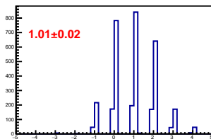
Cross-talk distribution in channel 15
