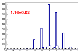
Cross-talk distribution in channel 7
