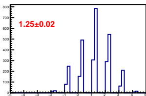
Cross-talk distribution in channel 25
