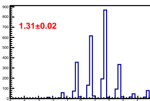
Cross-talk distribution in channel 20
