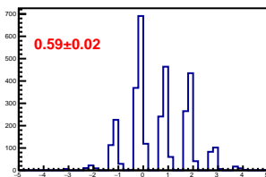
Cross-talk distribution in channel 0
