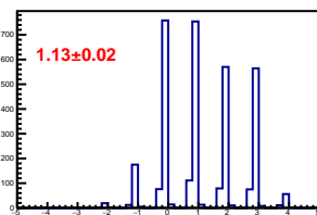
Cross-talk distribution in channel 26
