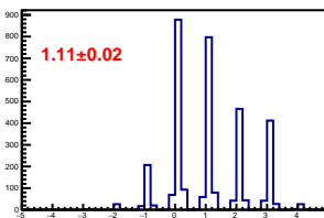
Cross-talk distribution in channel 4
