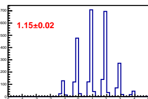
Cross-talk distribution in channel 18
