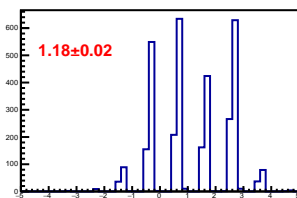
Cross-talk distribution in channel 24
