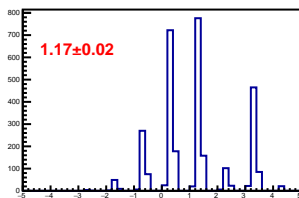
Cross-talk distribution in channel 14
