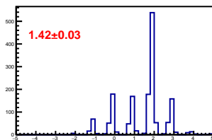
Cross-talk distribution in channel 6
