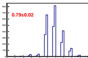
Cross-talk distribution in channel 22
