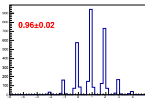
Cross-talk distribution in channel 28
