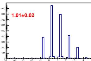
Cross-talk distribution in channel 12
