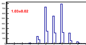
Cross-talk distribution in channel 0
