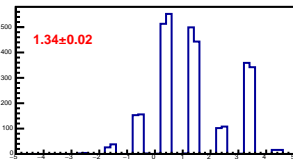
Cross-talk distribution in channel 10
