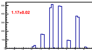
Cross-talk distribution in channel 14
