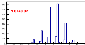
Cross-talk distribution in channel 8
