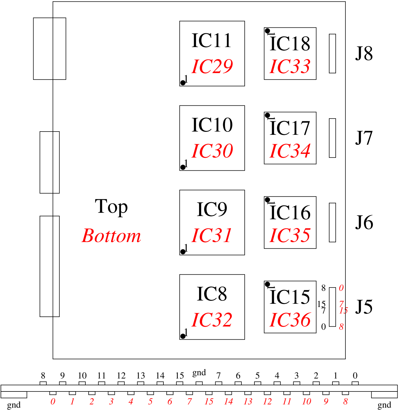
Cable seen as comming out from detector
