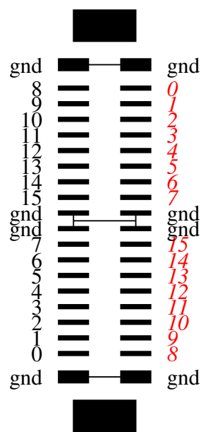
Connector on FEC seen from top
