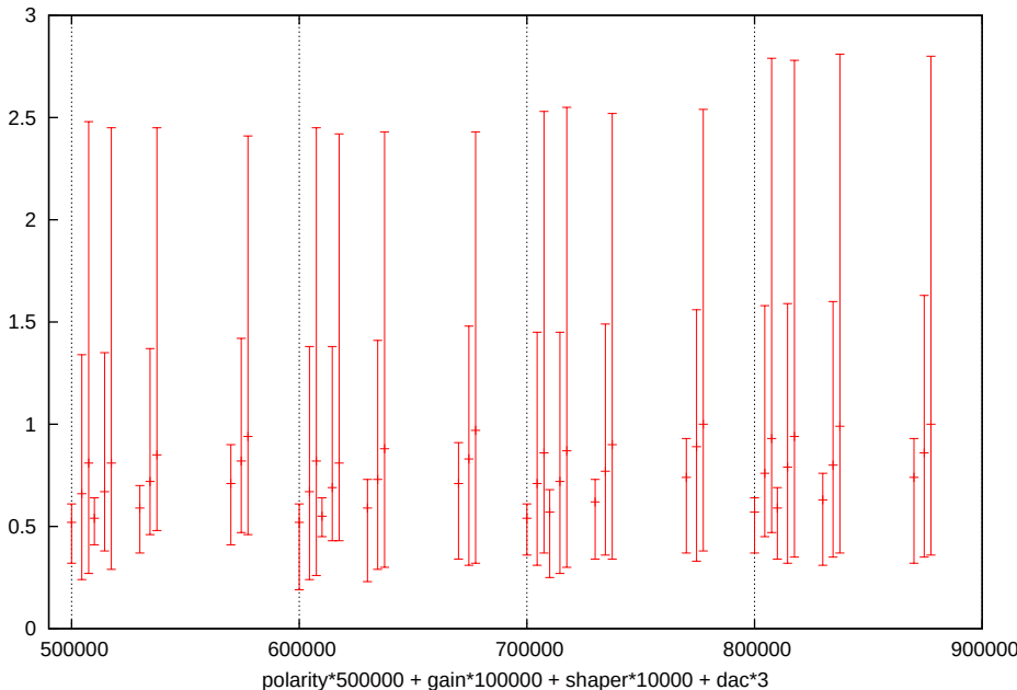
VREF=1200, 2500 voltage power supplies, cables connected shielded, noshaper
