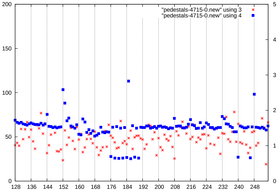
p1-gain3-shaper0-dac1500
