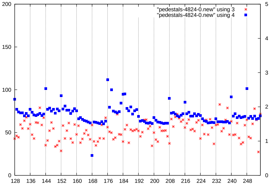
p1-gain3-shaper1-dac2500
