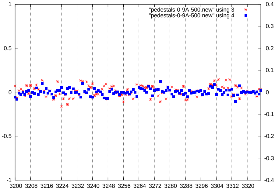
p1-gain1-shaper3-dac500
