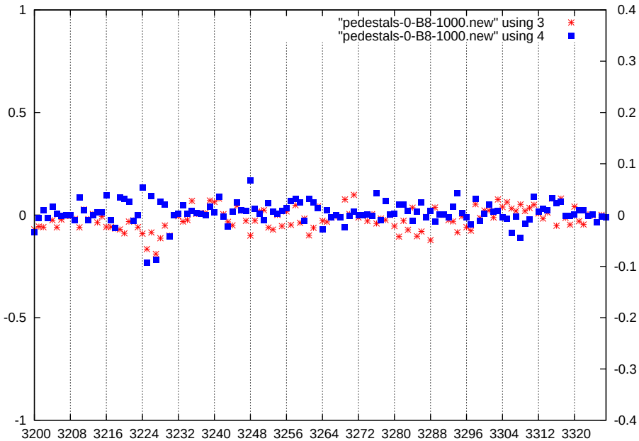
p1-gain0-shaper7-dac1000
