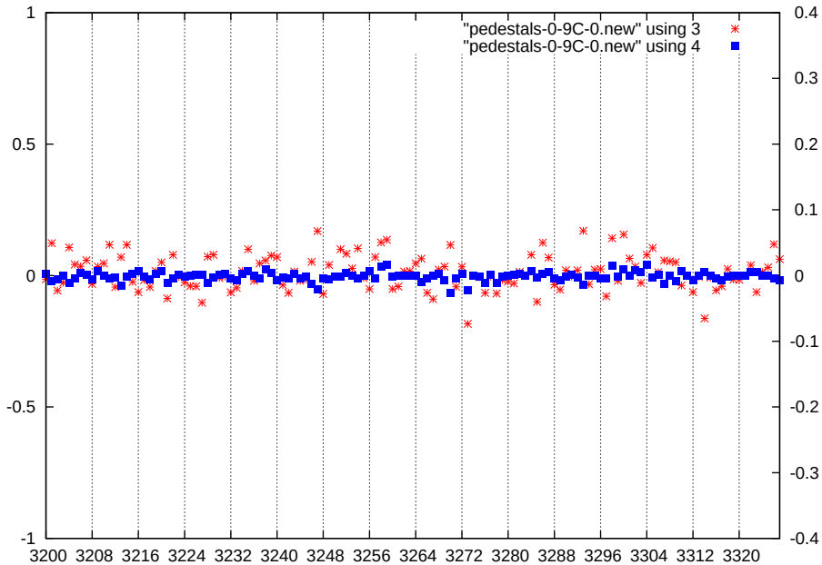
p1-gain2-shaper3-dac0
