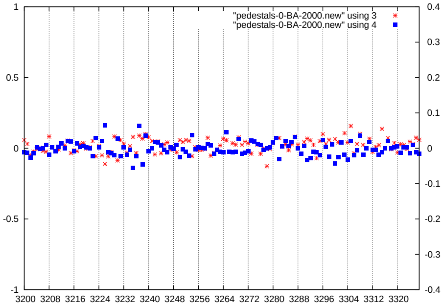
p1-gain1-shaper7-dac2000
