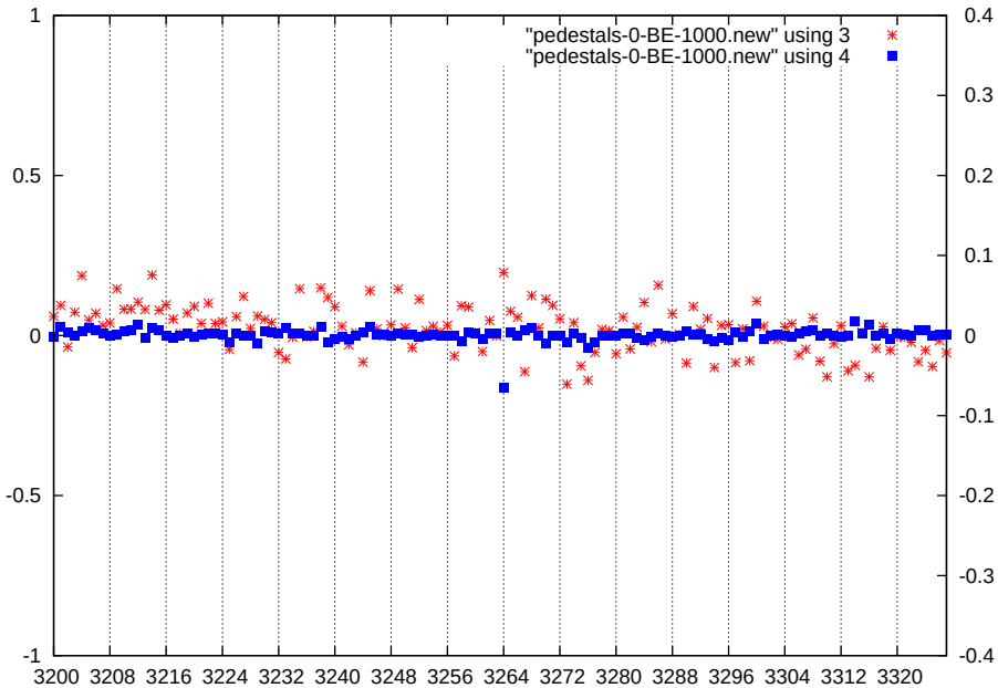
p1-gain3-shaper7-dac1000
