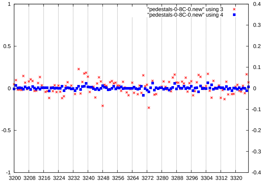
p1-gain2-shaper1-dac0
