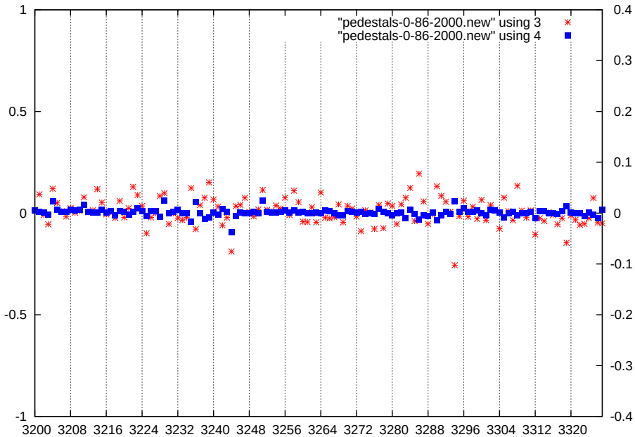
p1-gain3-shaper0-dac2000
