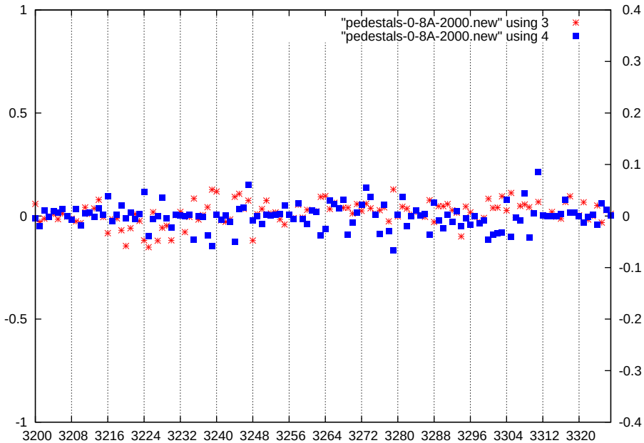
p1-gain1-shaper1-dac2000
