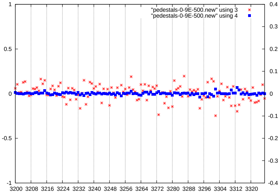
p1-gain3-shaper3-dac500
