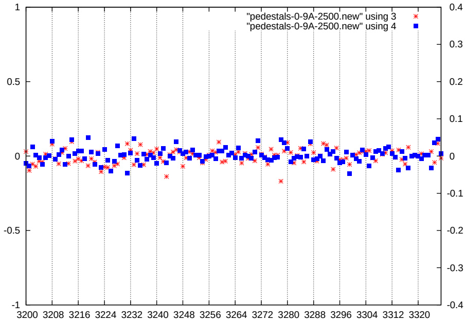
p1-gain1-shaper3-dac2500
