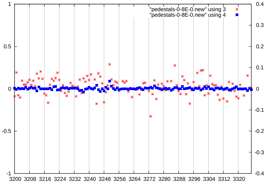
p1-gain3-shaper1-dac0
