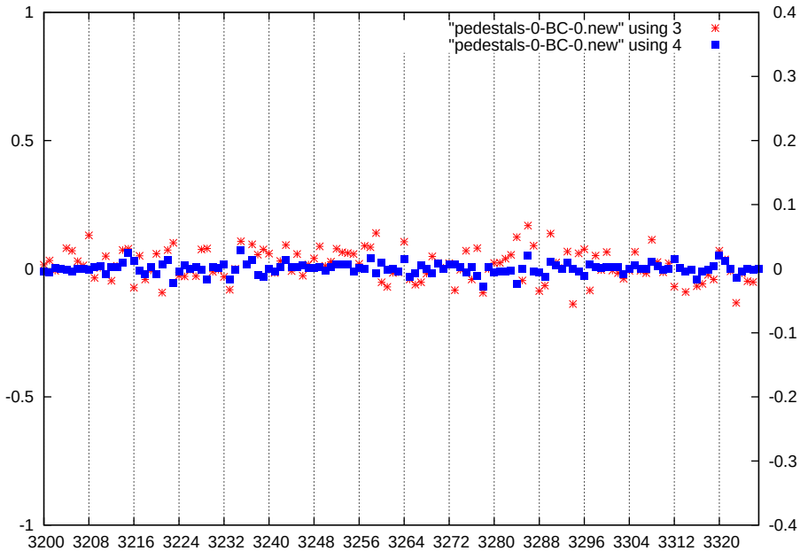
p1-gain2-shaper7-dac0
