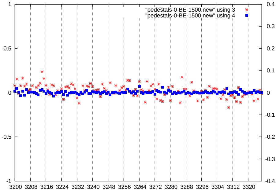
p1-gain3-shaper7-dac1500
