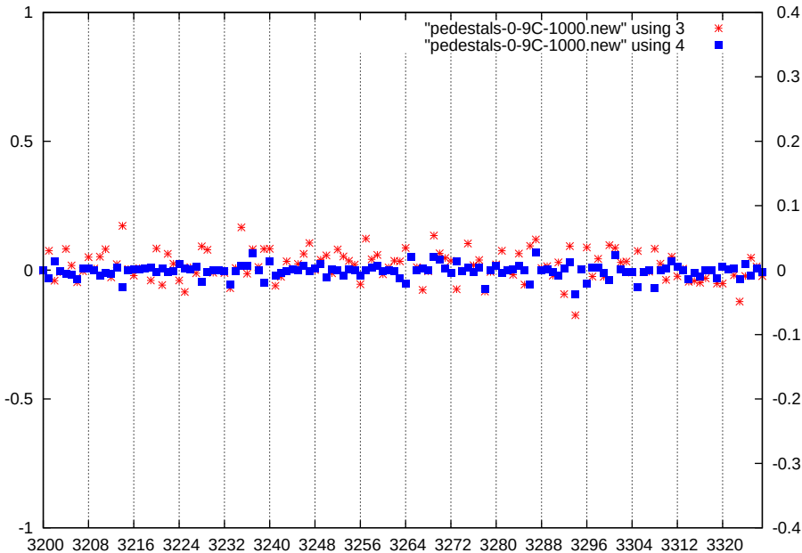
p1-gain2-shaper3-dac1000
