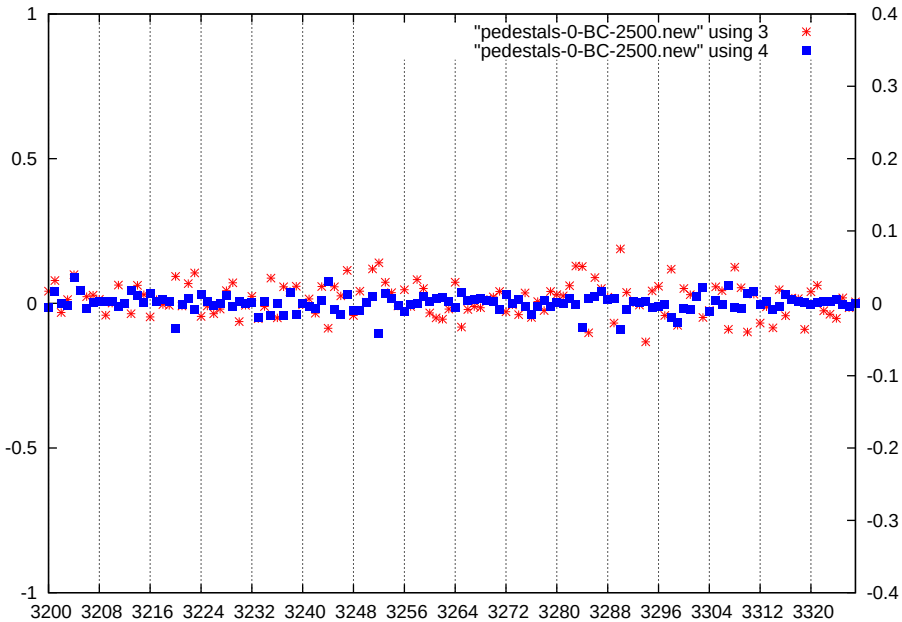
p1-gain2-shaper7-dac2500
