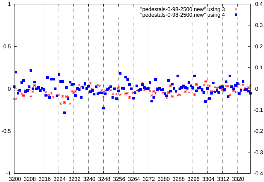
p1-gain0-shaper3-dac2500
