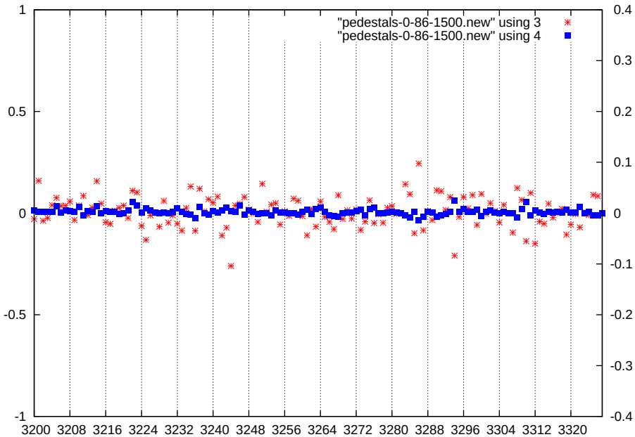
p1-gain3-shaper0-dac1500
