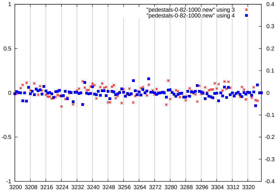
p1-gain1-shaper0-dac1000
