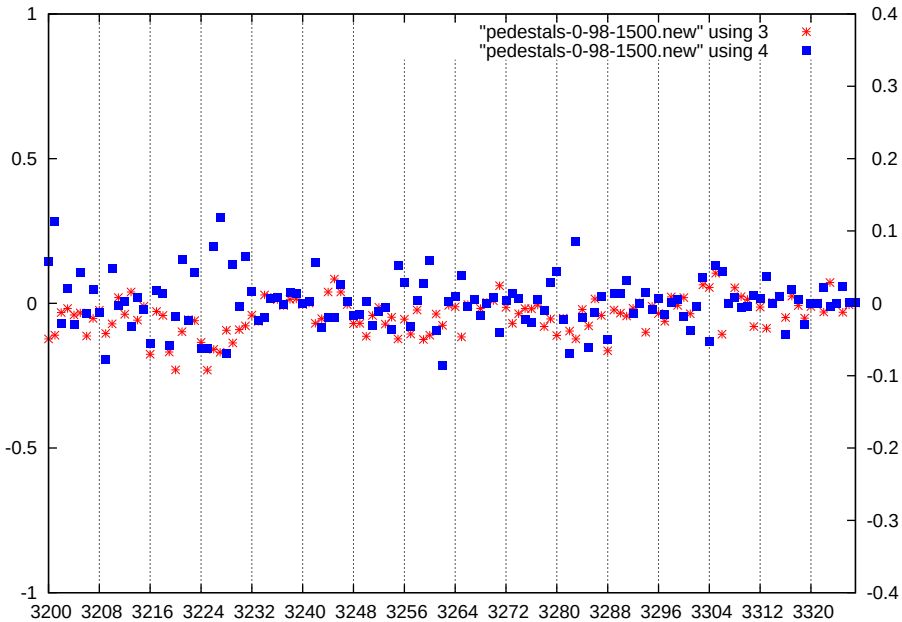
p1-gain0-shaper3-dac1500
