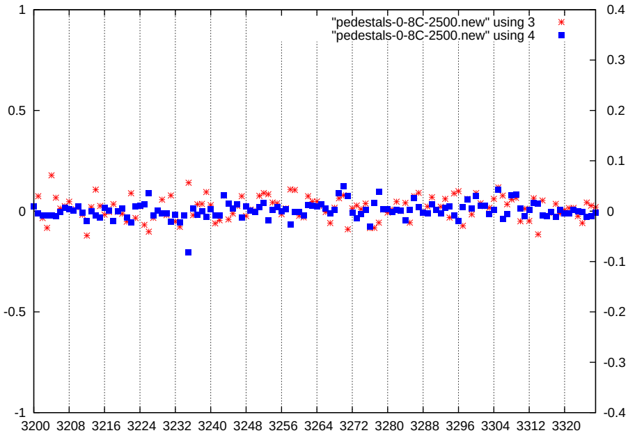
p1-gain2-shaper1-dac2500
