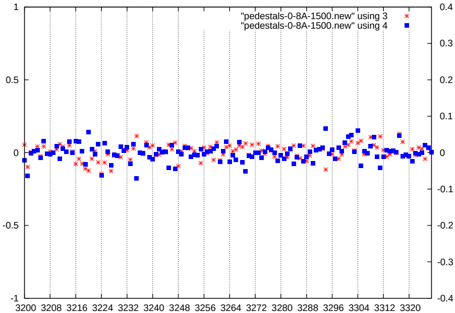
p1-gain1-shaper1-dac1500
