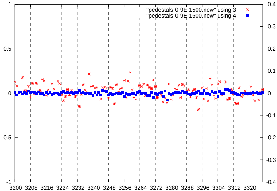
p1-gain3-shaper3-dac1500
