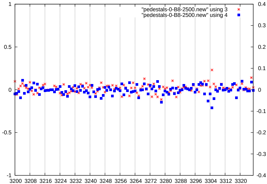
p1-gain0-shaper7-dac2500
