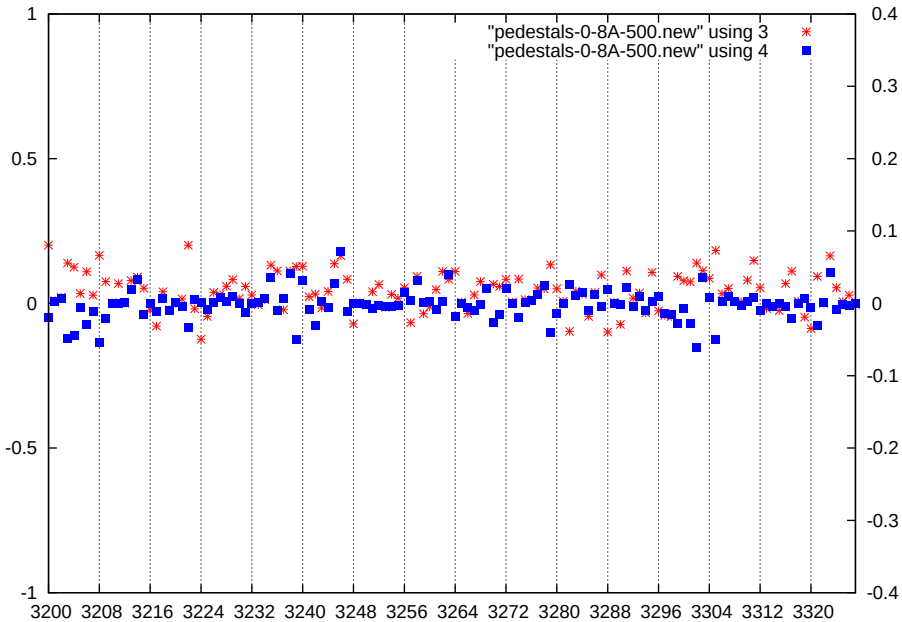
p1-gain1-shaper1-dac500
