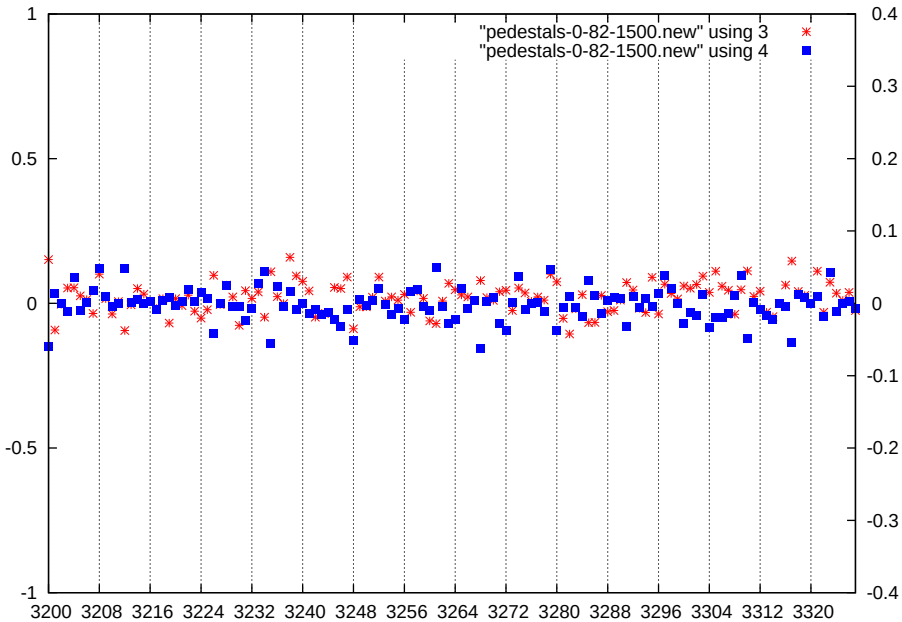
p1-gain1-shaper0-dac1500
