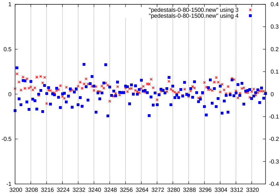
p1-gain0-shaper0-dac1500
