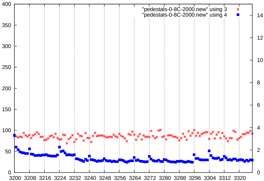
p1-gain2-shaper1-dac2000
