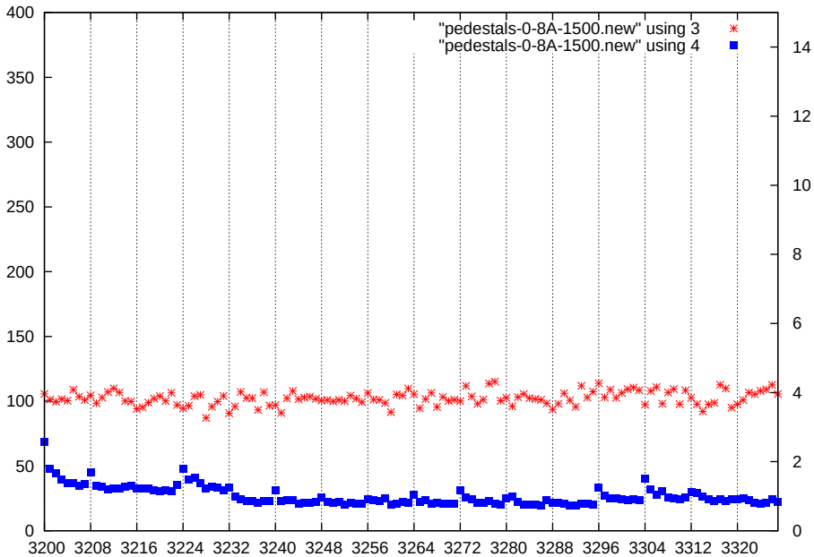
p1-gain1-shaper1-dac1500
