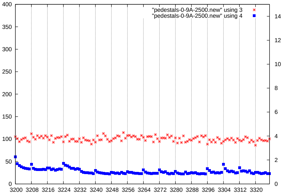
p1-gain1-shaper3-dac2500
