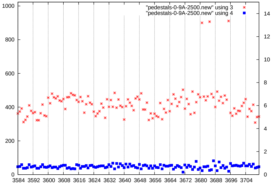
p1-gain1-shaper3-dac2500
