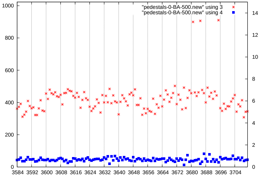
p1-gain1-shaper7-dac500
