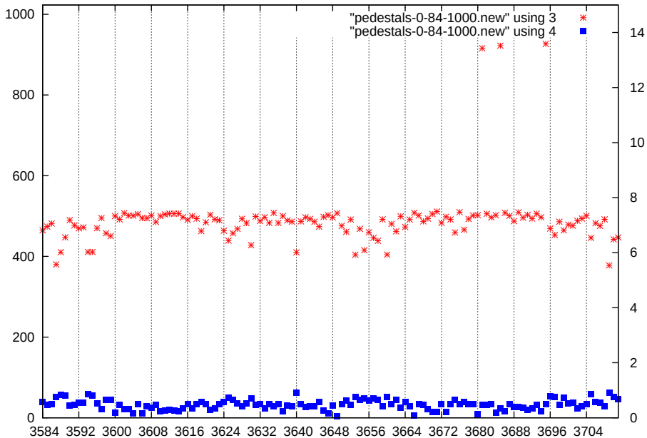
p1-gain2-shaper0-dac1000
