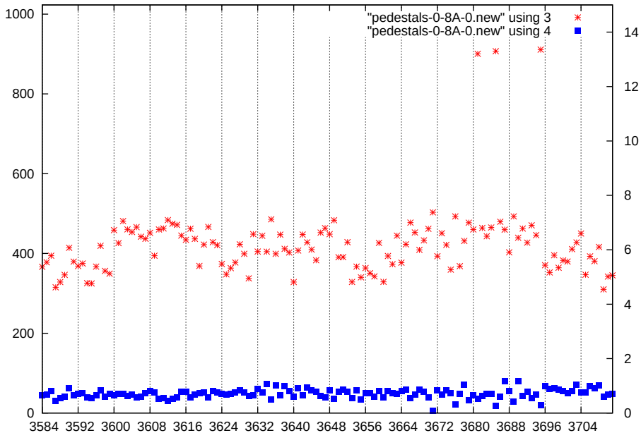
p1-gain1-shaper1-dac0
