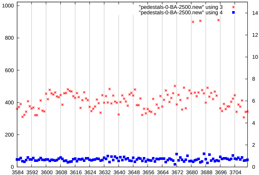
p1-gain1-shaper7-dac2500
