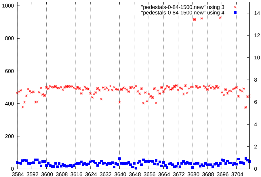
p1-gain2-shaper0-dac1500
