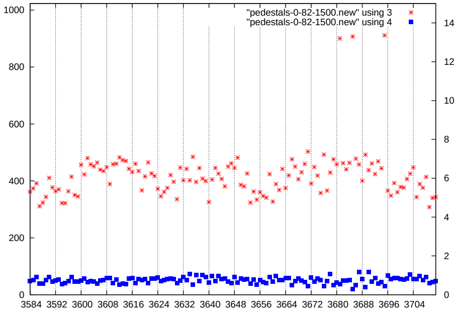
p1-gain1-shaper0-dac1500
