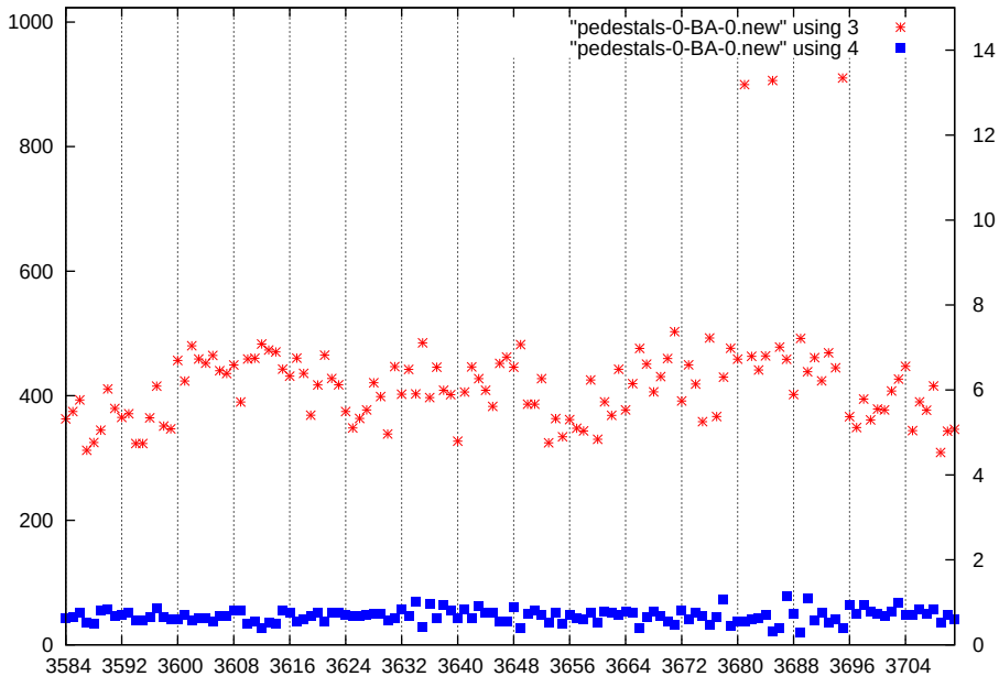
p1-gain1-shaper7-dac0
