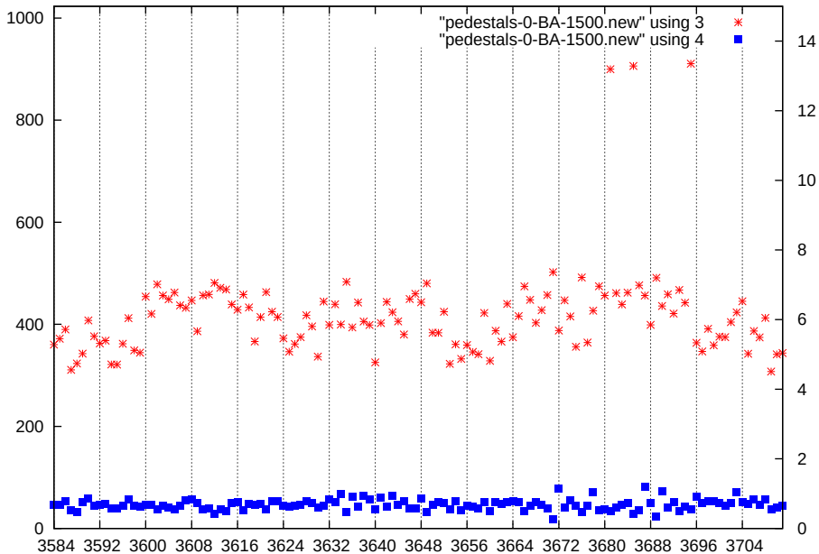
p1-gain1-shaper7-dac1500
