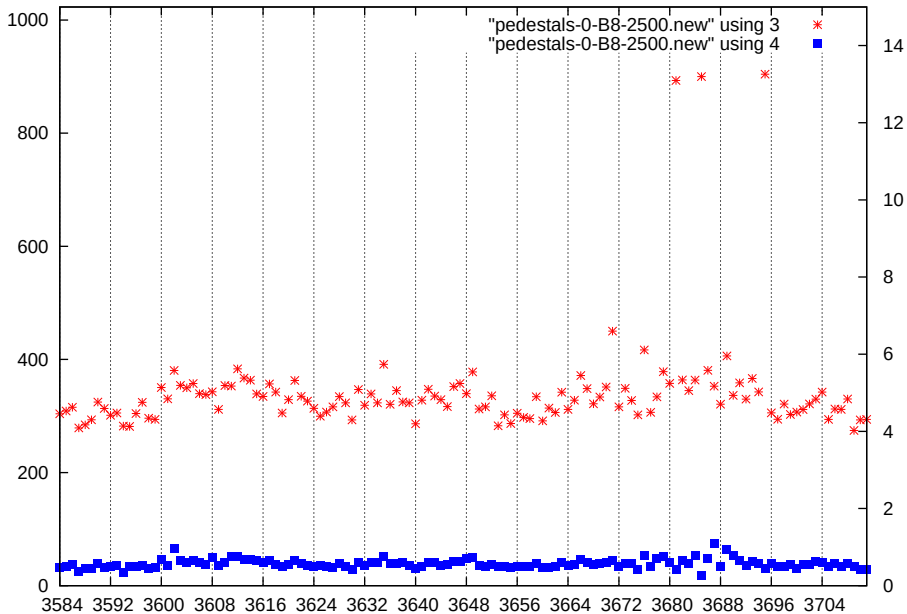
p1-gain0-shaper7-dac2500
