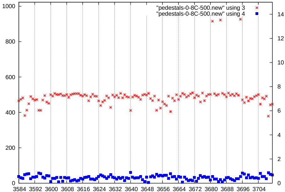
p1-gain2-shaper1-dac500
