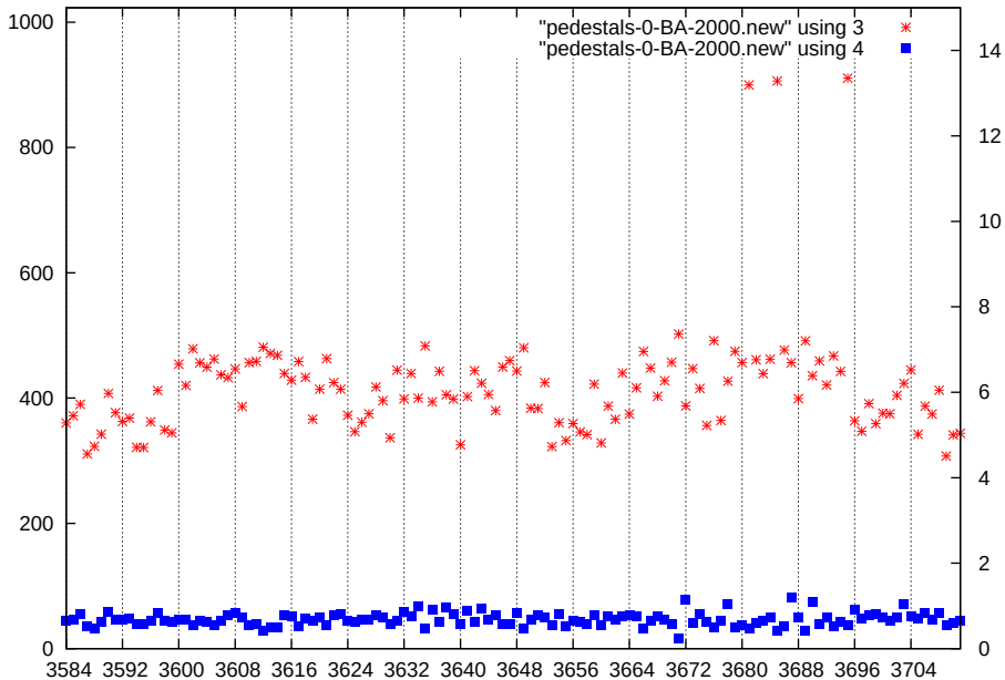
p1-gain1-shaper7-dac2000
