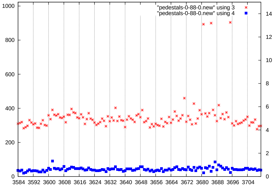
p1-gain0-shaper1-dac0
