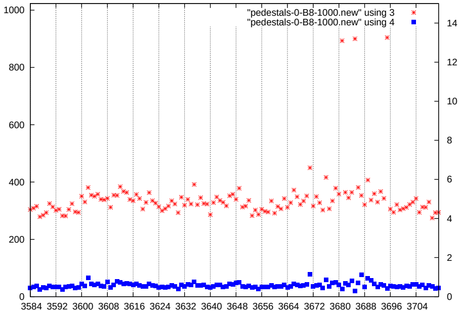
p1-gain0-shaper7-dac1000
