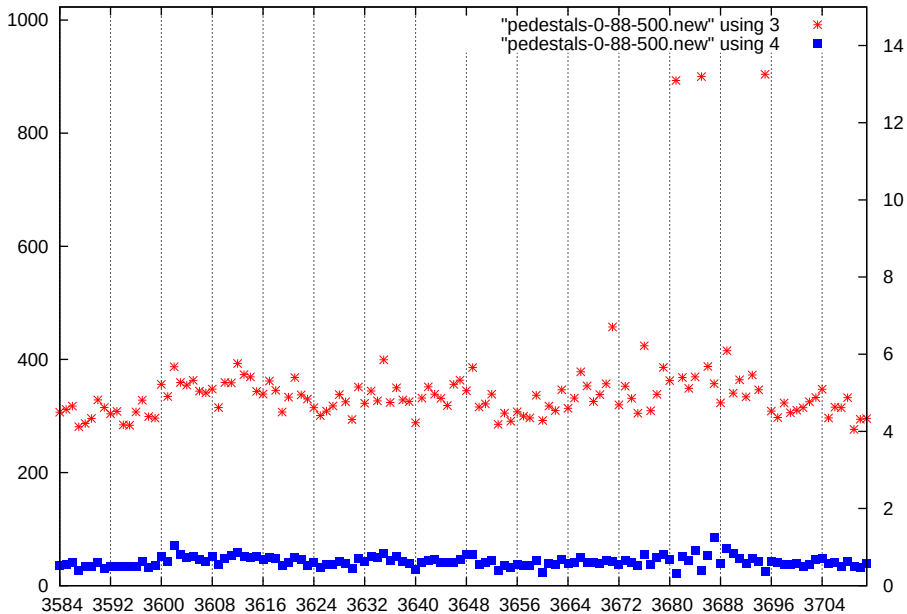
p1-gain0-shaper1-dac500
