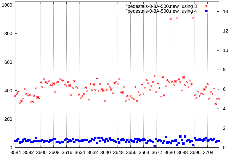
p1-gain1-shaper1-dac500
