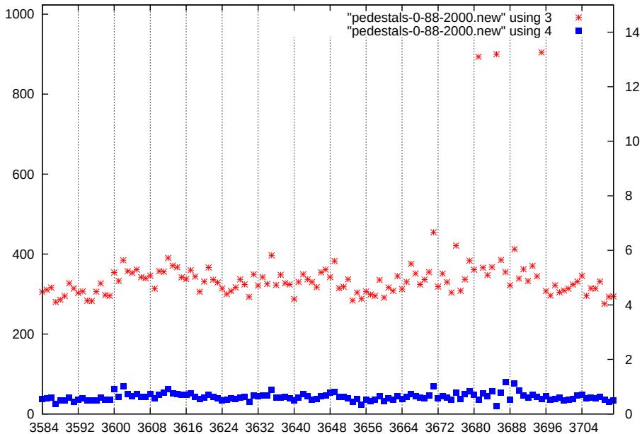
p1-gain0-shaper1-dac2000
