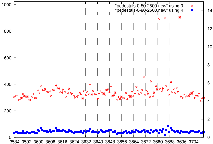
p1-gain0-shaper0-dac2500
