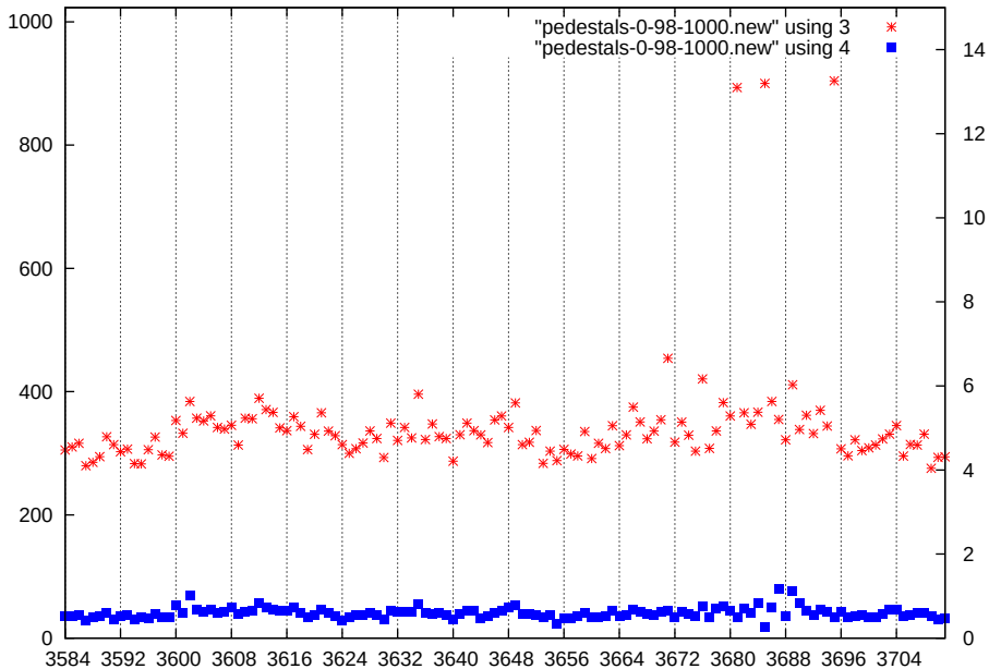
p1-gain0-shaper3-dac1000
