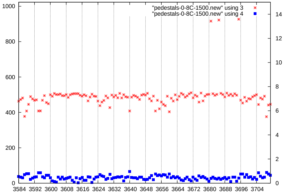
p1-gain2-shaper1-dac1500
