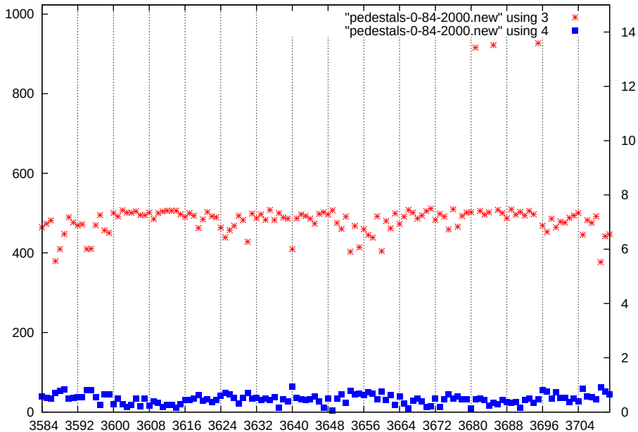
p1-gain2-shaper0-dac2000
