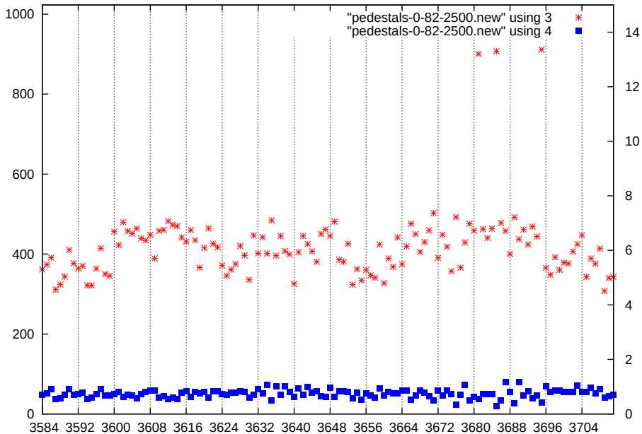
p1-gain1-shaper0-dac2500
