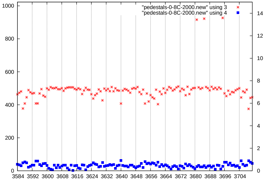
p1-gain2-shaper1-dac2000
