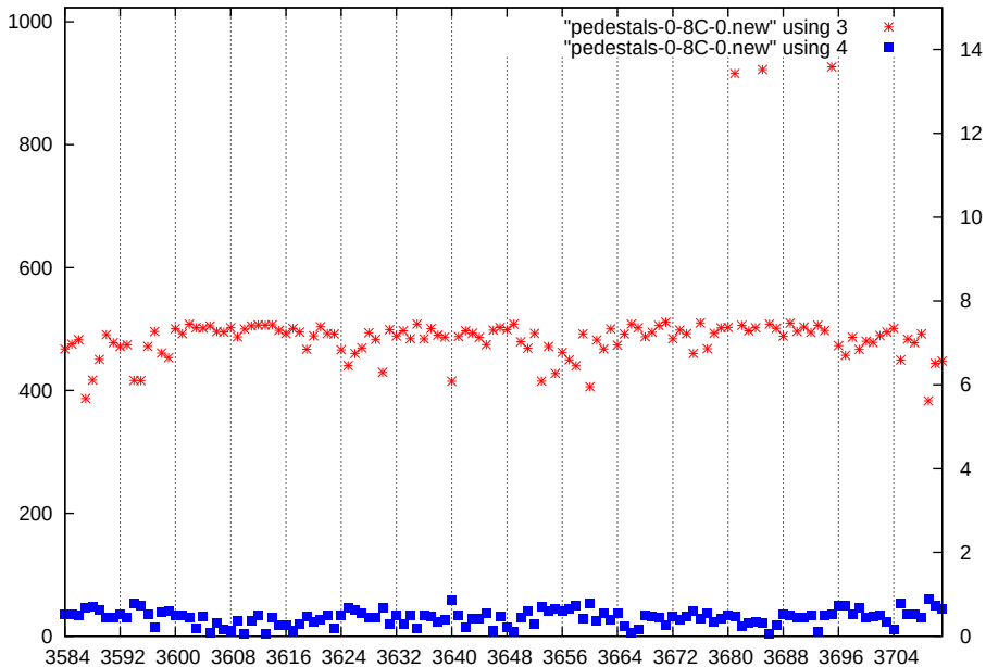
p1-gain2-shaper1-dac0
