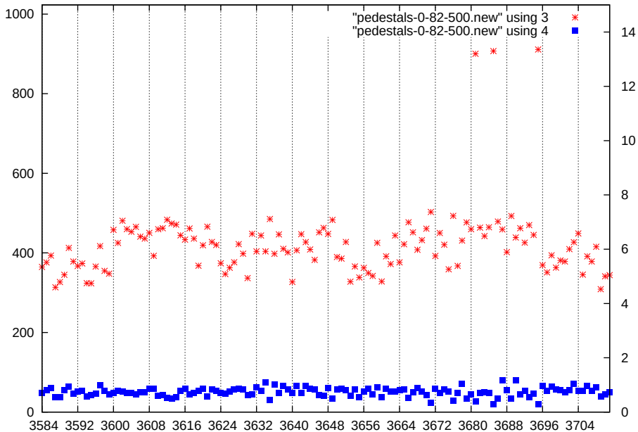
p1-gain1-shaper0-dac500
