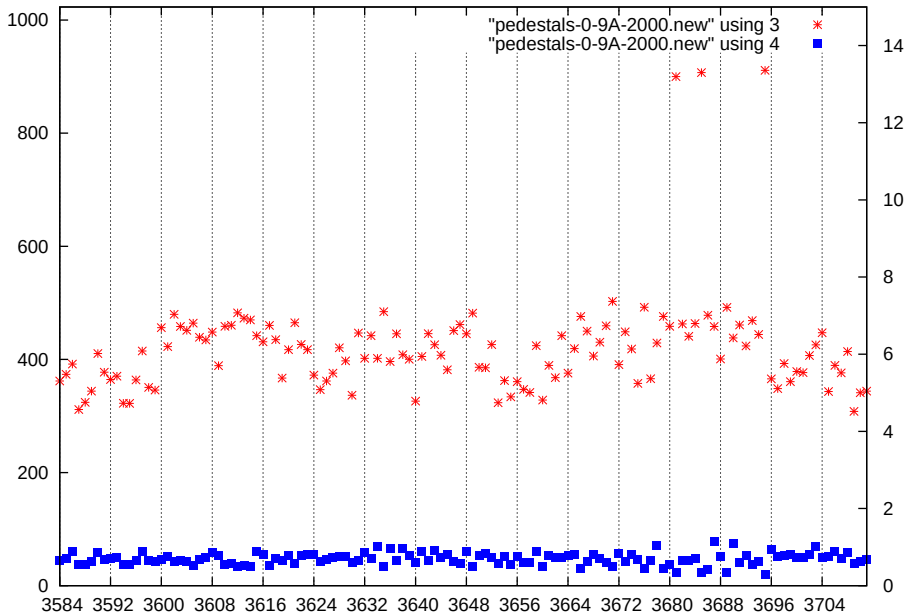
p1-gain1-shaper3-dac2000
