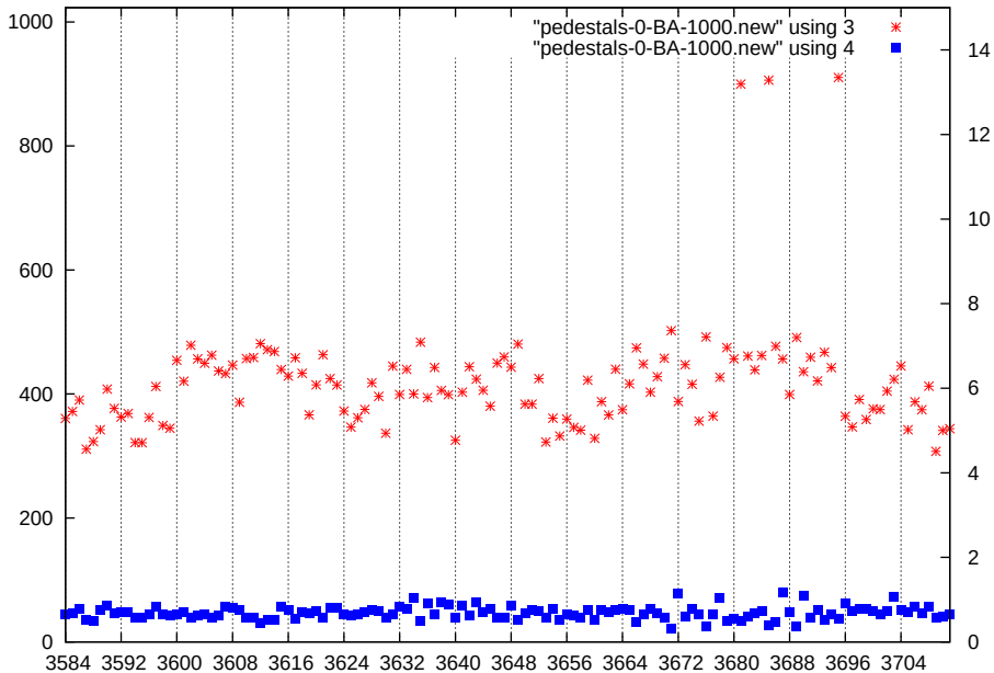
p1-gain1-shaper7-dac1000
