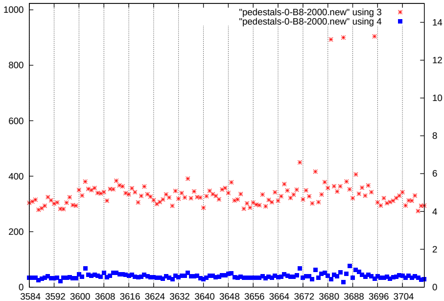
p1-gain0-shaper7-dac2000
