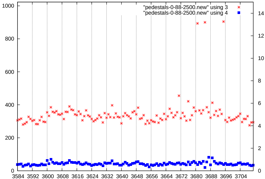
p1-gain0-shaper1-dac2500
