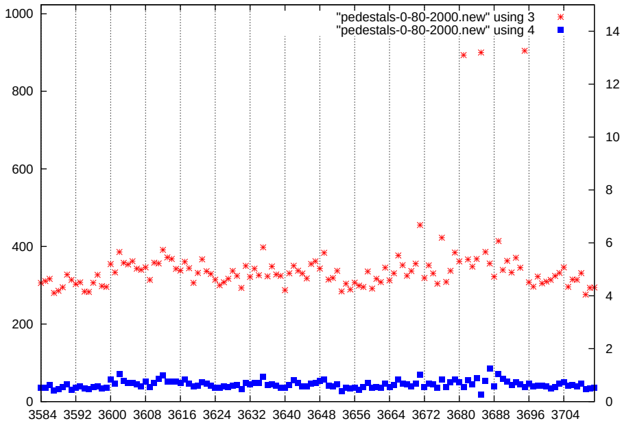
p1-gain0-shaper0-dac2000
