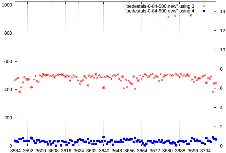
p1-gain2-shaper0-dac500
