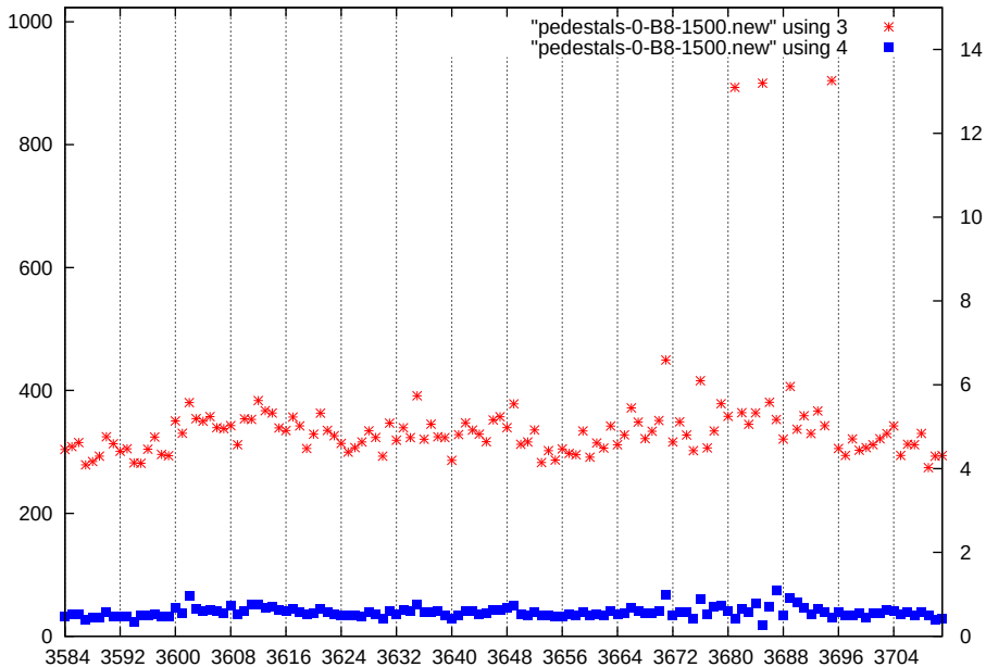
p1-gain0-shaper7-dac1500
