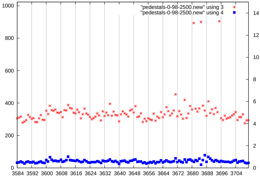
p1-gain0-shaper3-dac2500
