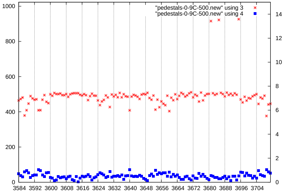
p1-gain2-shaper3-dac500
