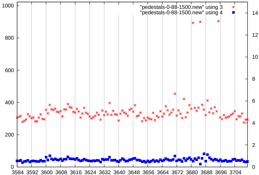
p1-gain0-shaper1-dac1500
