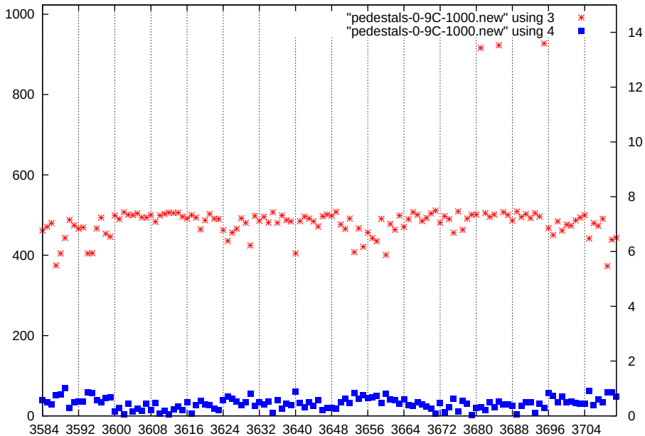
p1-gain2-shaper3-dac1000
