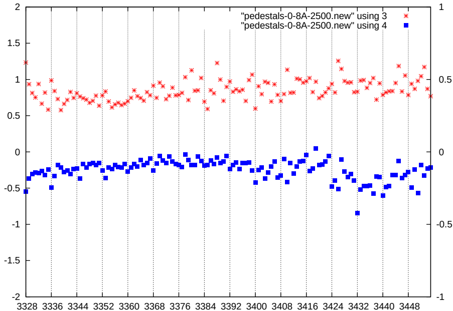
p1-gain1-shaper1-dac2500
