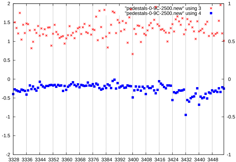
p1-gain2-shaper3-dac2500
