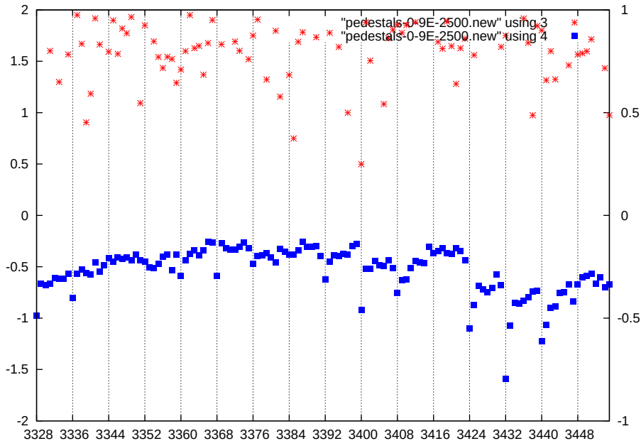
p1-gain3-shaper3-dac2500
