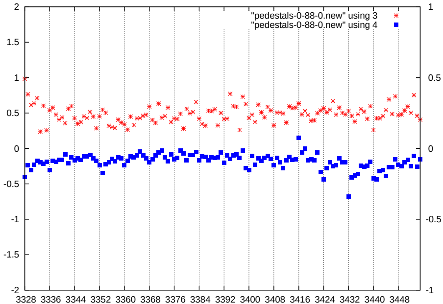
p1-gain0-shaper1-dac0
