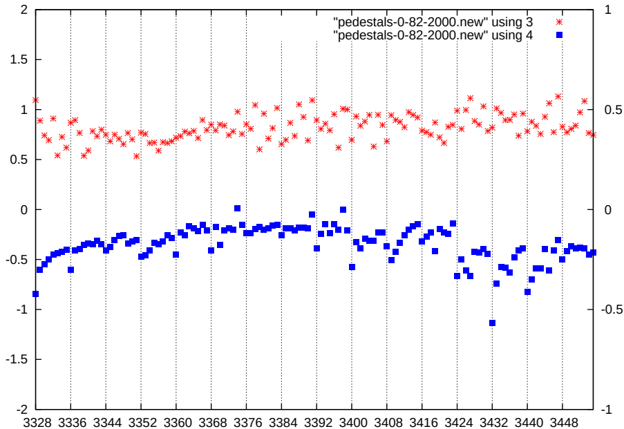
p1-gain1-shaper0-dac2000
