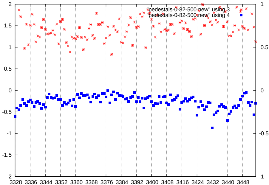
p1-gain1-shaper0-dac500
