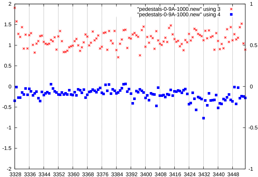
p1-gain1-shaper3-dac1000
