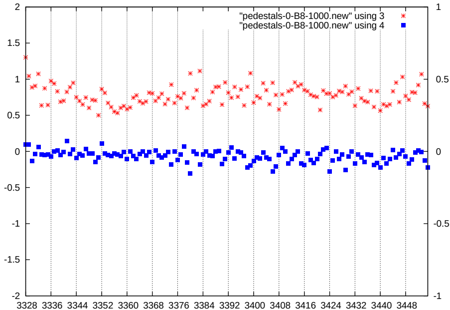
p1-gain0-shaper7-dac1000
