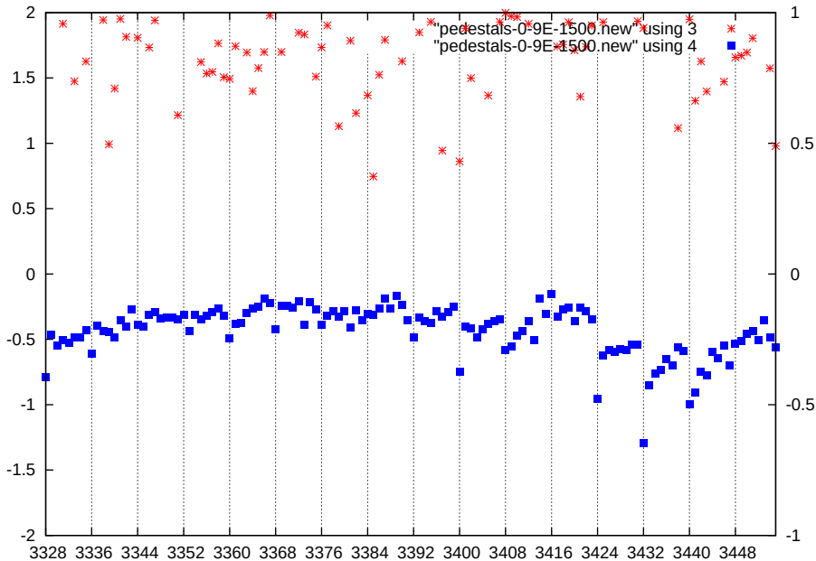
p1-gain3-shaper3-dac1500
