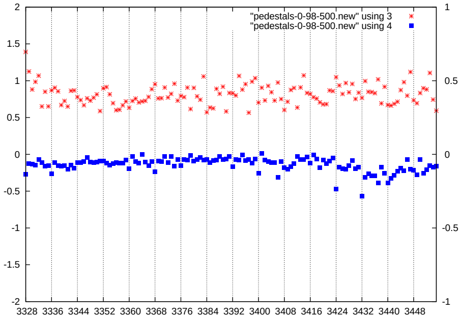
p1-gain0-shaper3-dac500
