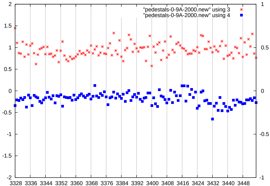
p1-gain1-shaper3-dac2000
