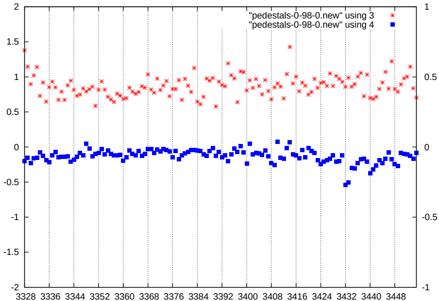
p1-gain0-shaper3-dac0
