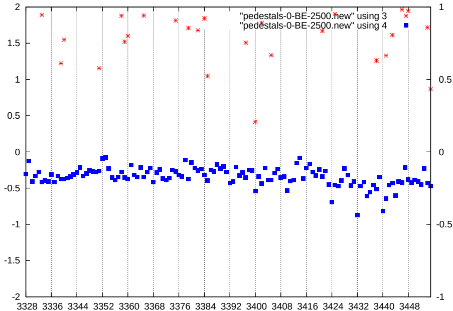
p1-gain3-shaper7-dac2500
