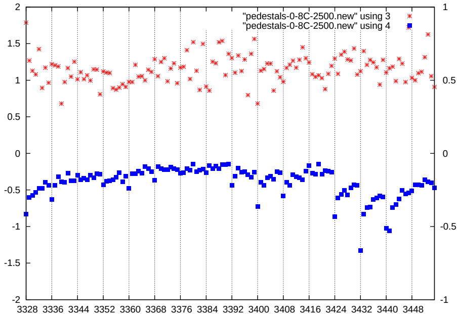
p1-gain2-shaper1-dac2500
