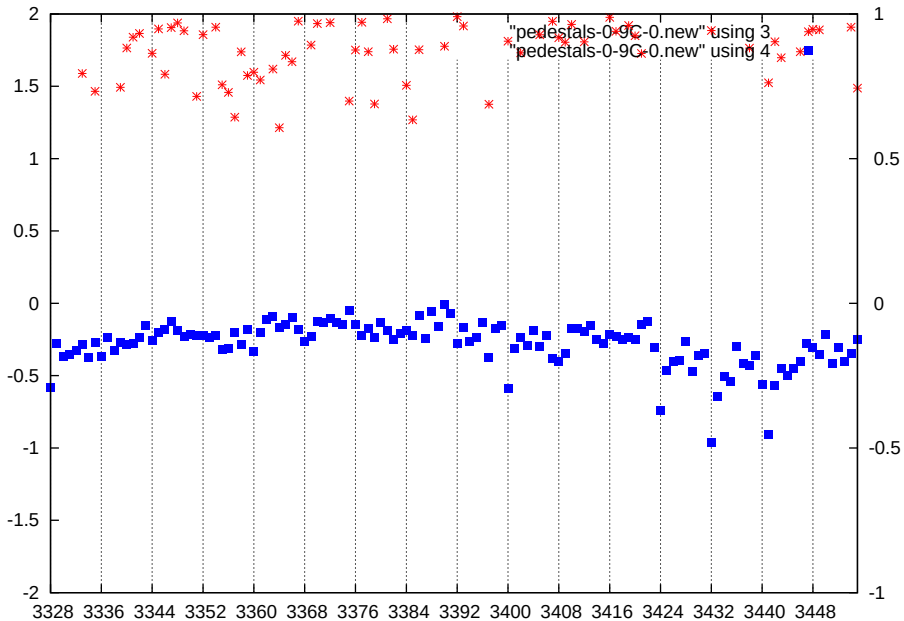
p1-gain2-shaper3-dac0
