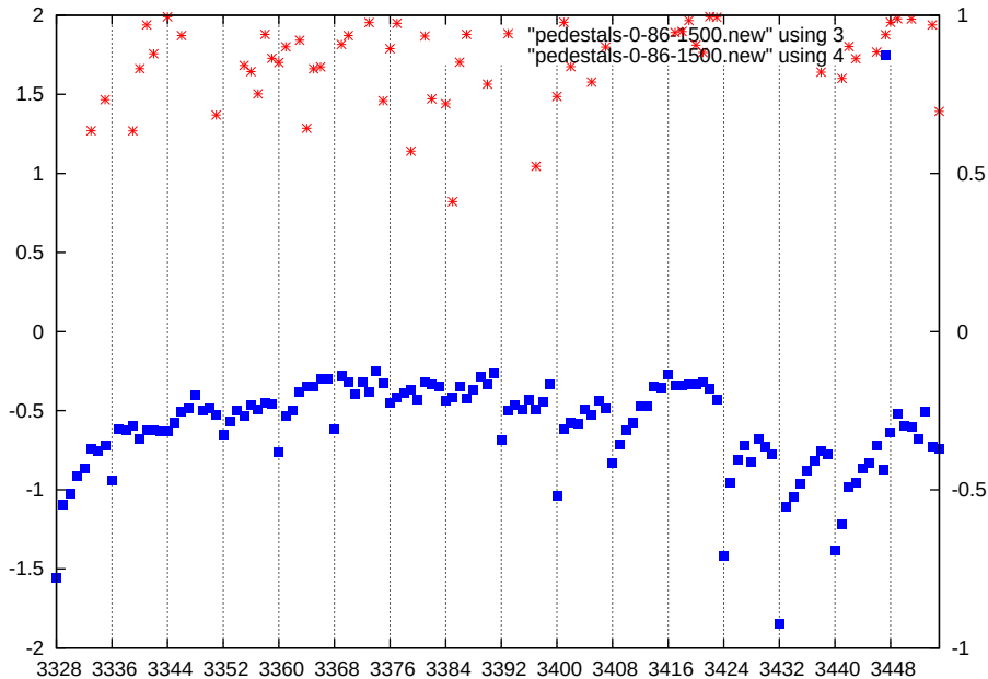
p1-gain3-shaper0-dac1500
