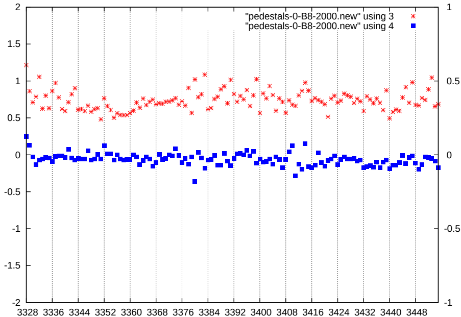
p1-gain0-shaper7-dac2000
