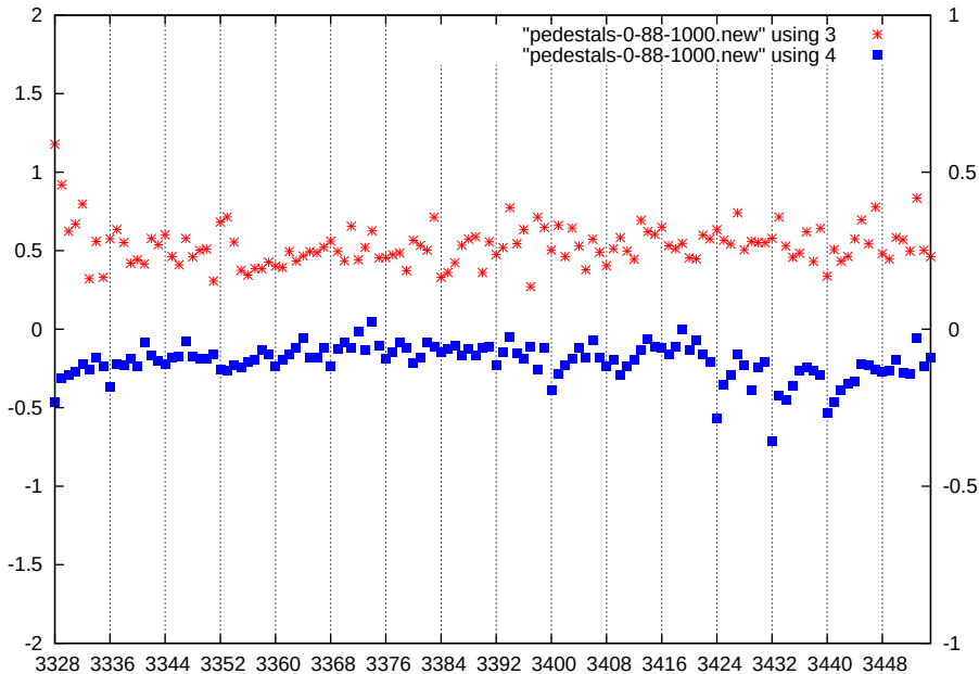
p1-gain0-shaper1-dac1000
