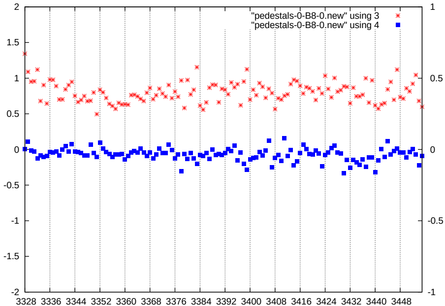
p1-gain0-shaper7-dac0
