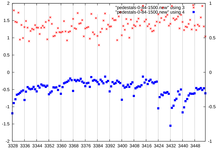
p1-gain2-shaper0-dac1500
