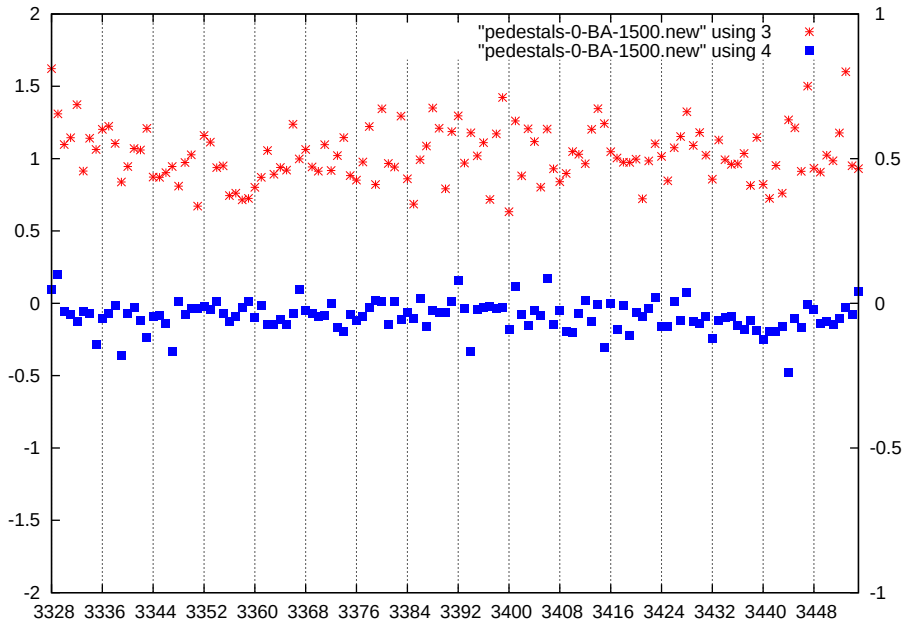
p1-gain1-shaper7-dac1500
