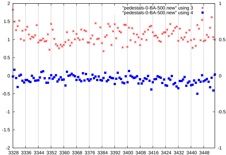
p1-gain1-shaper7-dac500
