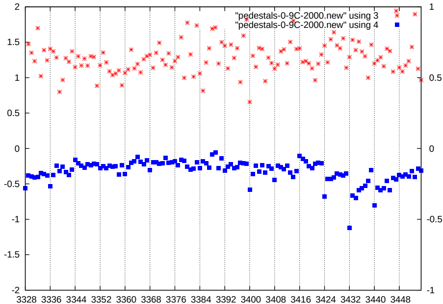
p1-gain2-shaper3-dac2000
