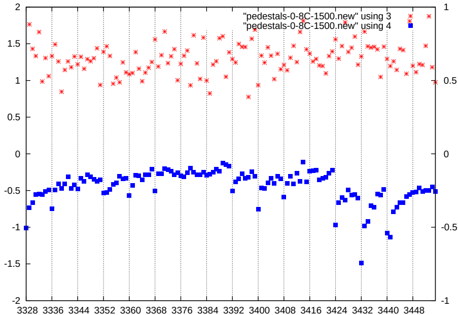
p1-gain2-shaper1-dac1500
