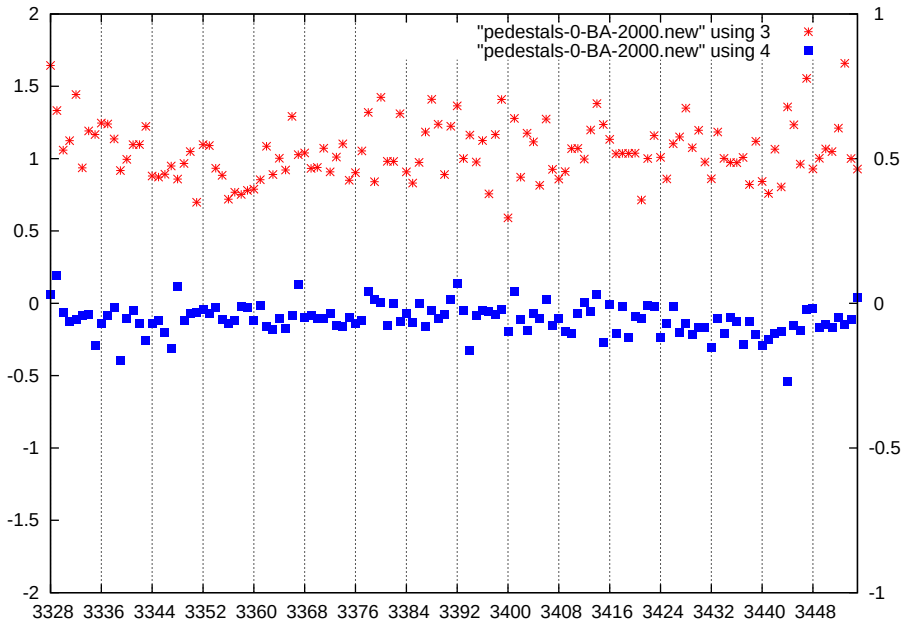
p1-gain1-shaper7-dac2000
