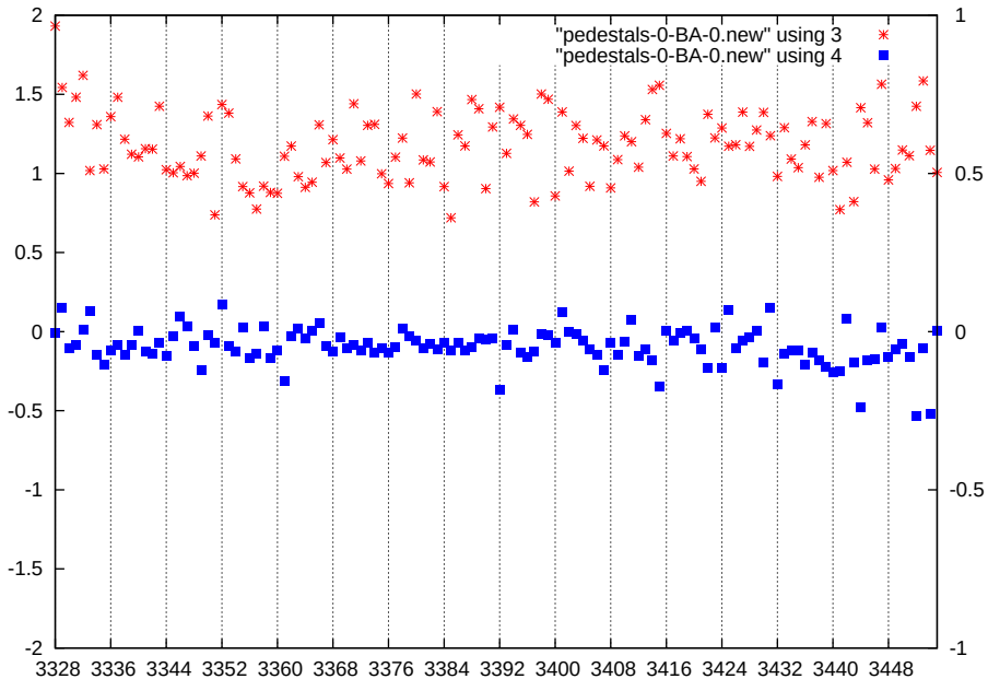
p1-gain1-shaper7-dac0
