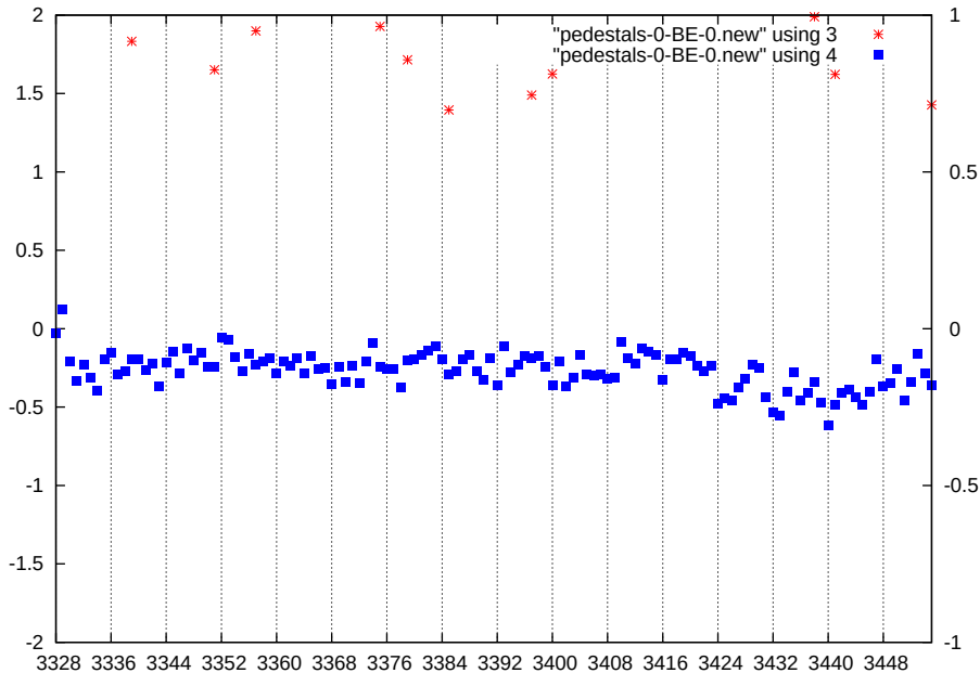
p1-gain3-shaper7-dac0
