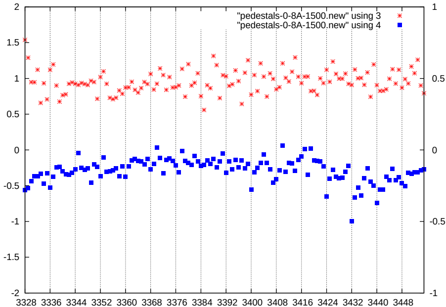
p1-gain1-shaper1-dac1500
