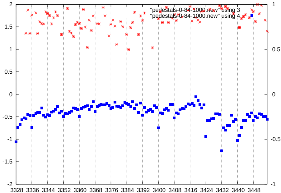
p1-gain2-shaper0-dac1000
