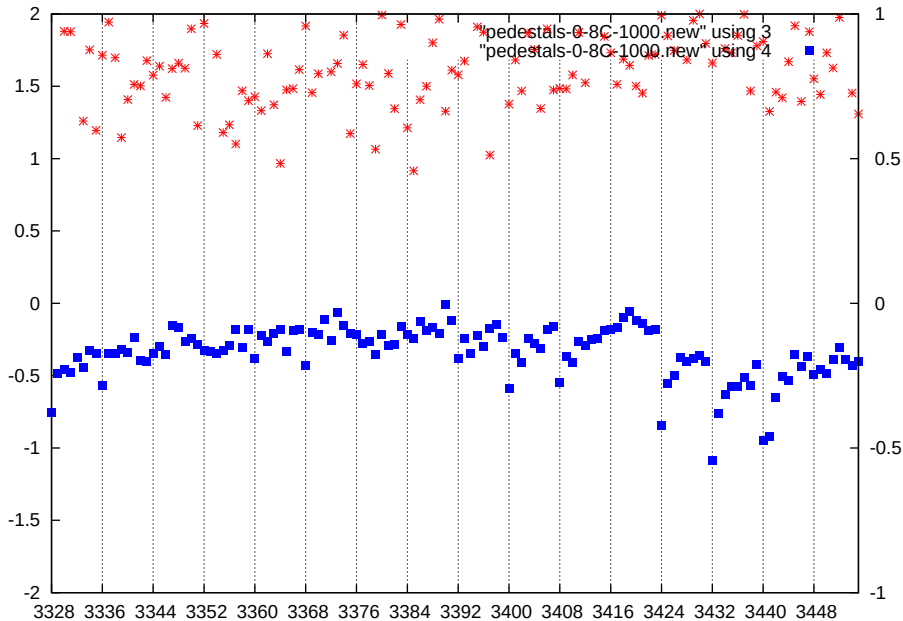
p1-gain2-shaper1-dac1000
