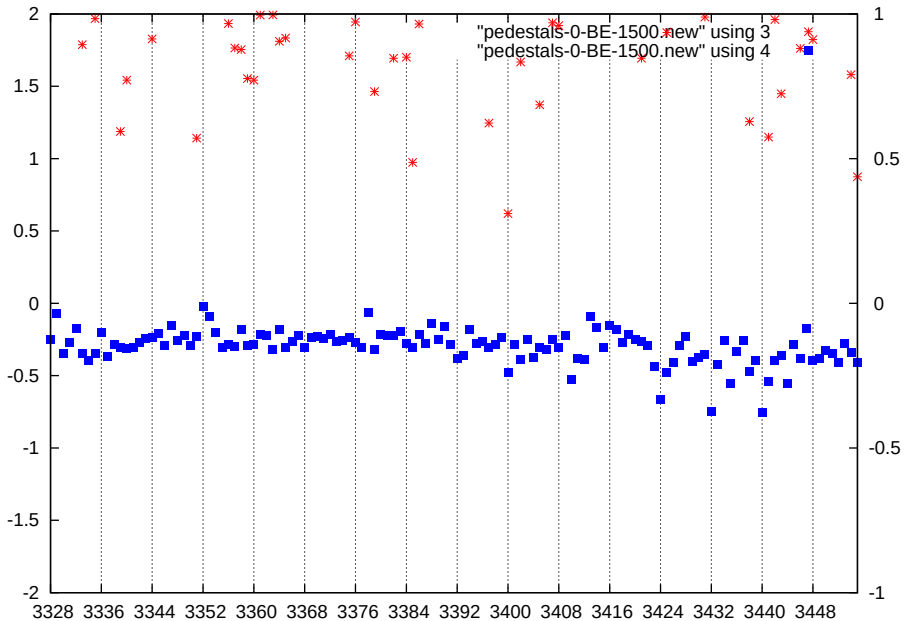
p1-gain3-shaper7-dac1500
