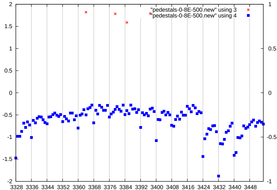
p1-gain3-shaper1-dac500
