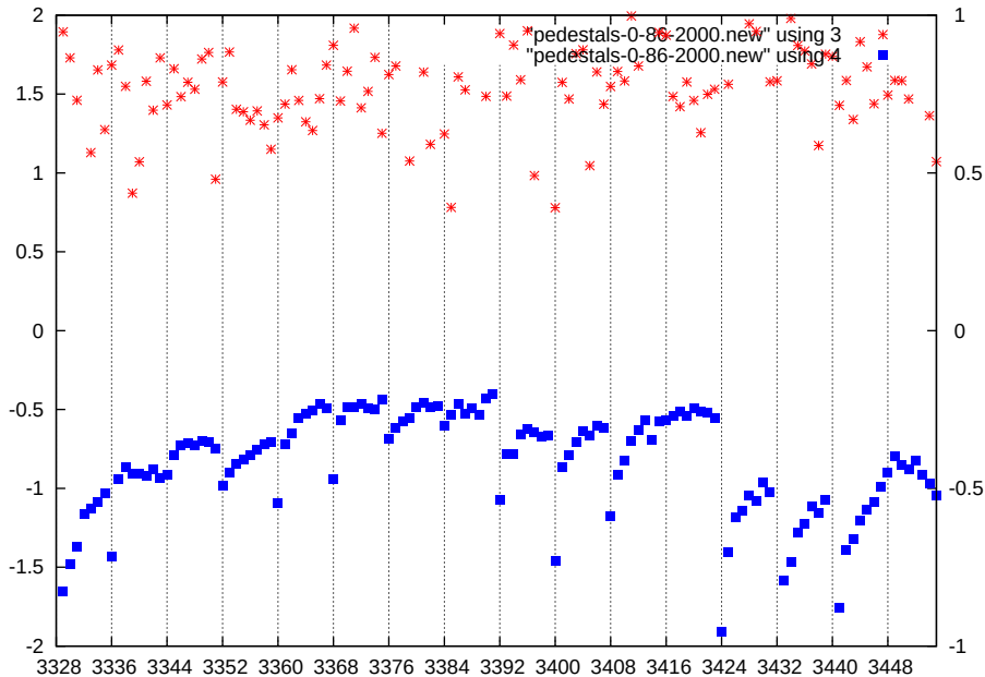
p1-gain3-shaper0-dac2000
