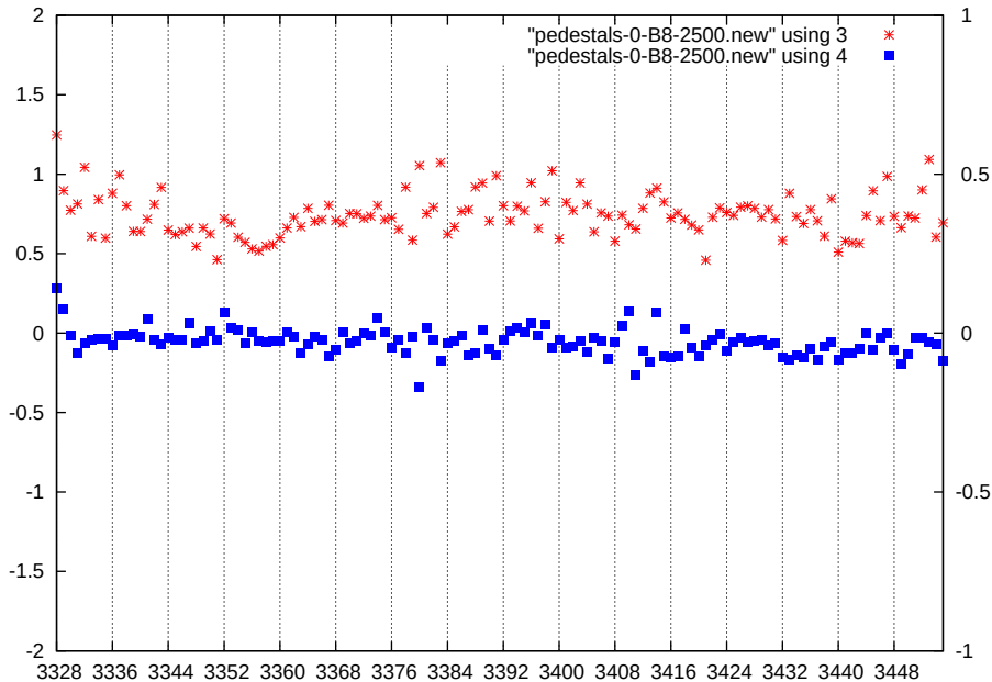
p1-gain0-shaper7-dac2500
