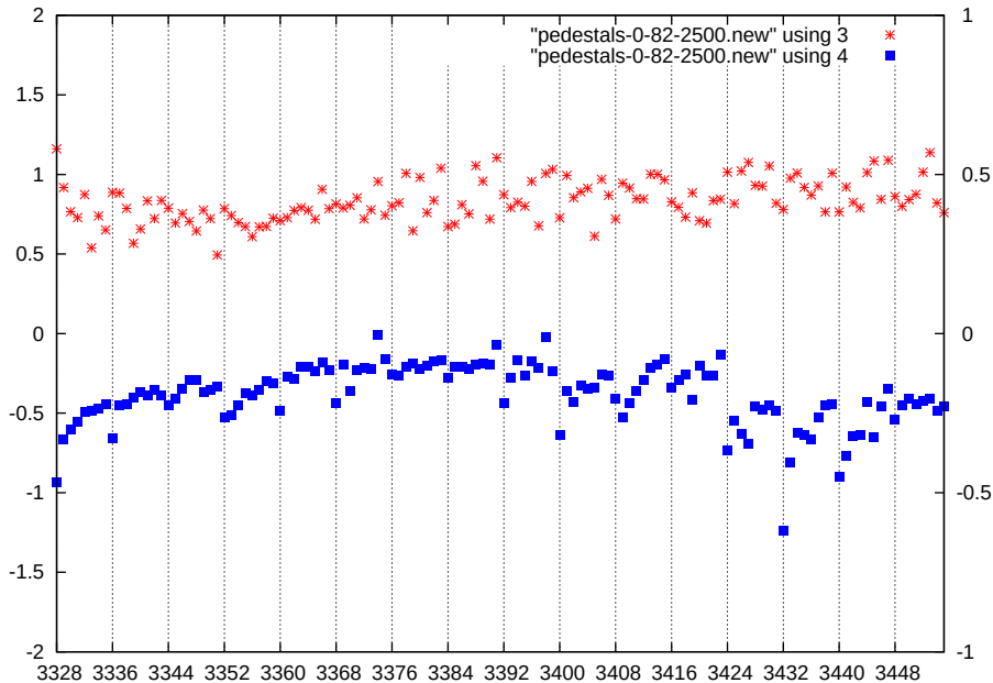
p1-gain1-shaper0-dac2500
