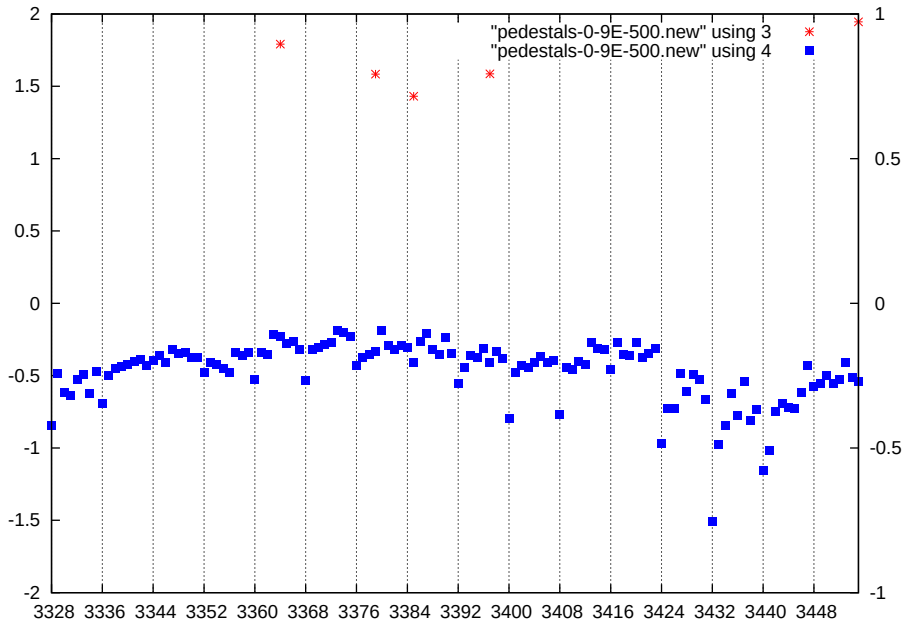
p1-gain3-shaper3-dac500
