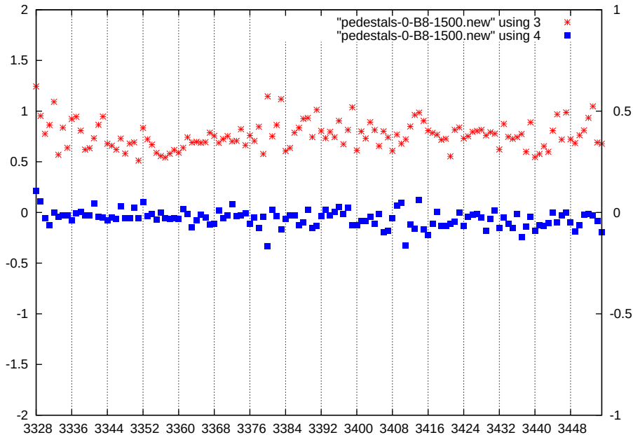
p1-gain0-shaper7-dac1500
