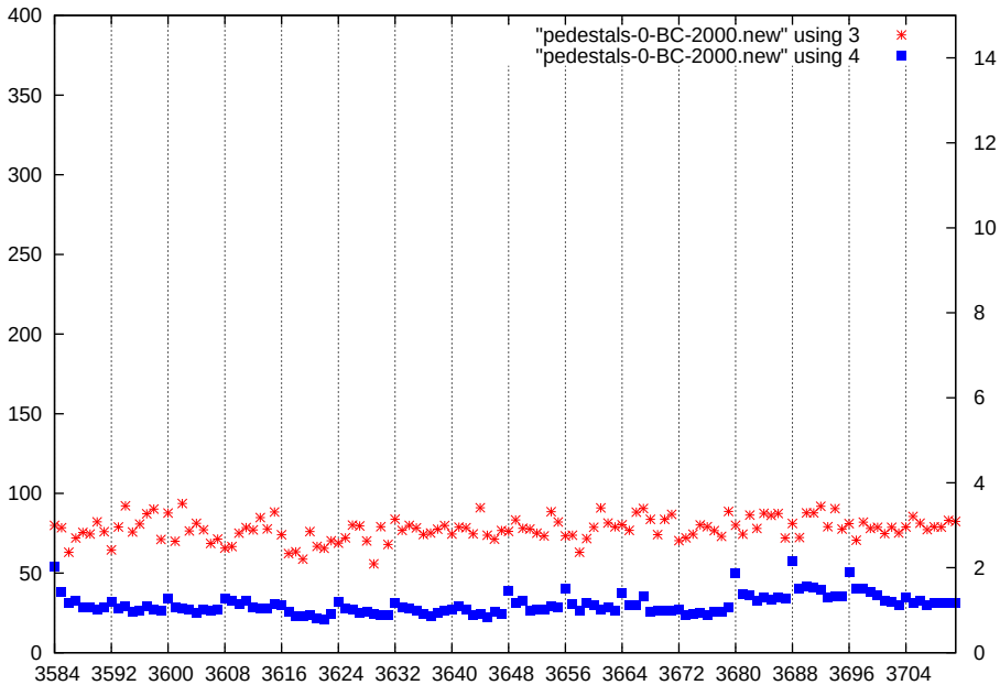
p1-gain2-shaper7-dac2000
