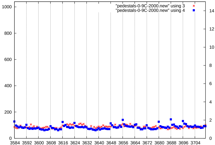
p1-gain2-shaper3-dac2000
