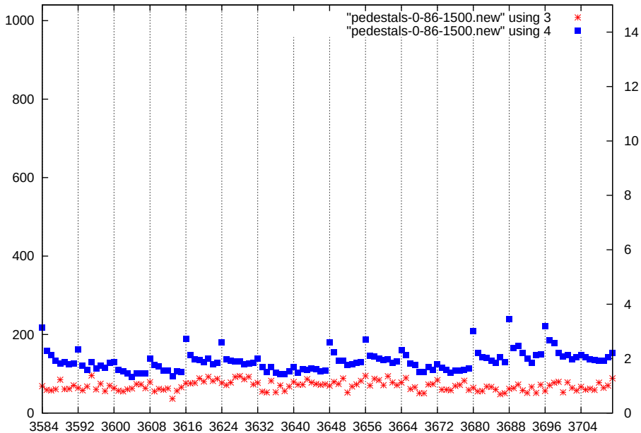
p1-gain3-shaper0-dac1500
