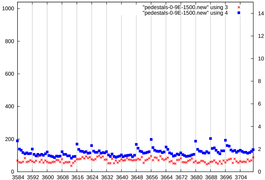
p1-gain3-shaper3-dac1500
