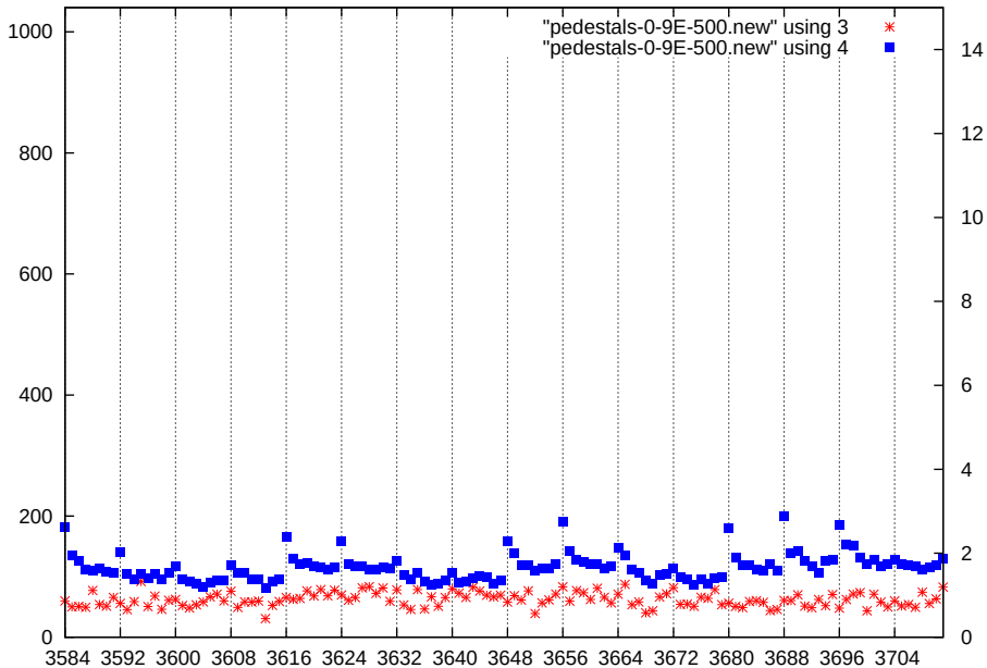
p1-gain3-shaper3-dac500
