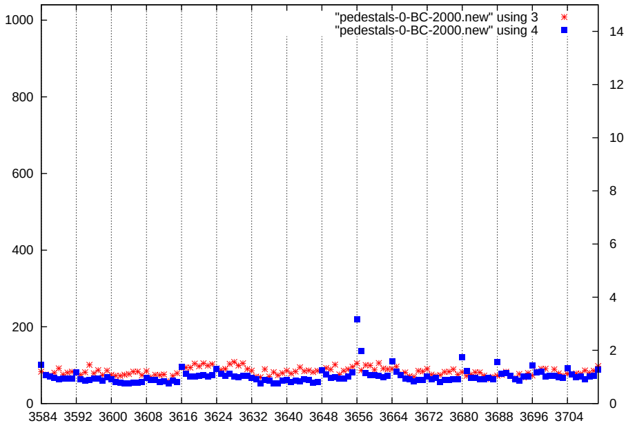
p1-gain2-shaper7-dac2000
