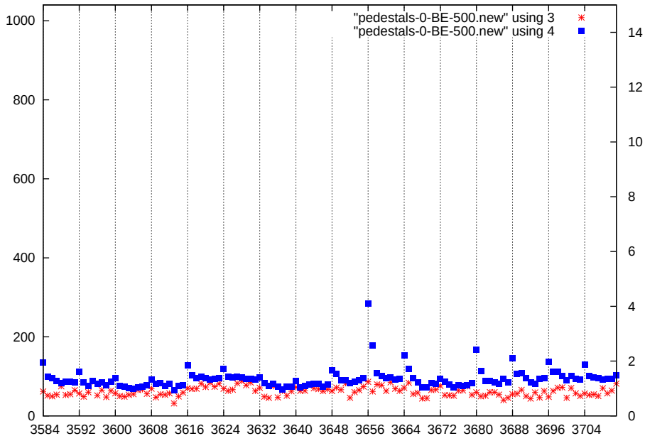
p1-gain3-shaper7-dac500
