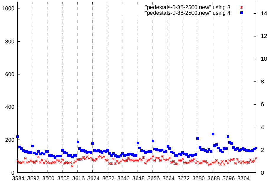
p1-gain3-shaper0-dac2500
