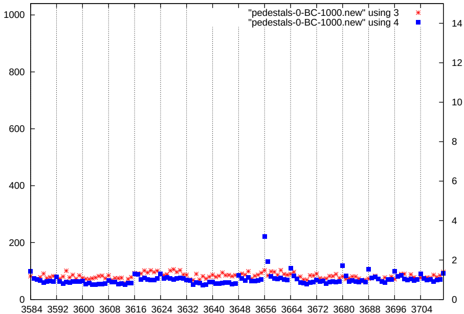
p1-gain2-shaper7-dac1000
