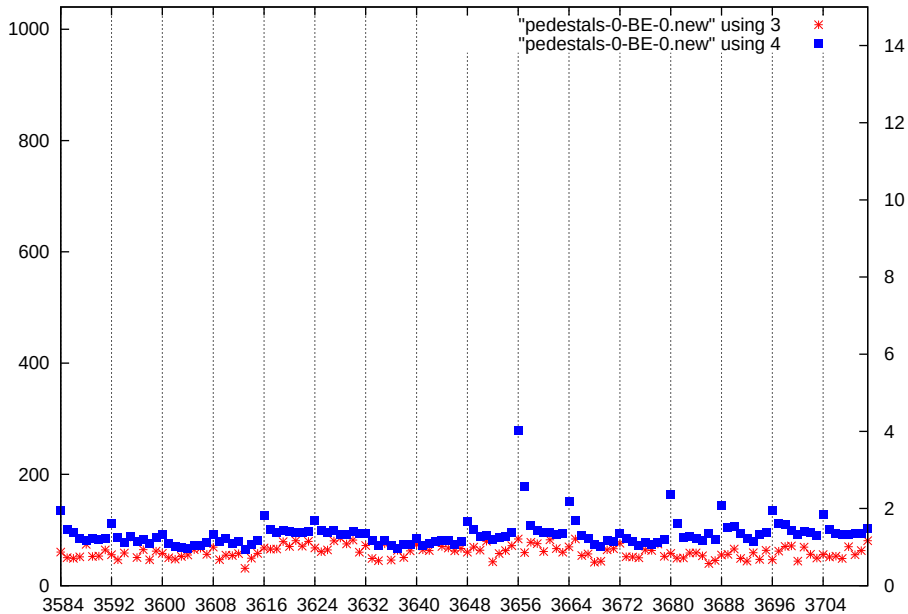
p1-gain3-shaper7-dac0
