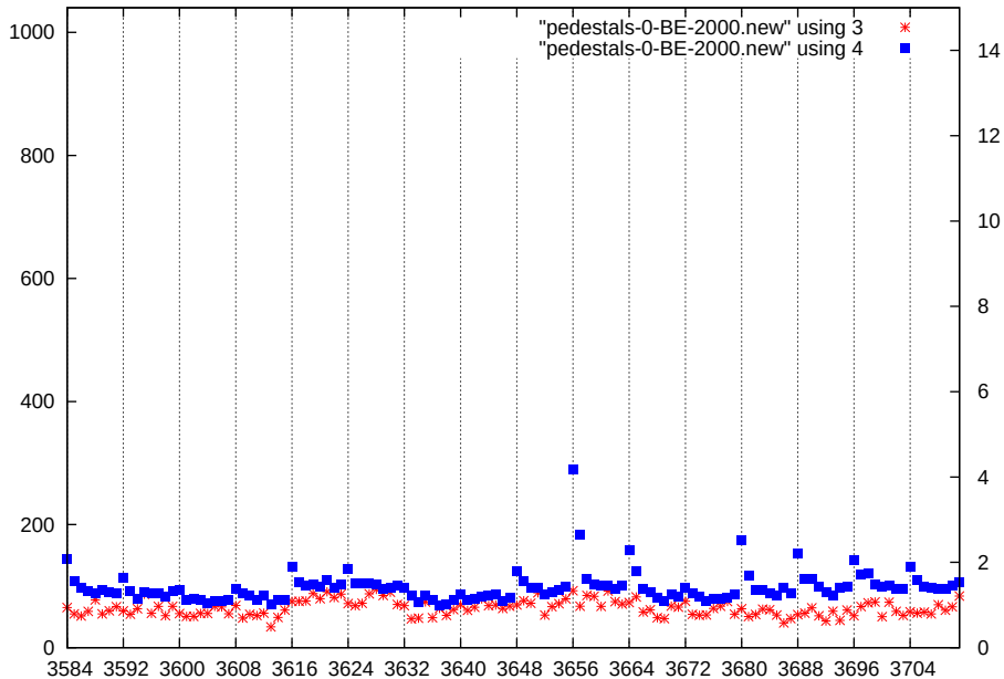
p1-gain3-shaper7-dac2000
