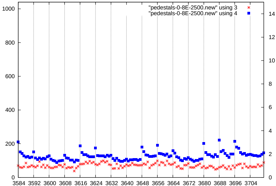
p1-gain3-shaper1-dac2500
