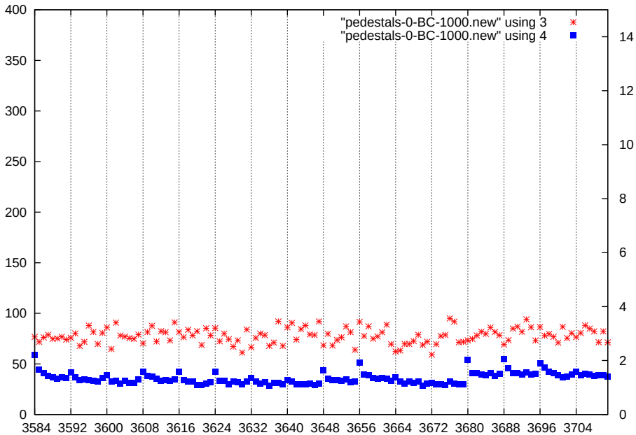
p1-gain2-shaper7-dac1000
