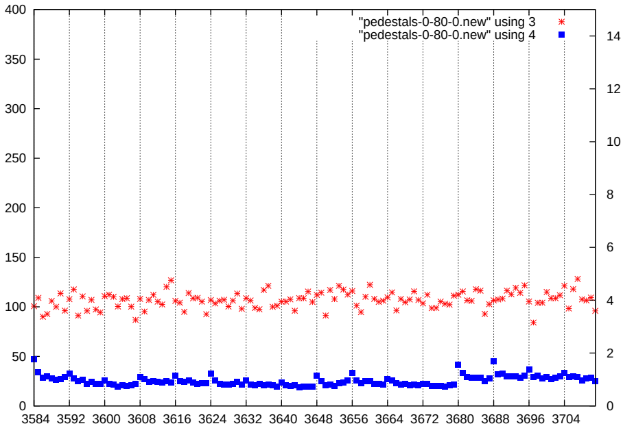
p1-gain0-shaper0-dac0
