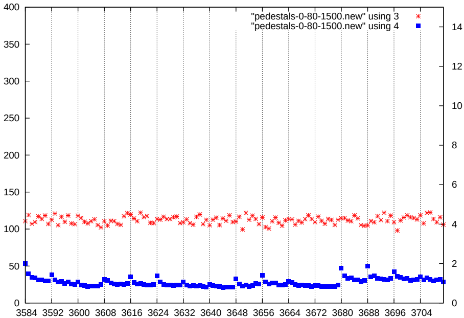
p1-gain0-shaper0-dac1500
