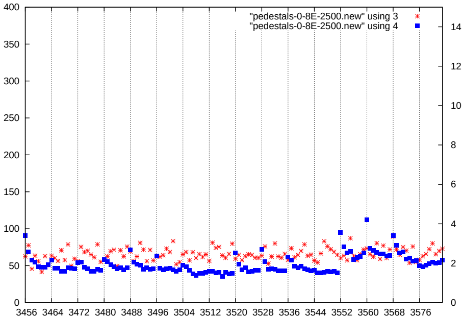
p1-gain3-shaper1-dac2500
