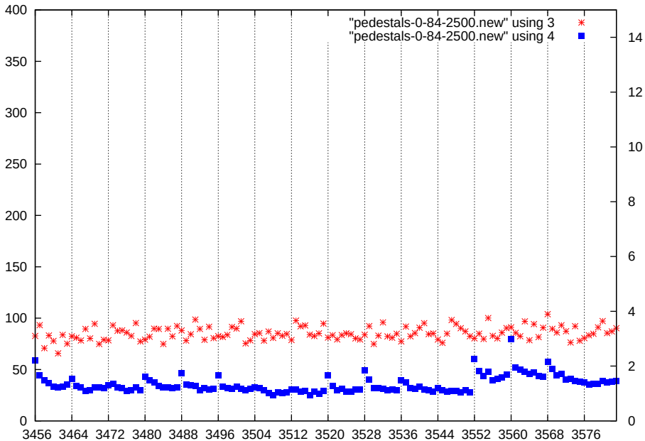
p1-gain2-shaper0-dac2500
