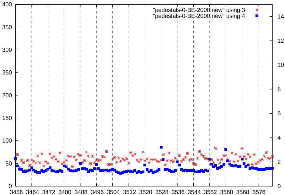
p1-gain3-shaper7-dac2000
