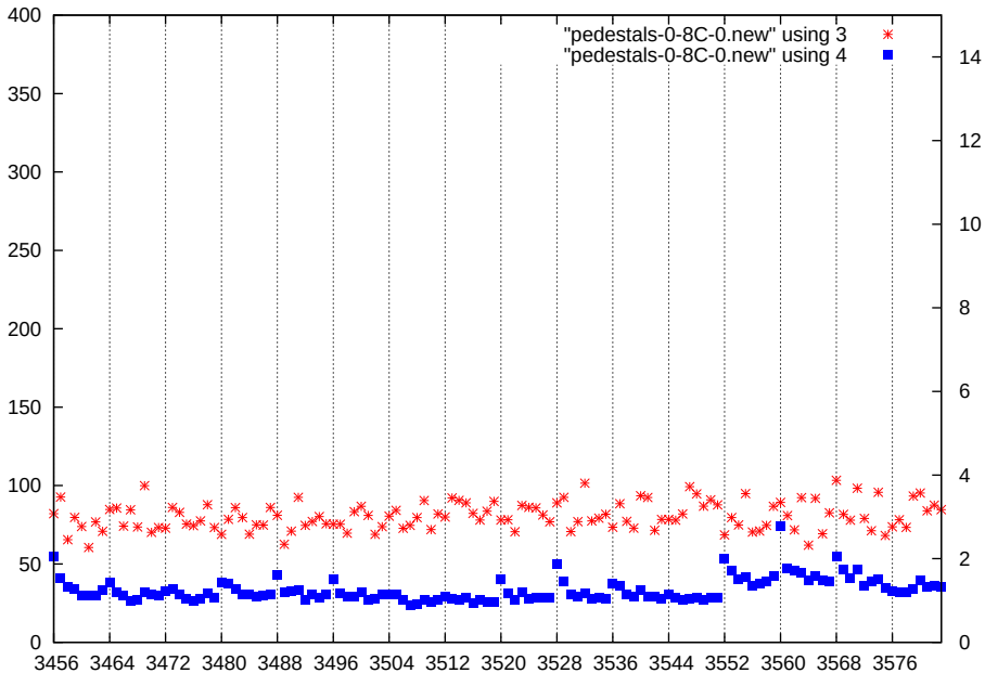
p1-gain2-shaper1-dac0
