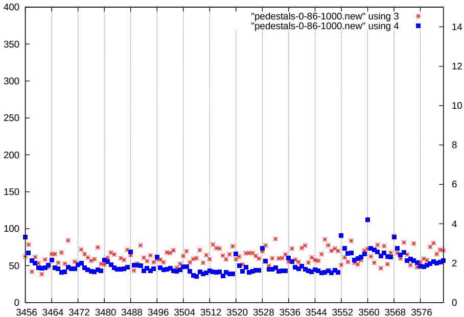
p1-gain3-shaper0-dac1000
