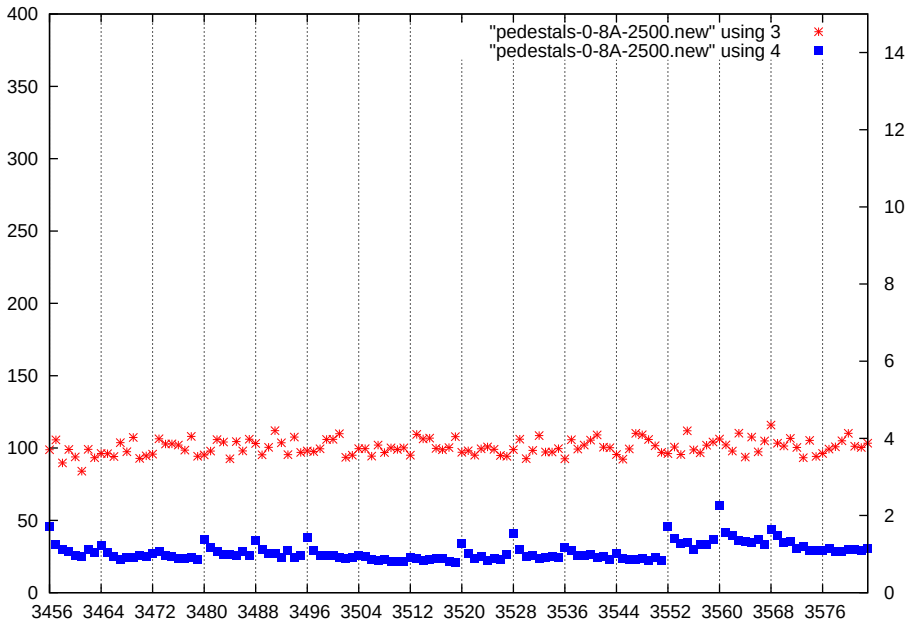
p1-gain1-shaper1-dac2500
