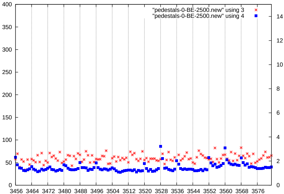
p1-gain3-shaper7-dac2500
