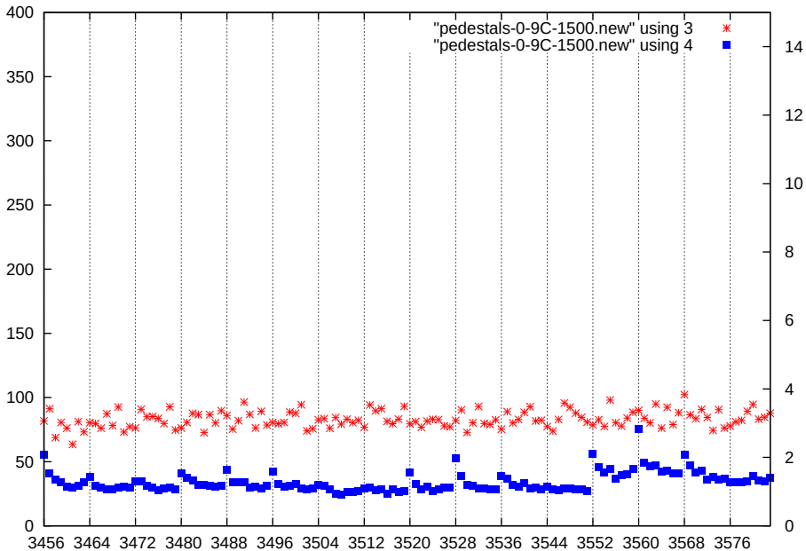
p1-gain2-shaper3-dac1500
