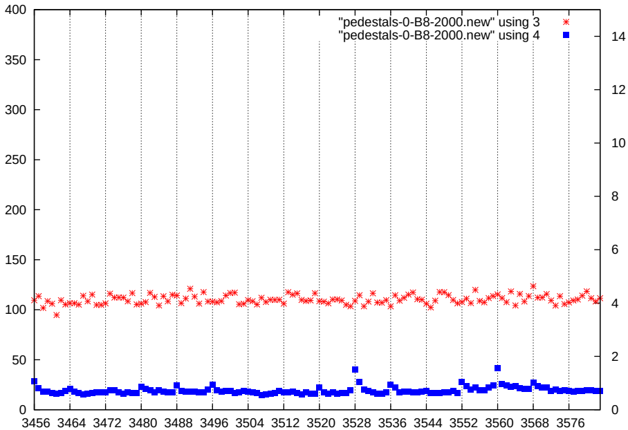
p1-gain0-shaper7-dac2000
