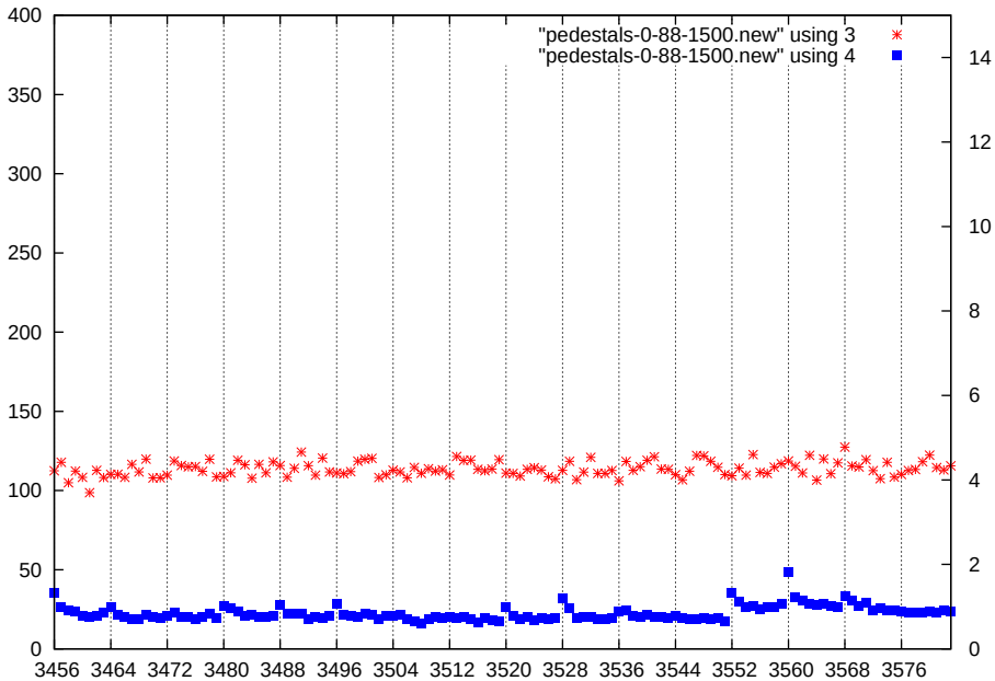
p1-gain0-shaper1-dac1500
