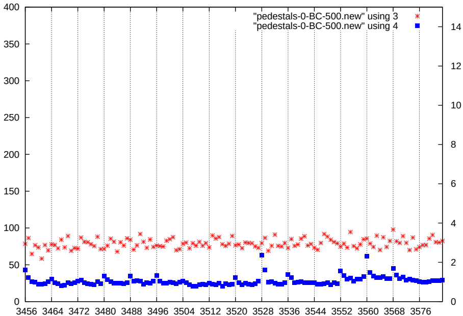
p1-gain2-shaper7-dac500
