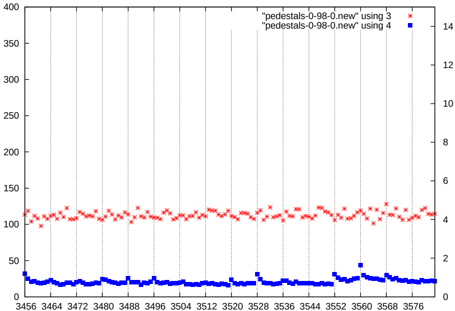
p1-gain0-shaper3-dac0
