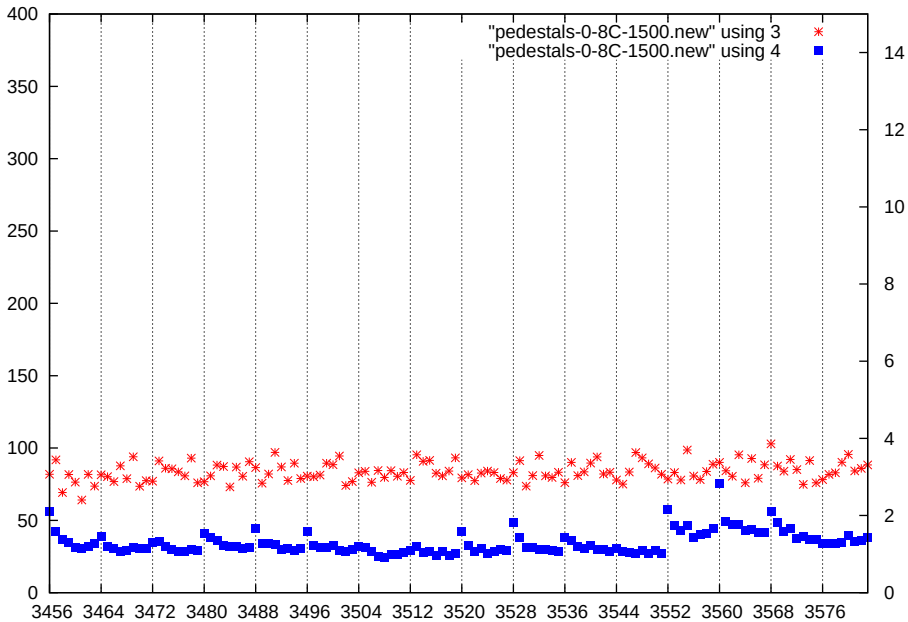
p1-gain2-shaper1-dac1500
