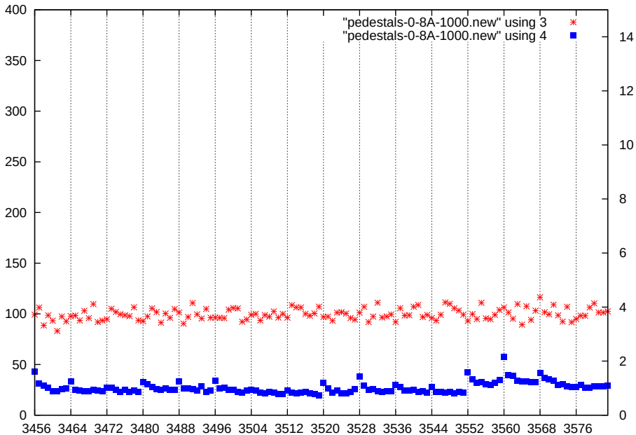
p1-gain1-shaper1-dac1000
