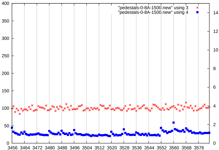
p1-gain1-shaper1-dac1500
