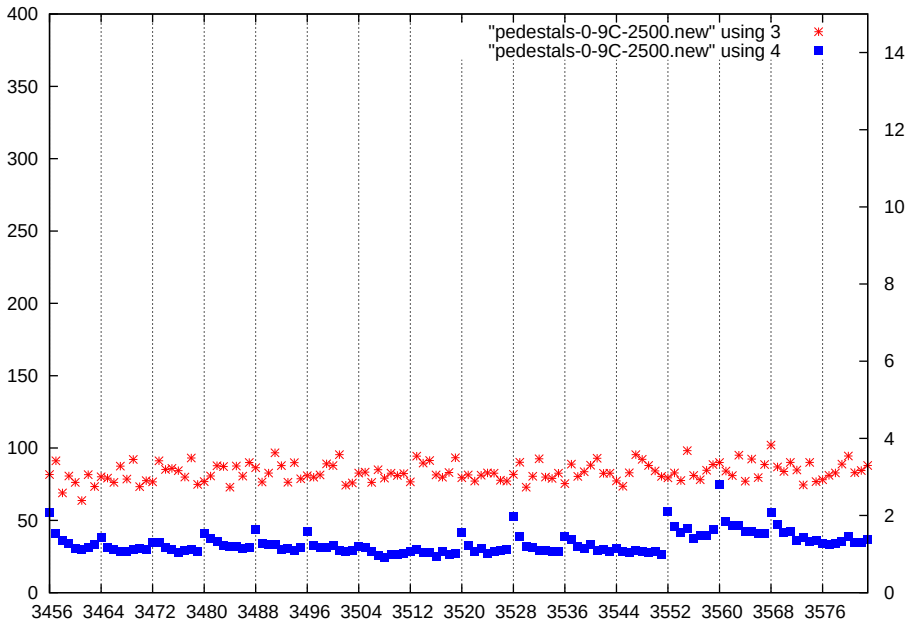
p1-gain2-shaper3-dac2500
