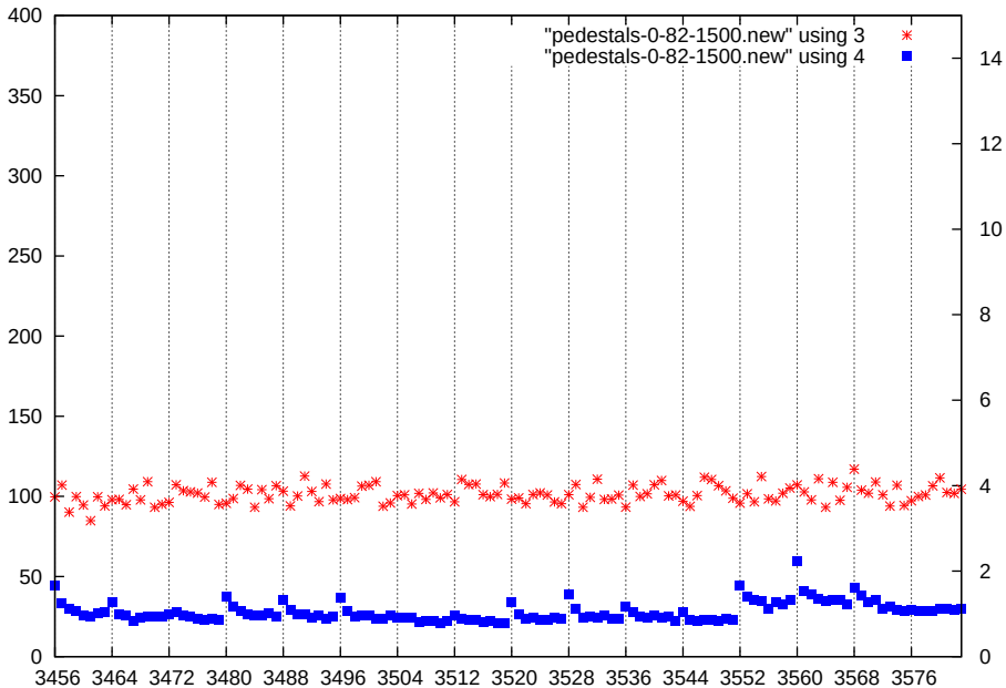
p1-gain1-shaper0-dac1500
