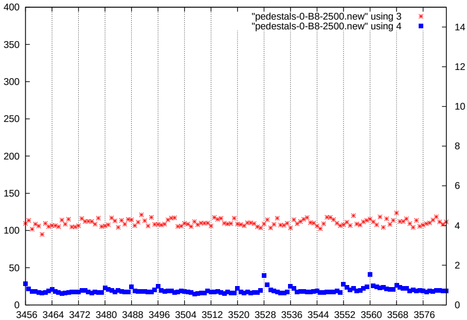
p1-gain0-shaper7-dac2500
