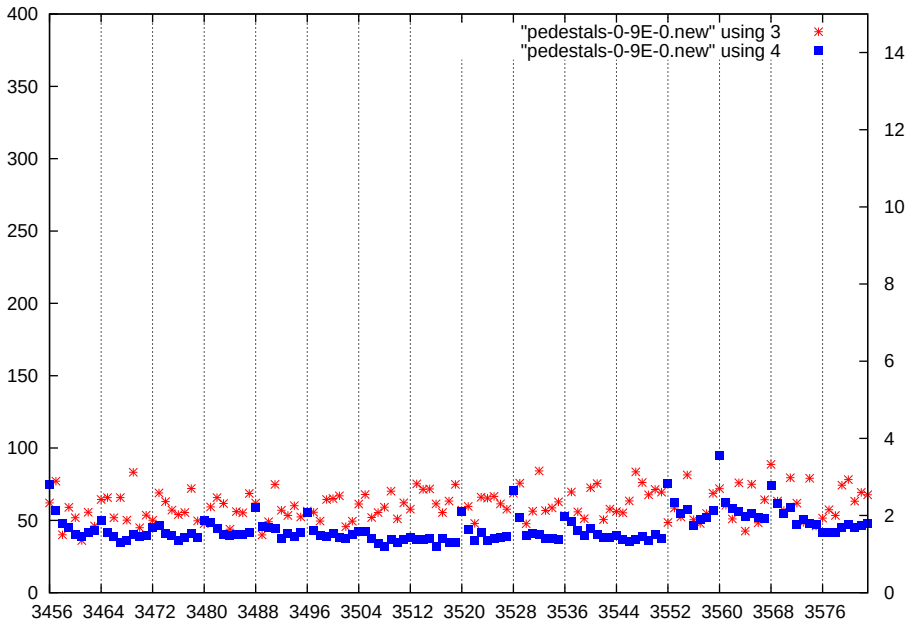
p1-gain3-shaper3-dac0
