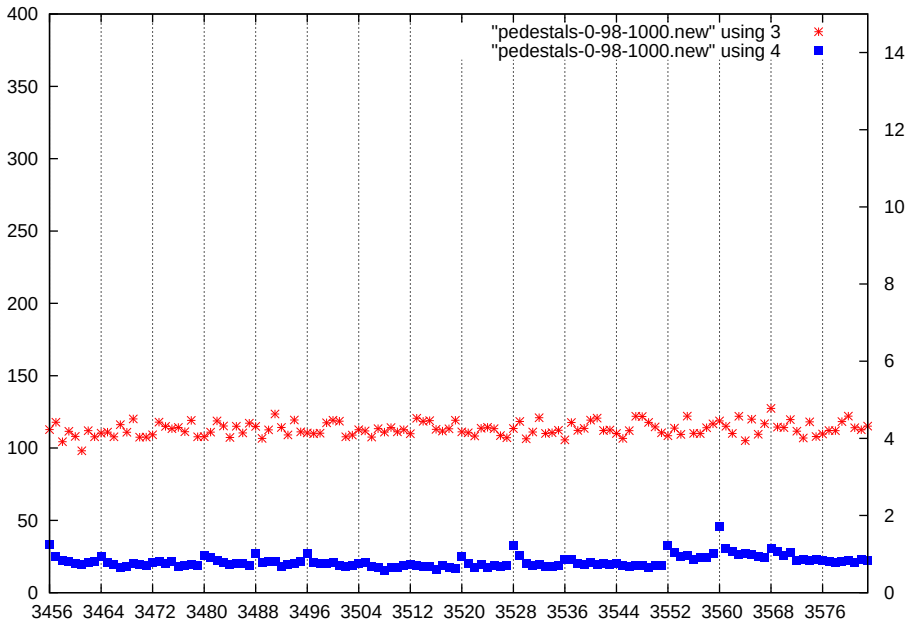
p1-gain0-shaper3-dac1000
