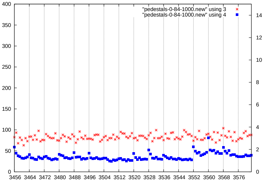
p1-gain2-shaper0-dac1000
