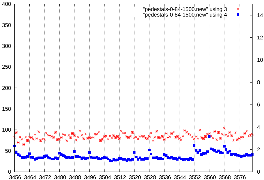
p1-gain2-shaper0-dac1500
