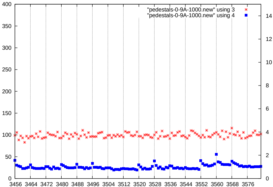
p1-gain1-shaper3-dac1000
