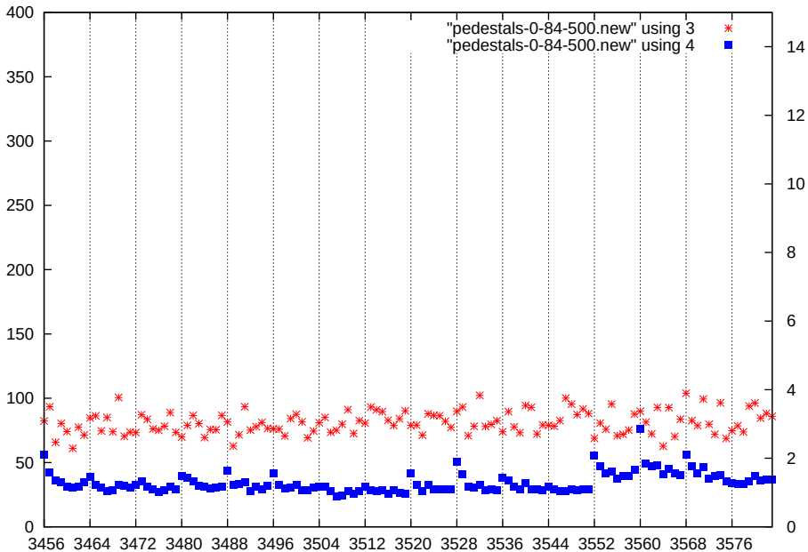
p1-gain2-shaper0-dac500
