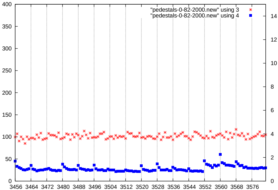
p1-gain1-shaper0-dac2000
