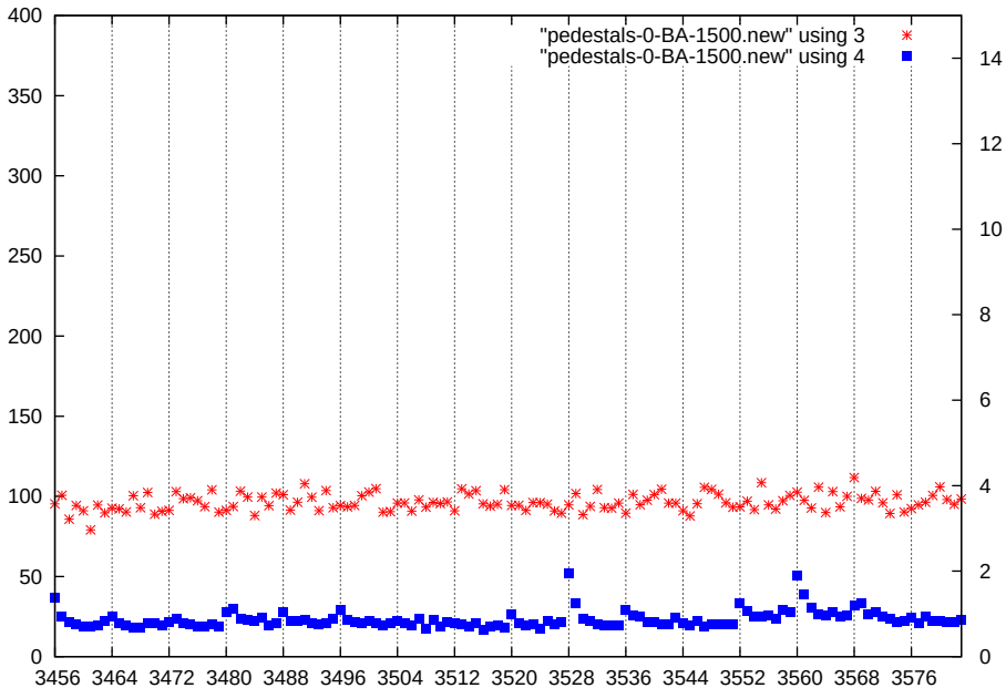
p1-gain1-shaper7-dac1500
