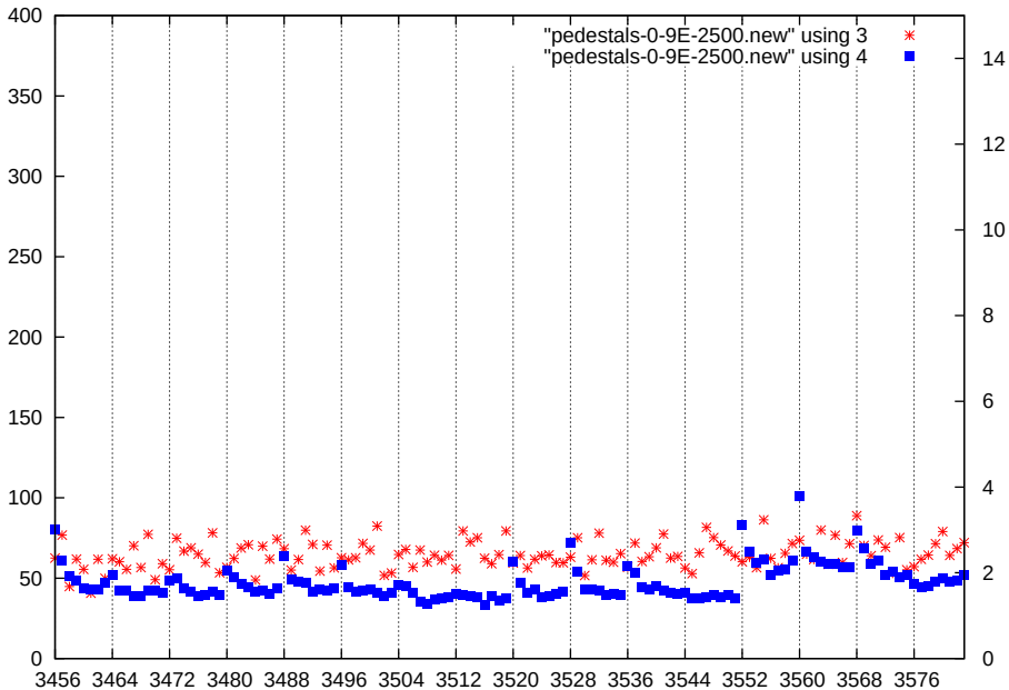
p1-gain3-shaper3-dac2500
