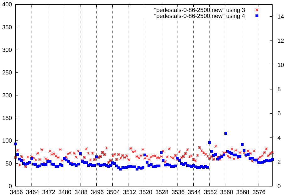
p1-gain3-shaper0-dac2500
