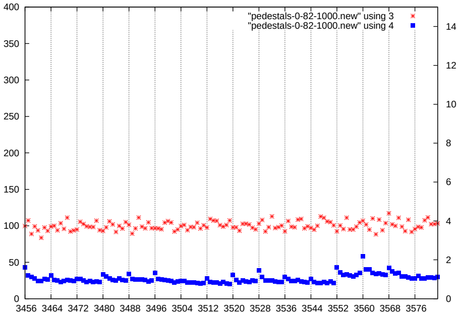
p1-gain1-shaper0-dac1000
