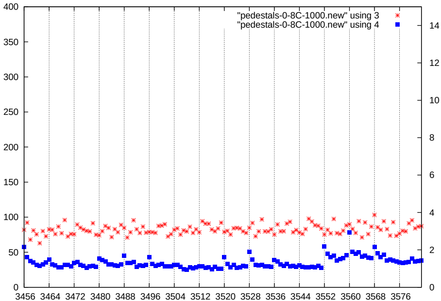
p1-gain2-shaper1-dac1000
