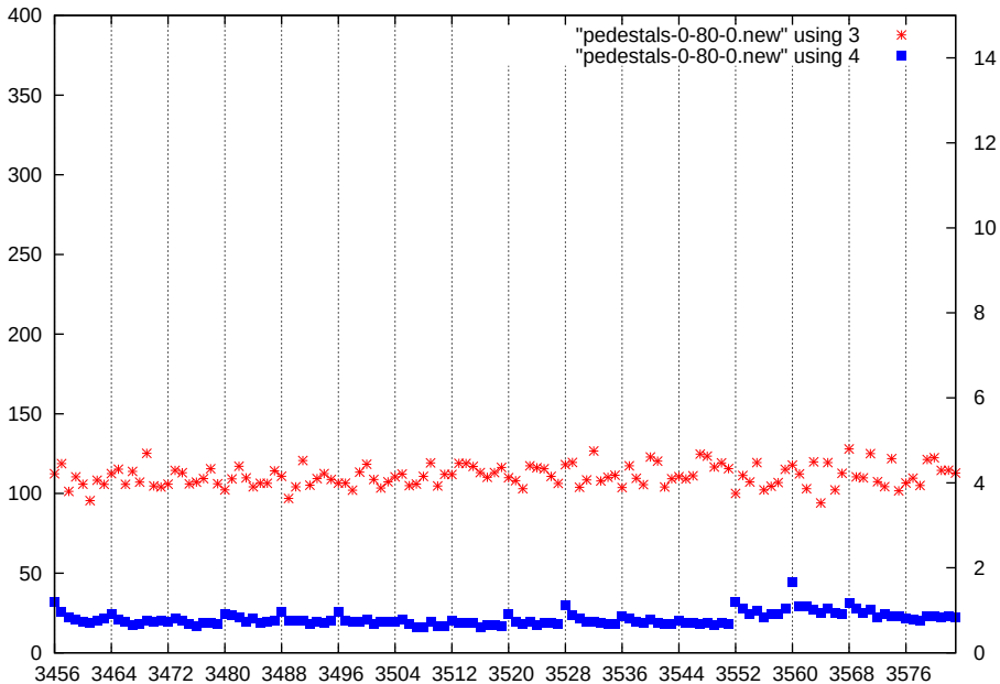
p1-gain0-shaper0-dac0
