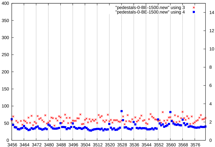
p1-gain3-shaper7-dac1500
