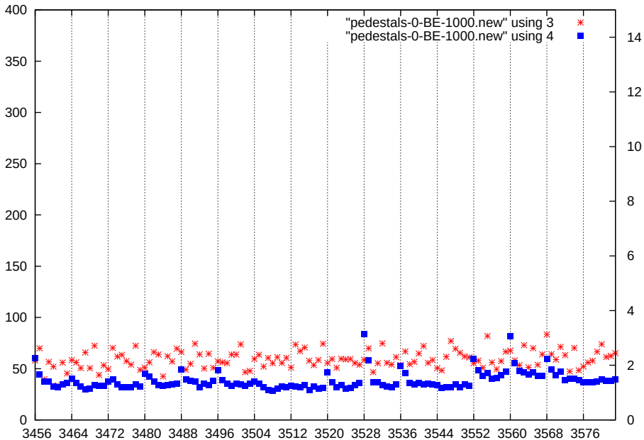
p1-gain3-shaper7-dac1000
