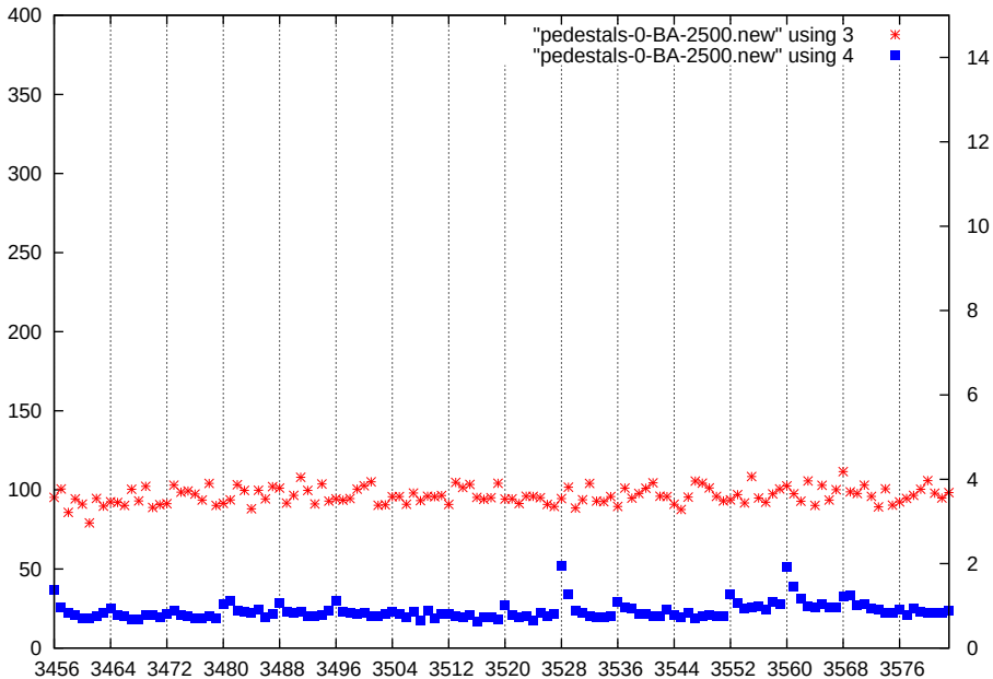
p1-gain1-shaper7-dac2500
