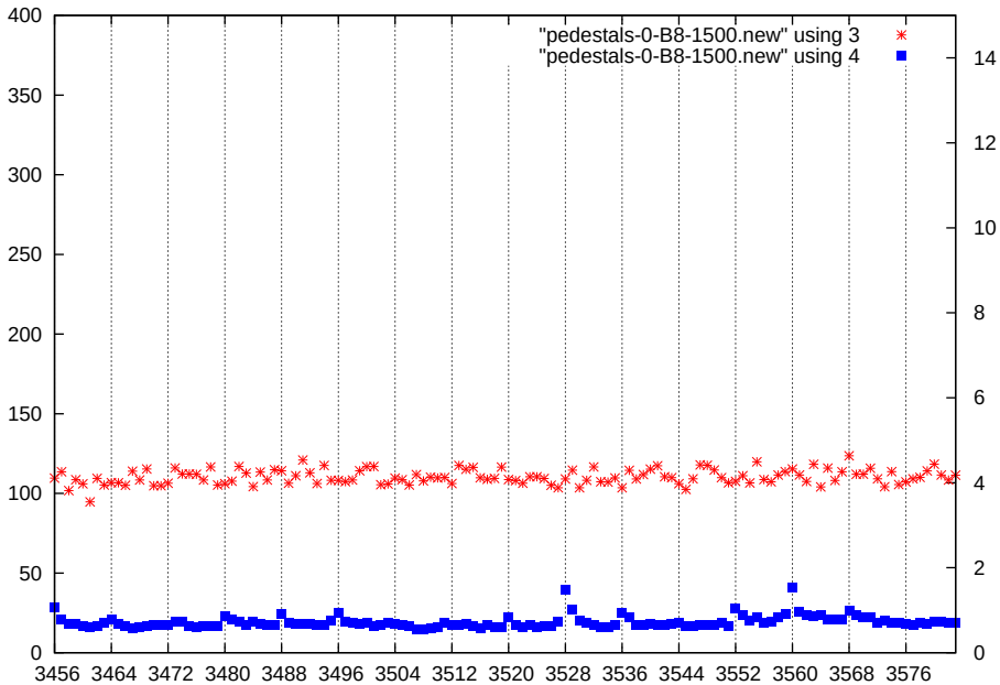
p1-gain0-shaper7-dac1500
