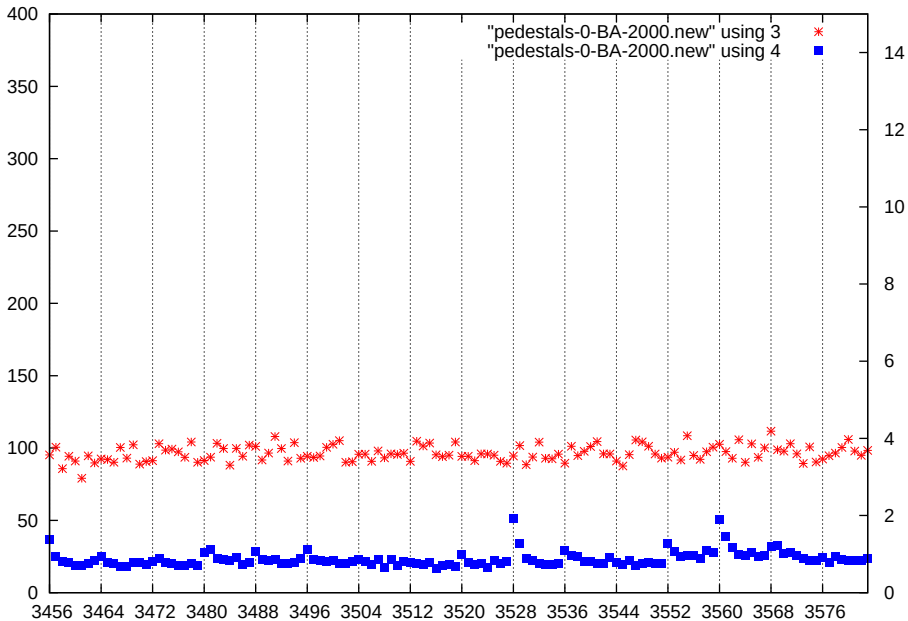
p1-gain1-shaper7-dac2000
