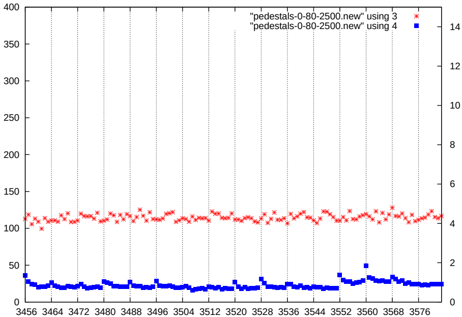
p1-gain0-shaper0-dac2500
