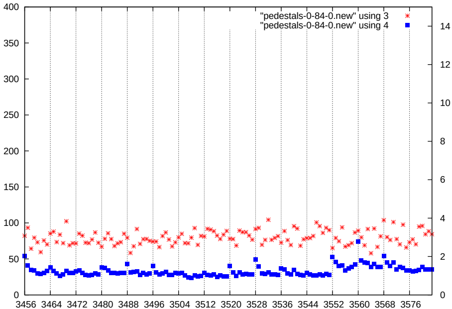
p1-gain2-shaper0-dac0
