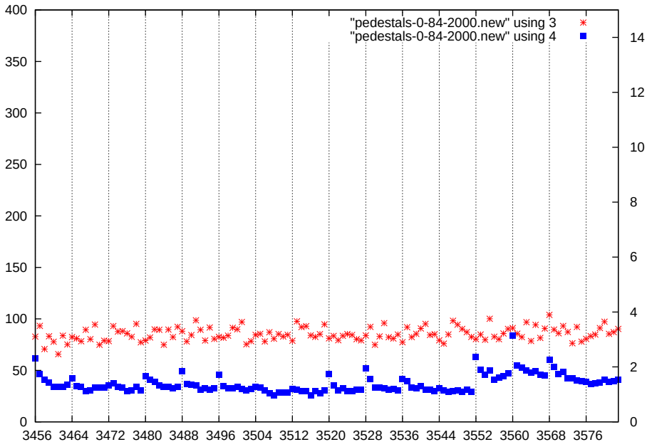
p1-gain2-shaper0-dac2000
