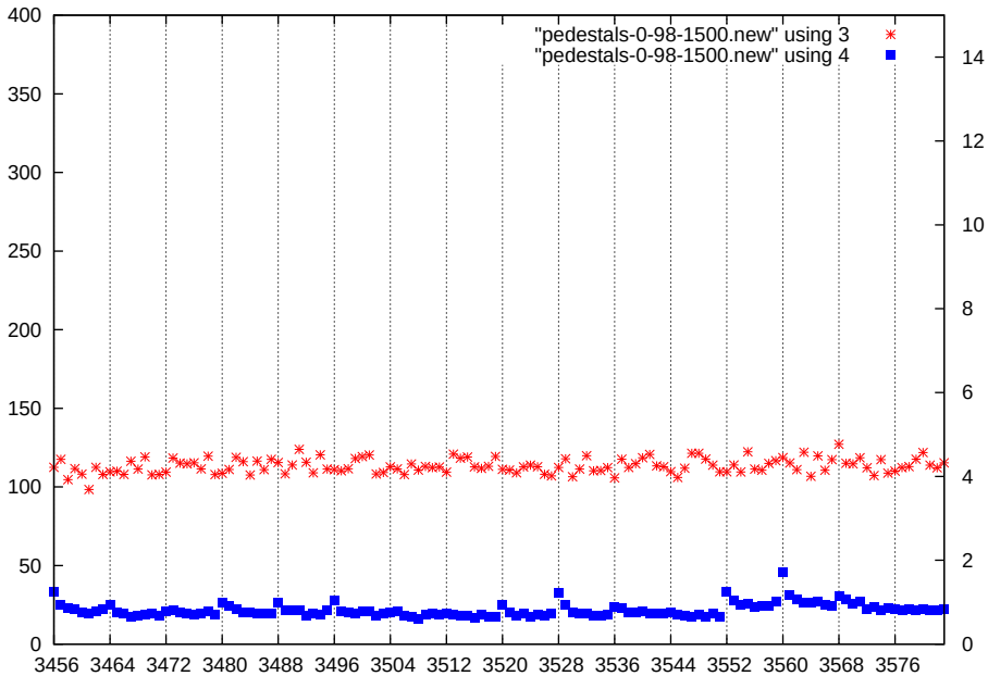
p1-gain0-shaper3-dac1500
