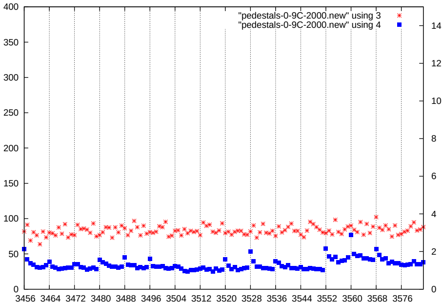
p1-gain2-shaper3-dac2000
