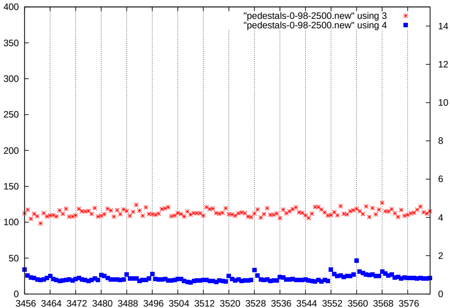
p1-gain0-shaper3-dac2500
