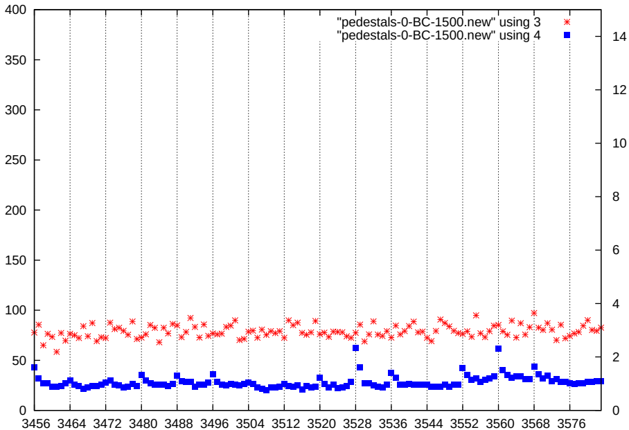
p1-gain2-shaper7-dac1500
