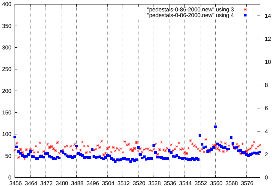
p1-gain3-shaper0-dac2000
