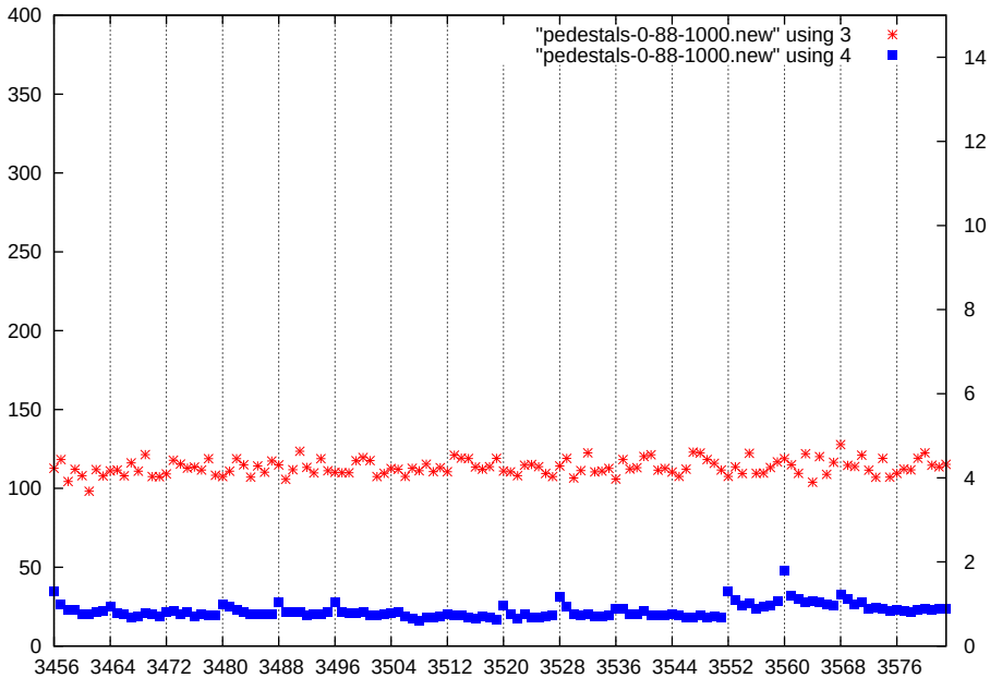
p1-gain0-shaper1-dac1000
