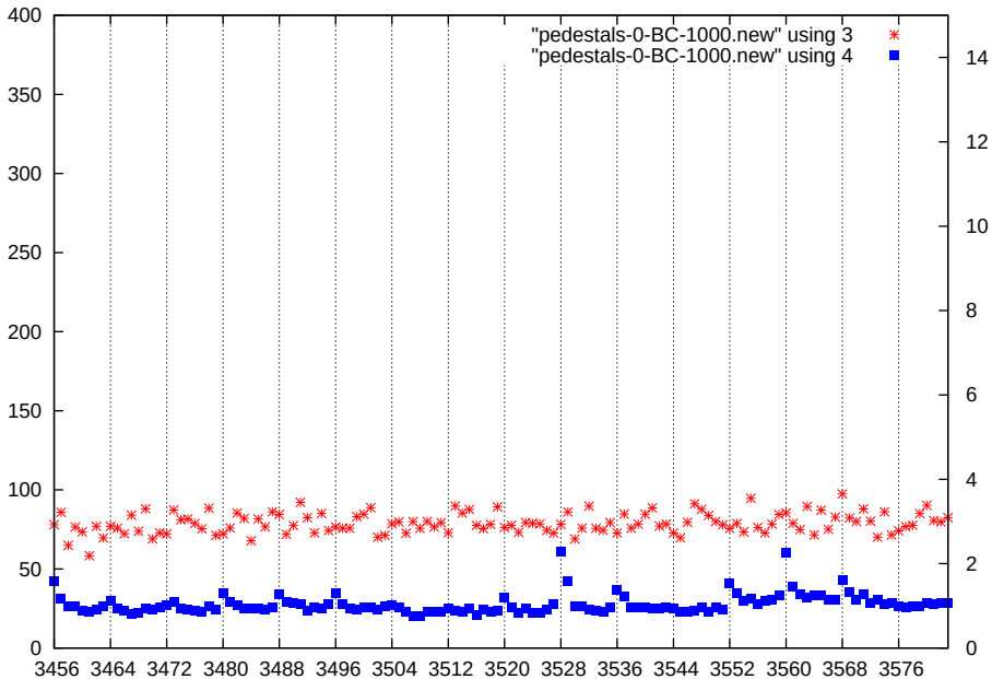
p1-gain2-shaper7-dac1000
