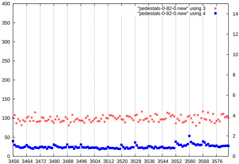
p1-gain1-shaper0-dac0
