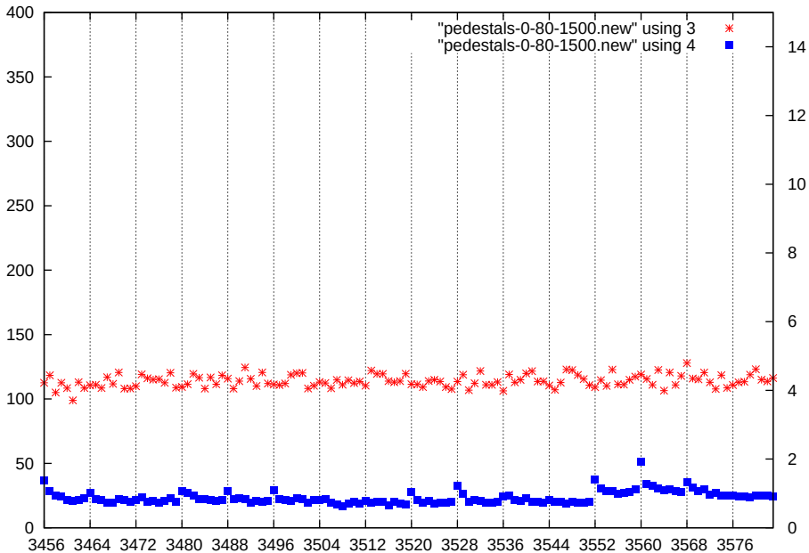
p1-gain0-shaper0-dac1500
