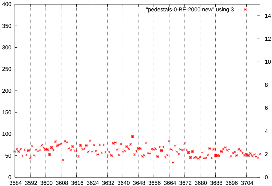
p1-gain3-shaper7-dac2000
