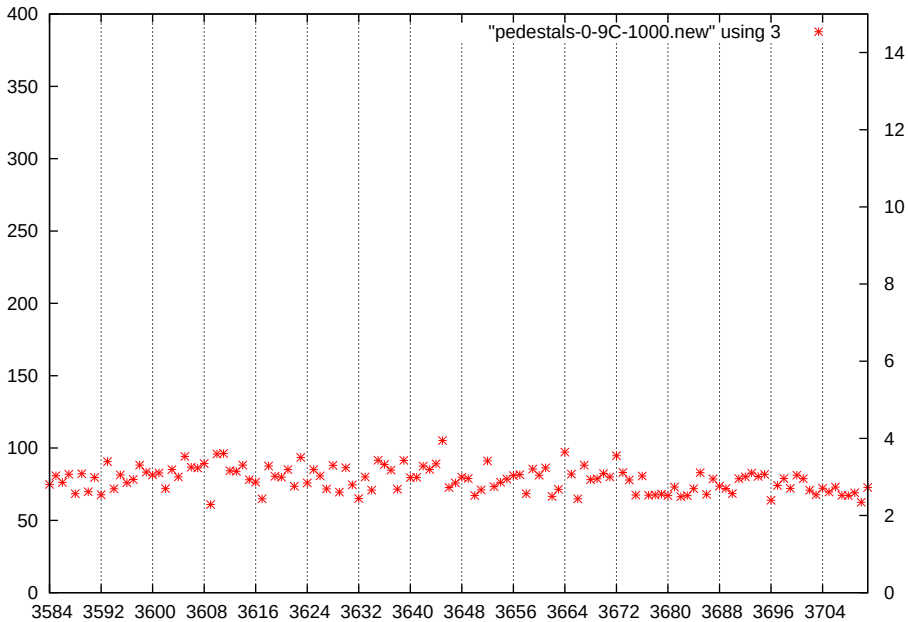
p1-gain2-shaper3-dac1000
