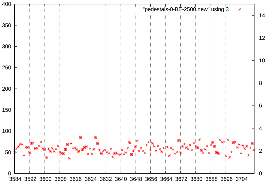
p1-gain3-shaper7-dac2500
