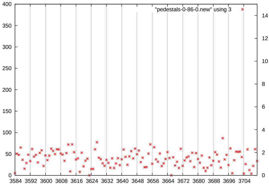
p1-gain3-shaper0-dac0
