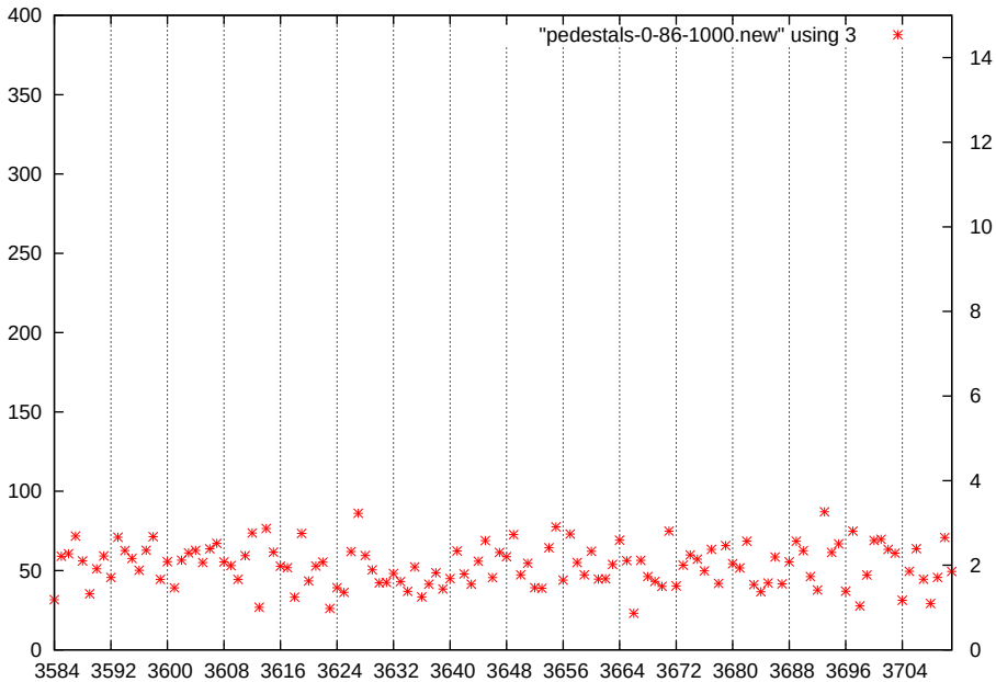
p1-gain3-shaper0-dac1000
