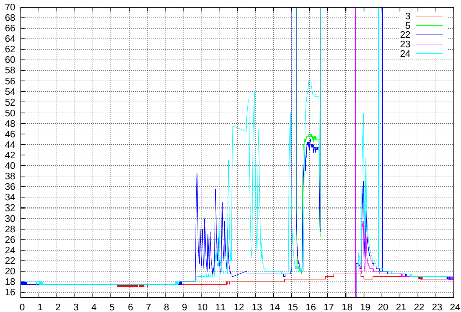
Temperatures Testbeam 20100325
