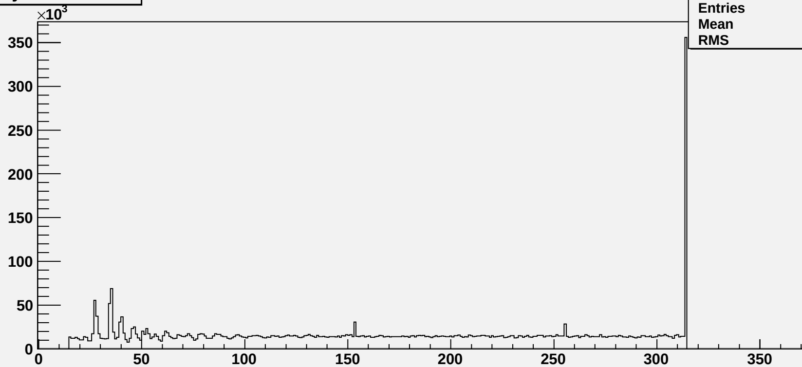
Empty clusters
