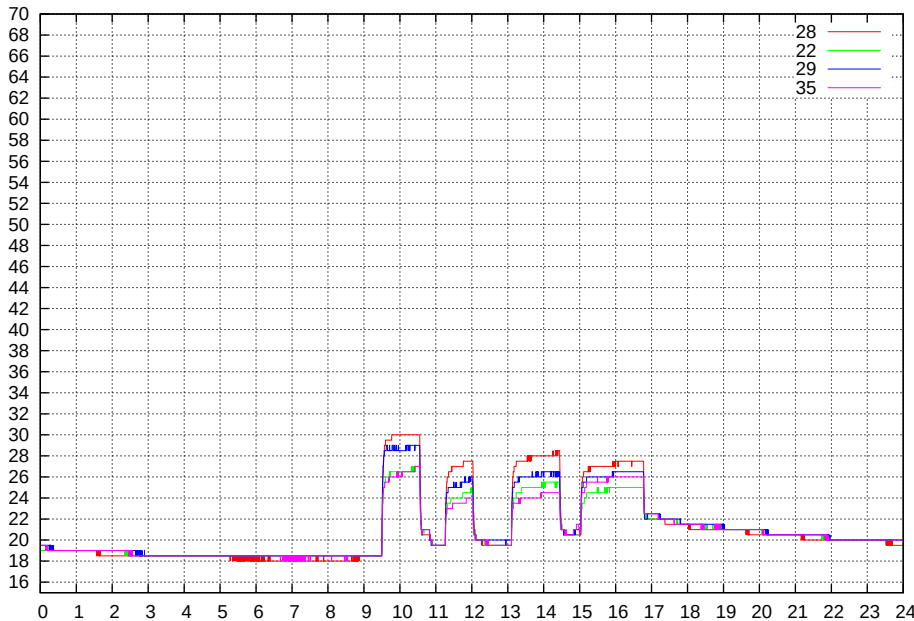
Temperatures Testbeam 20100922
