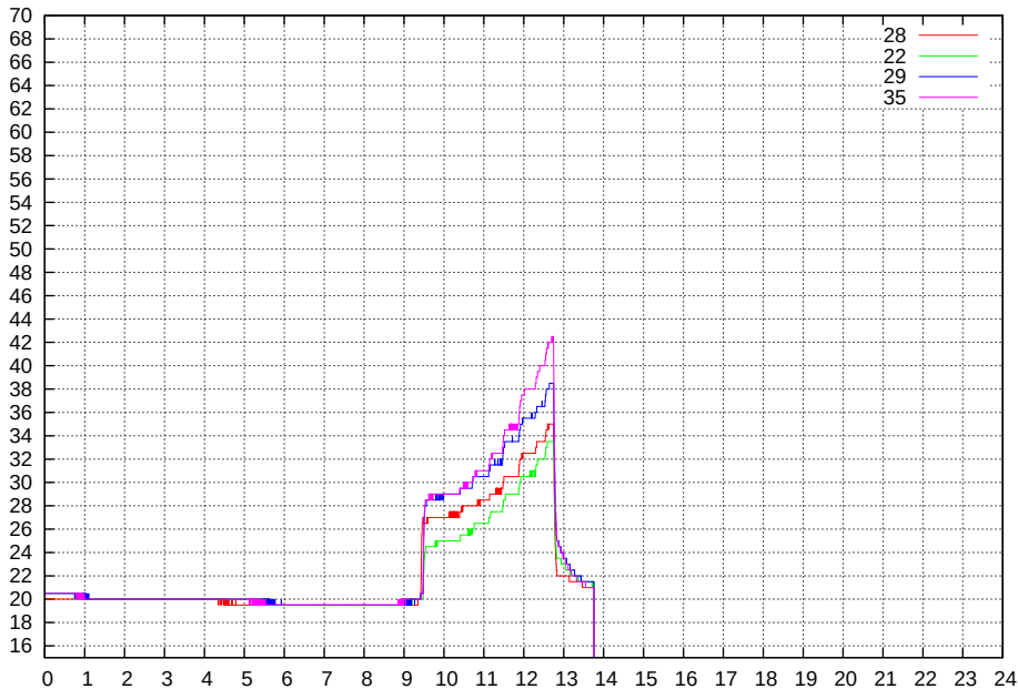
Temperatures Testbeam 20100924
