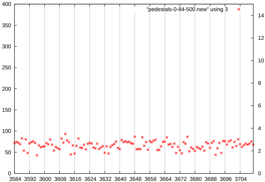
p1-gain2-shaper0-dac500
