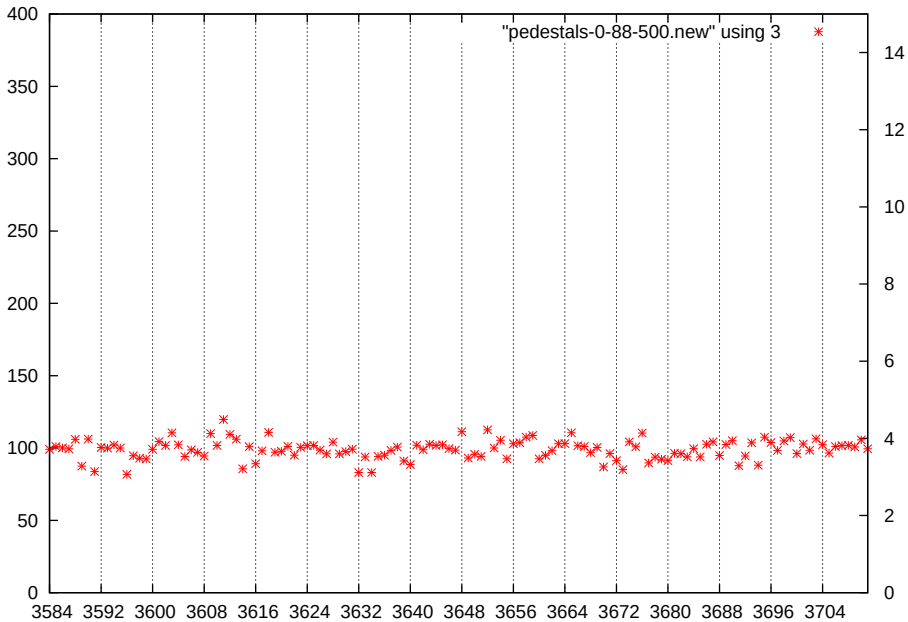
p1-gain0-shaper1-dac500
