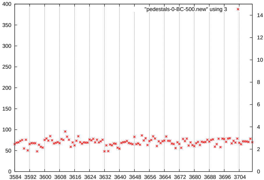
p1-gain2-shaper7-dac500
