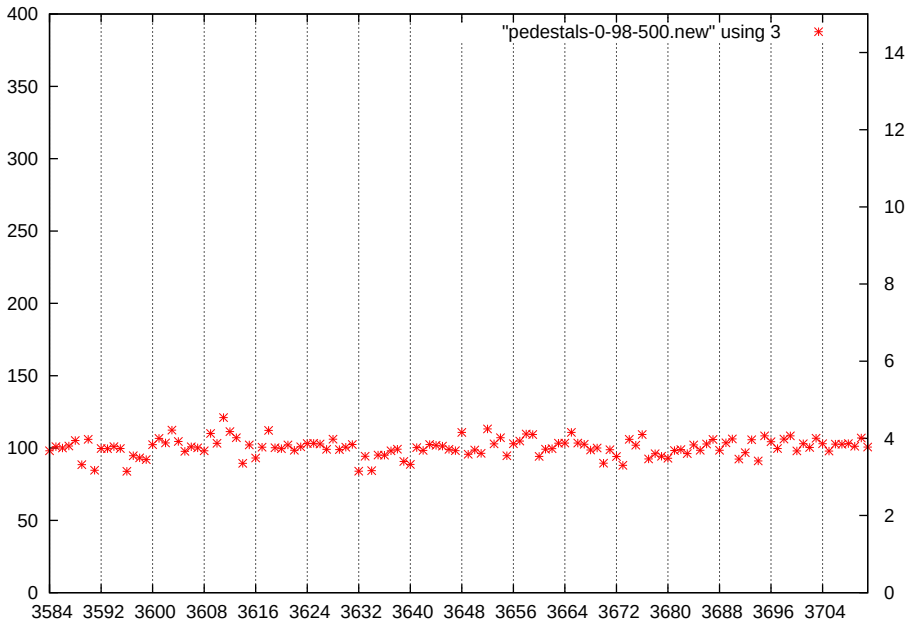
p1-gain0-shaper3-dac500
