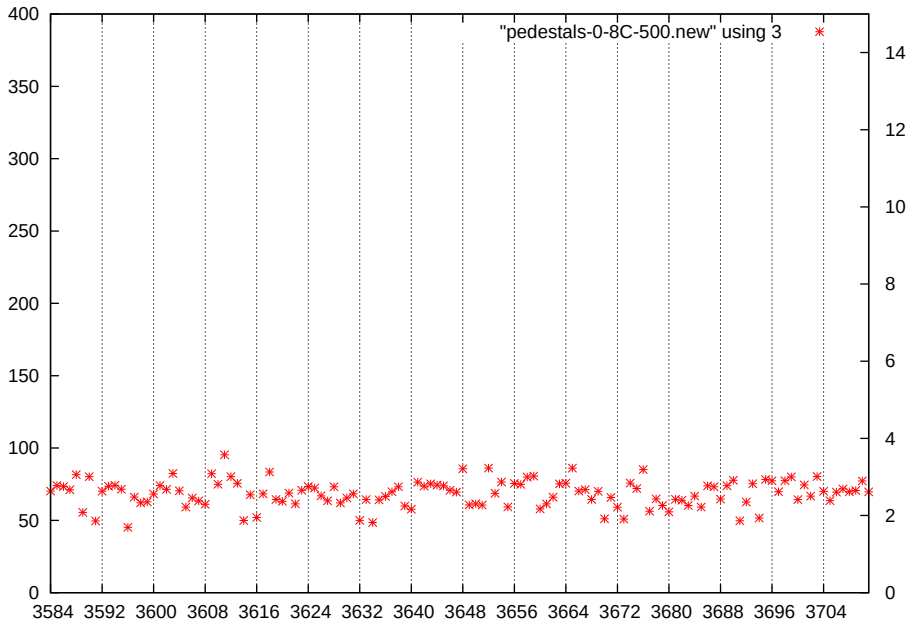
p1-gain2-shaper1-dac500
