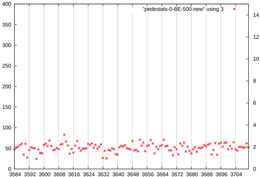
p1-gain3-shaper7-dac500
