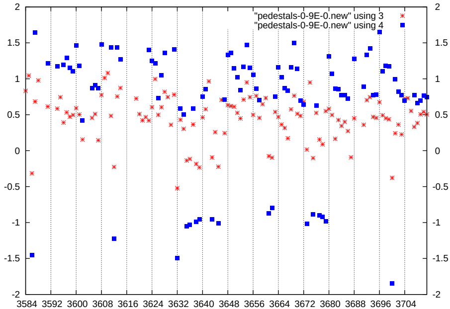
p1-gain3-shaper3-dac0
