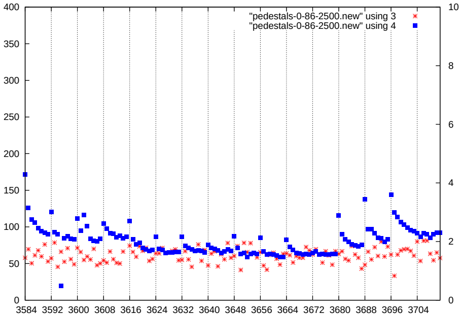
p1-gain3-shaper0-dac2500
