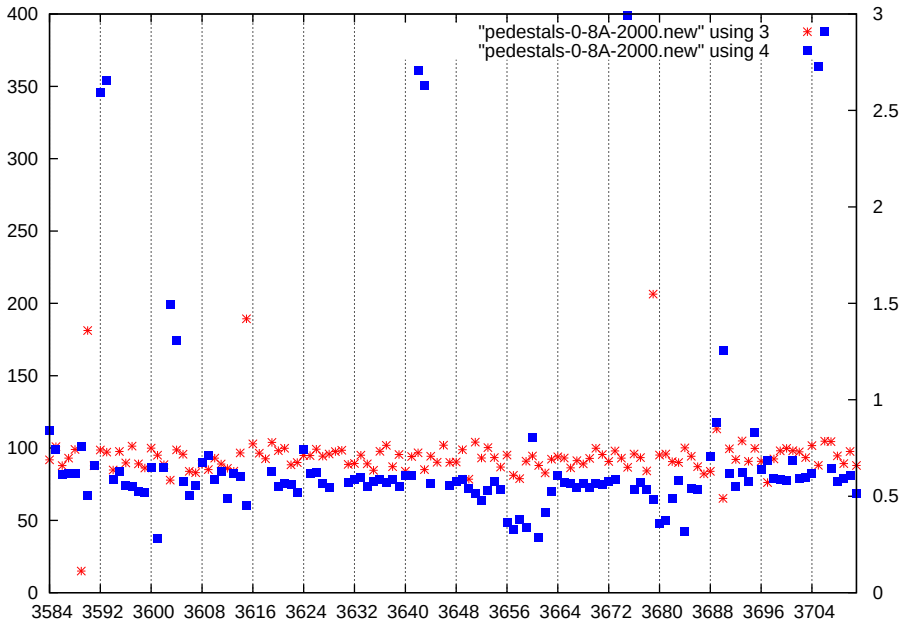
p1-gain1-shaper1-dac2000
