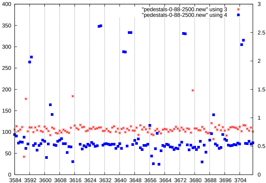
p1-gain0-shaper1-dac2500
