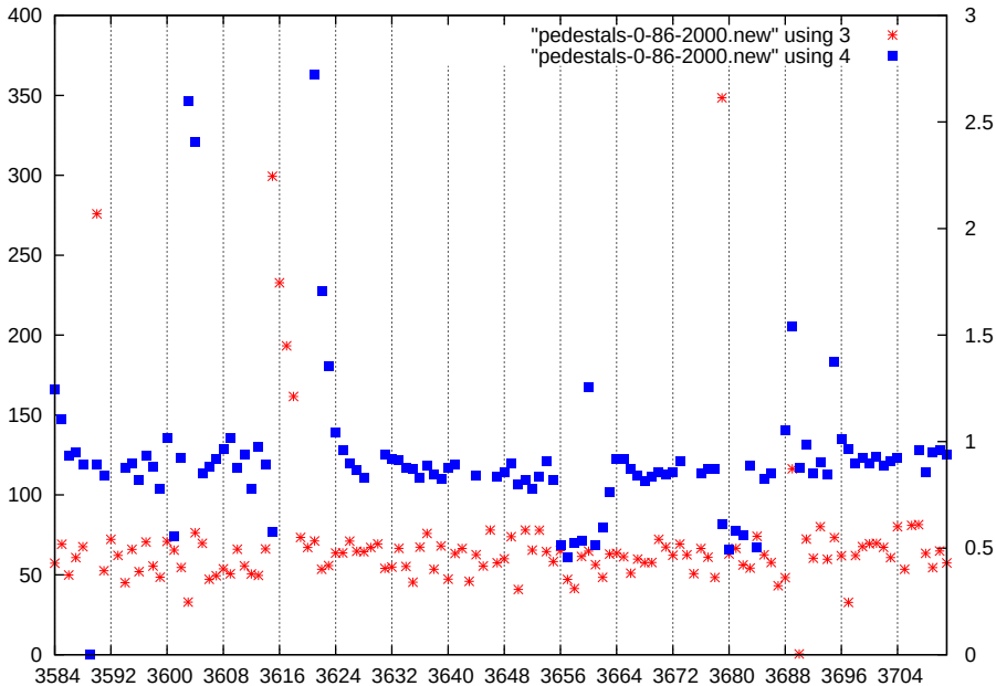
p1-gain3-shaper0-dac2000
