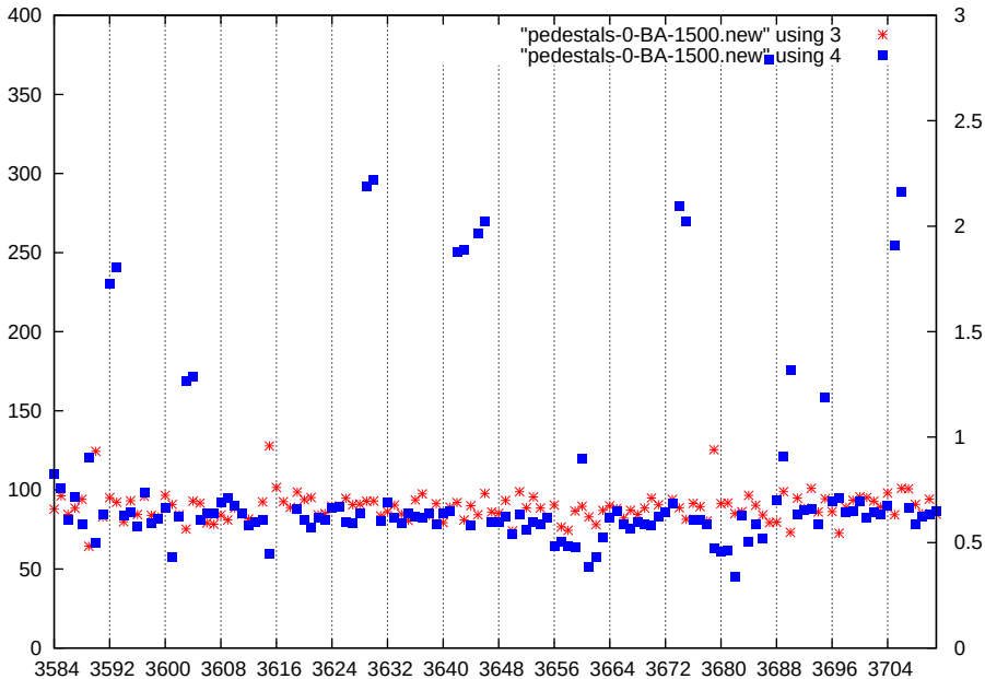
p1-gain1-shaper7-dac1500
