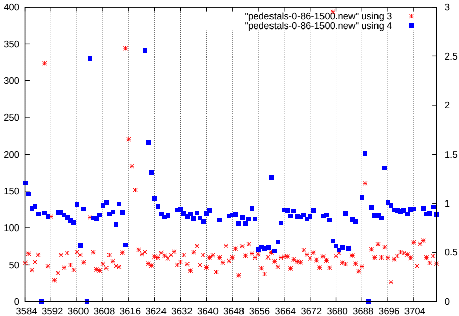
p1-gain3-shaper0-dac1500
