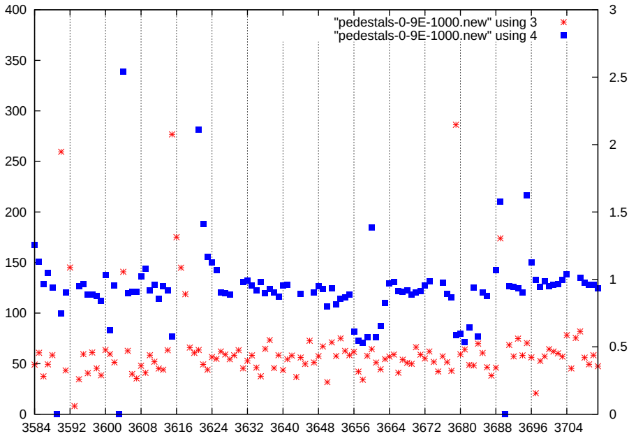
p1-gain3-shaper3-dac1000
