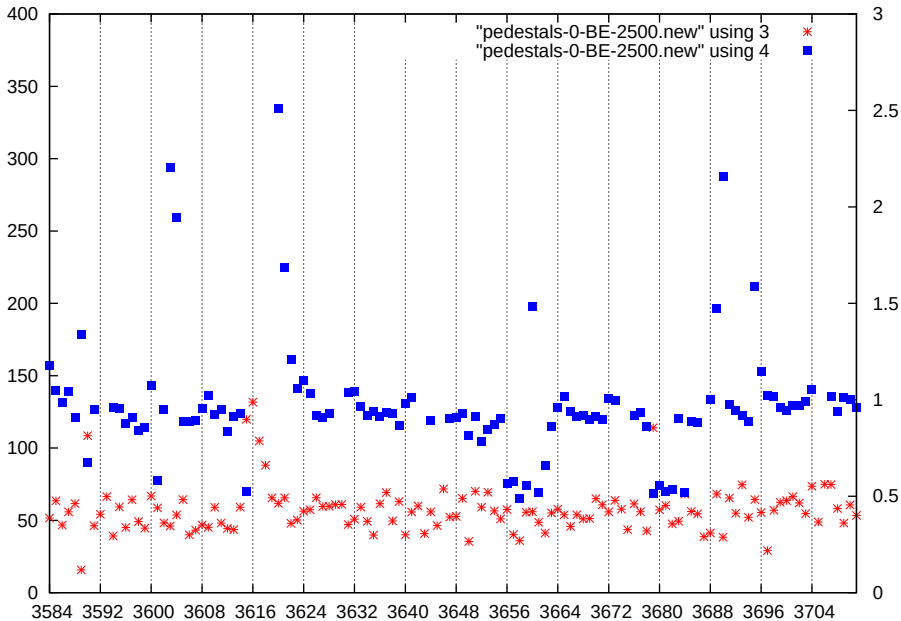
p1-gain3-shaper7-dac2500
