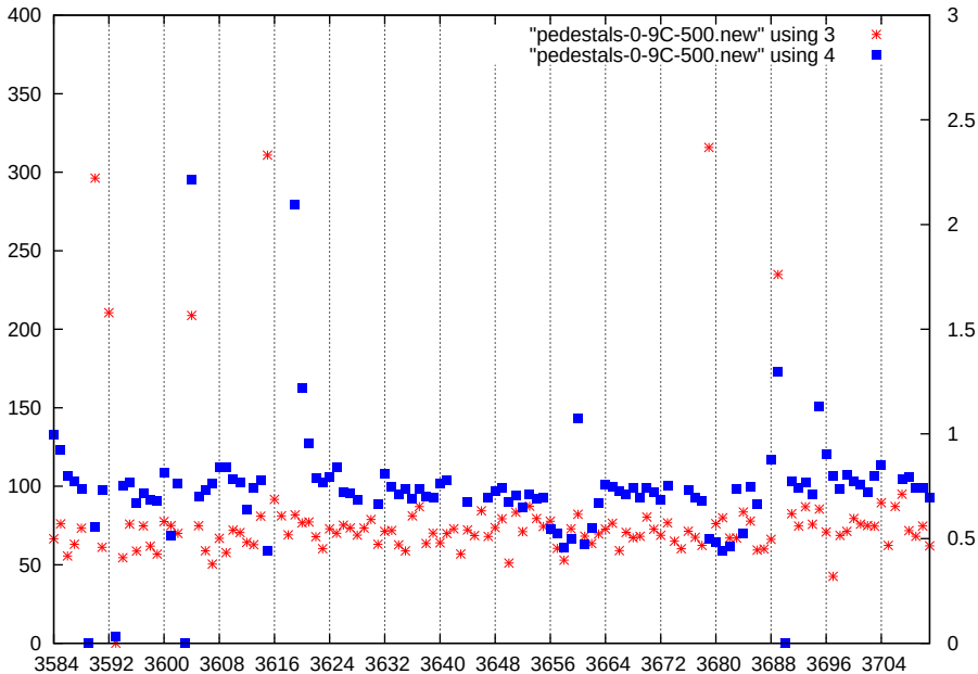
p1-gain2-shaper3-dac500
