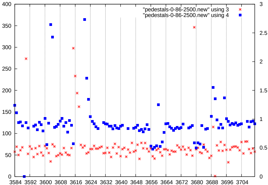
p1-gain3-shaper0-dac2500
