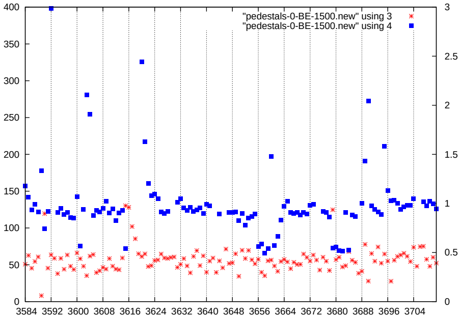
p1-gain3-shaper7-dac1500
