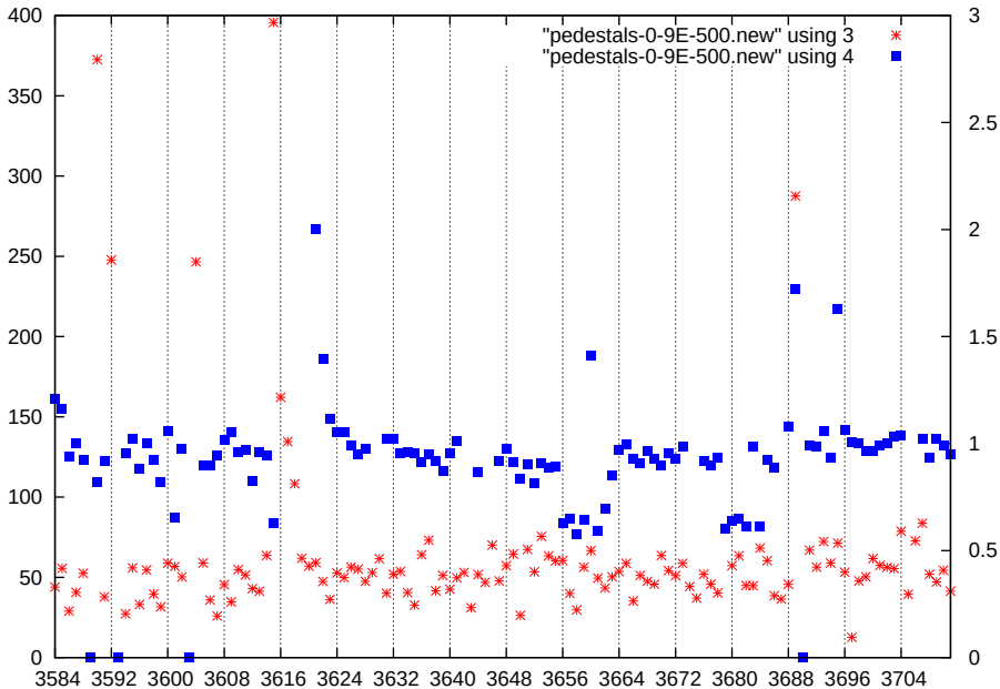
p1-gain3-shaper3-dac500
