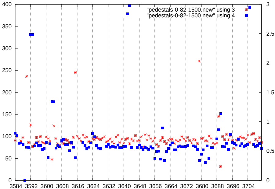
p1-gain1-shaper0-dac1500
