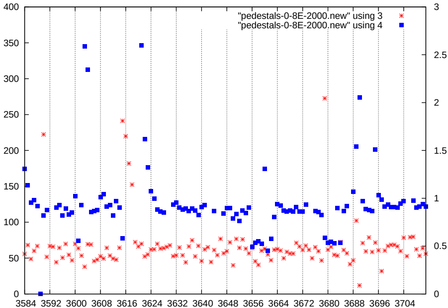
p1-gain3-shaper1-dac2000
