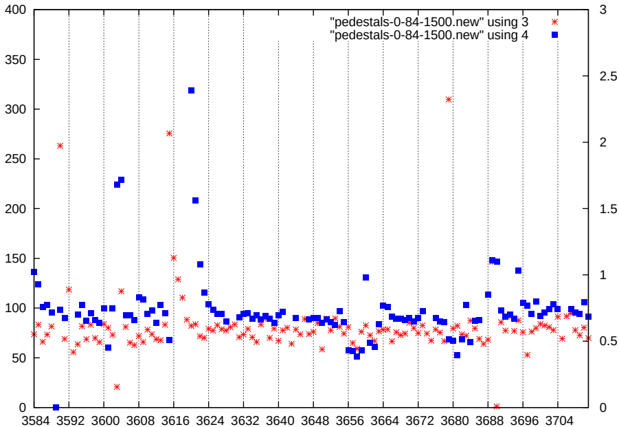
p1-gain2-shaper0-dac1500
