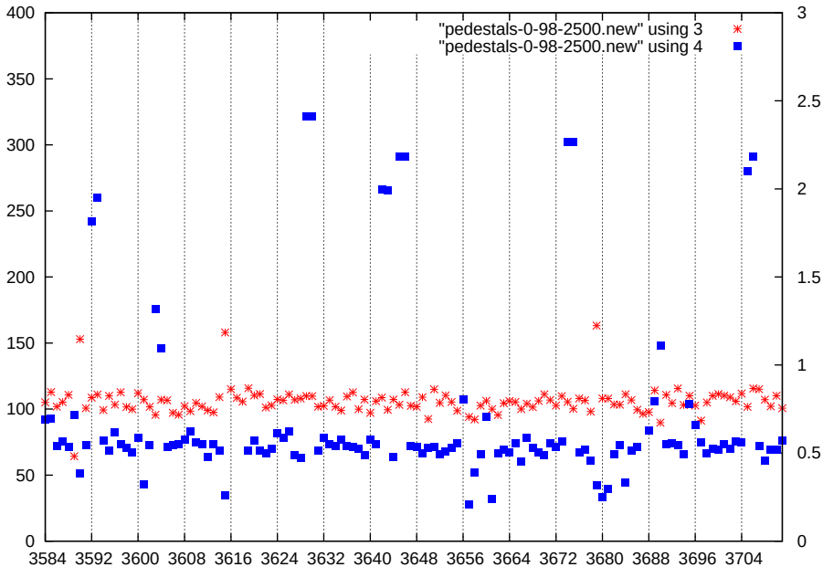
p1-gain0-shaper3-dac2500
