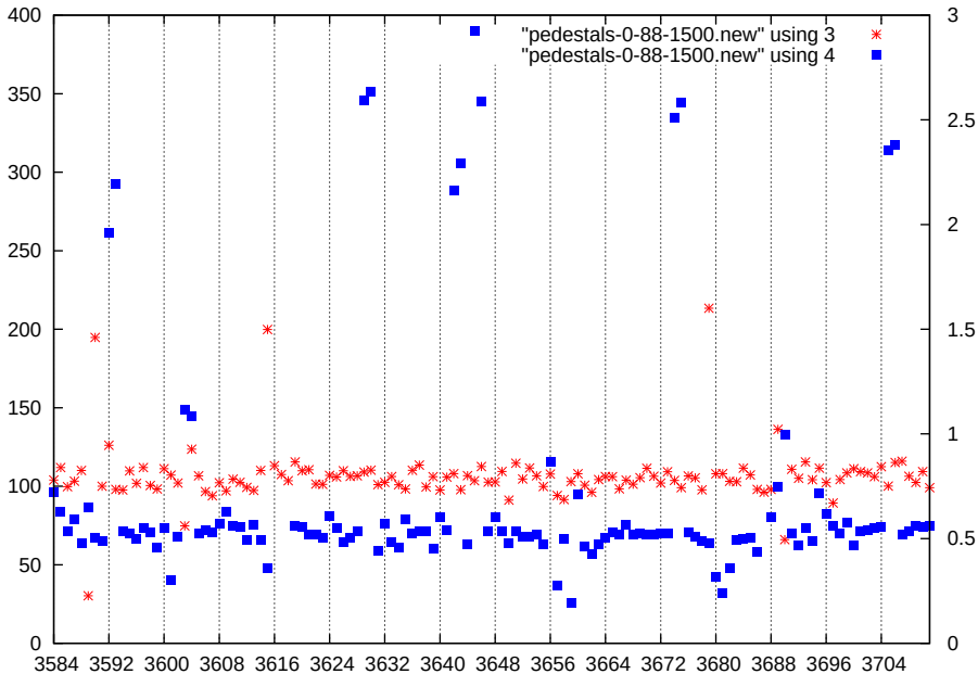
p1-gain0-shaper1-dac1500
