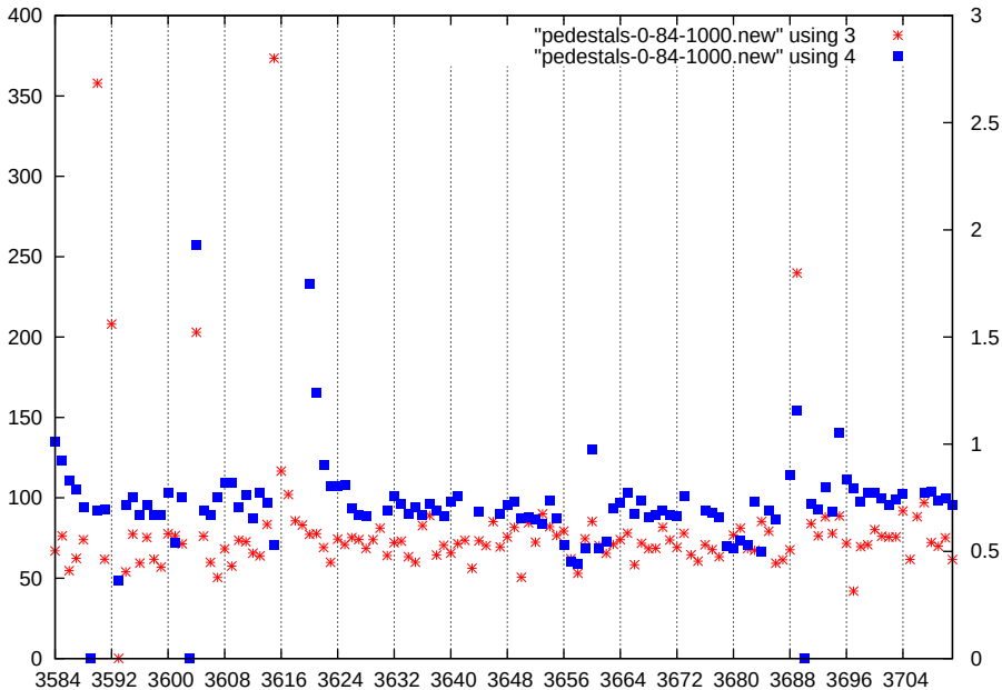
p1-gain2-shaper0-dac1000
