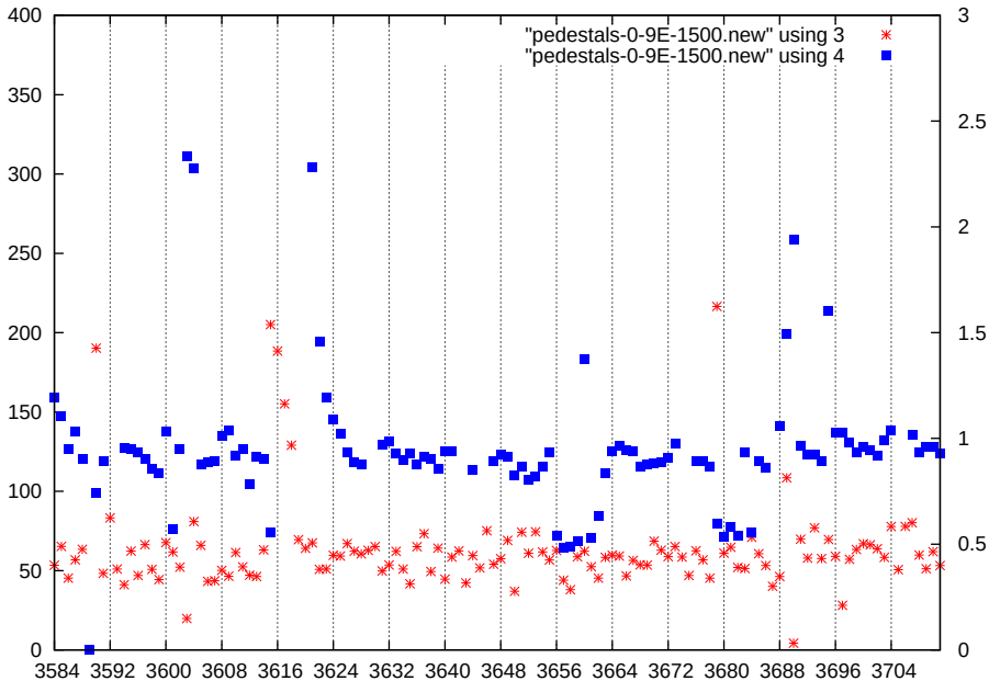
p1-gain3-shaper3-dac1500
