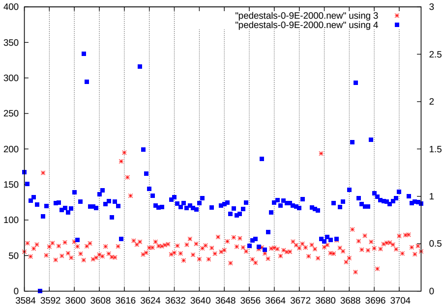
p1-gain3-shaper3-dac2000
