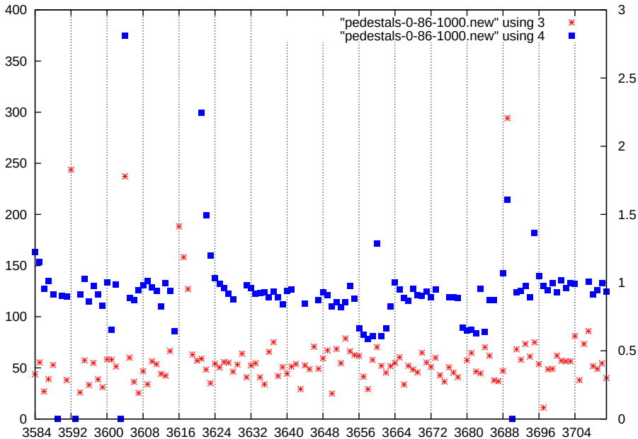
p1-gain3-shaper0-dac1000
