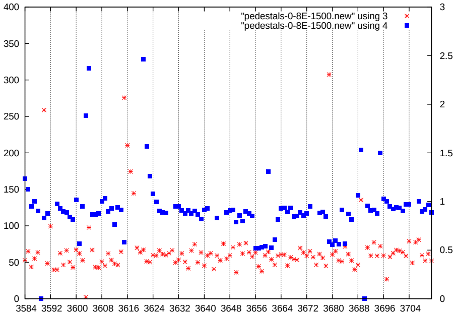
p1-gain3-shaper1-dac1500
