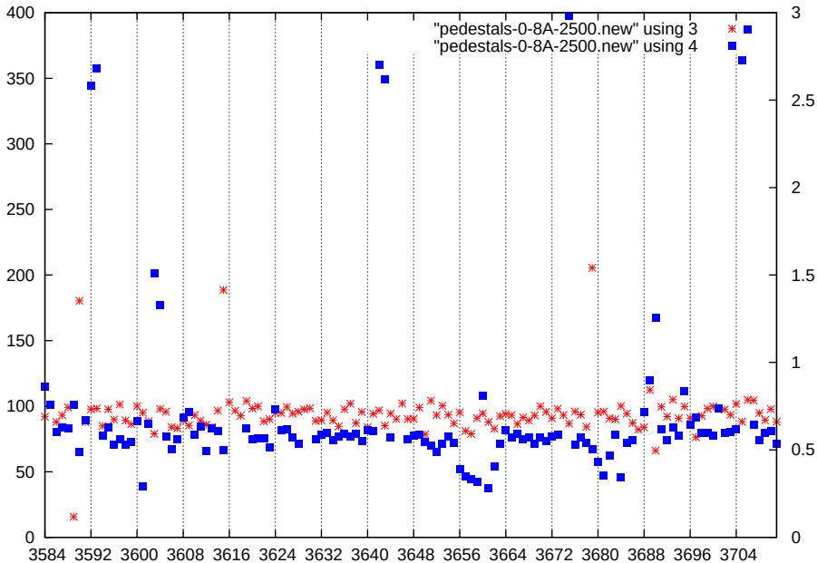
p1-gain1-shaper1-dac2500
