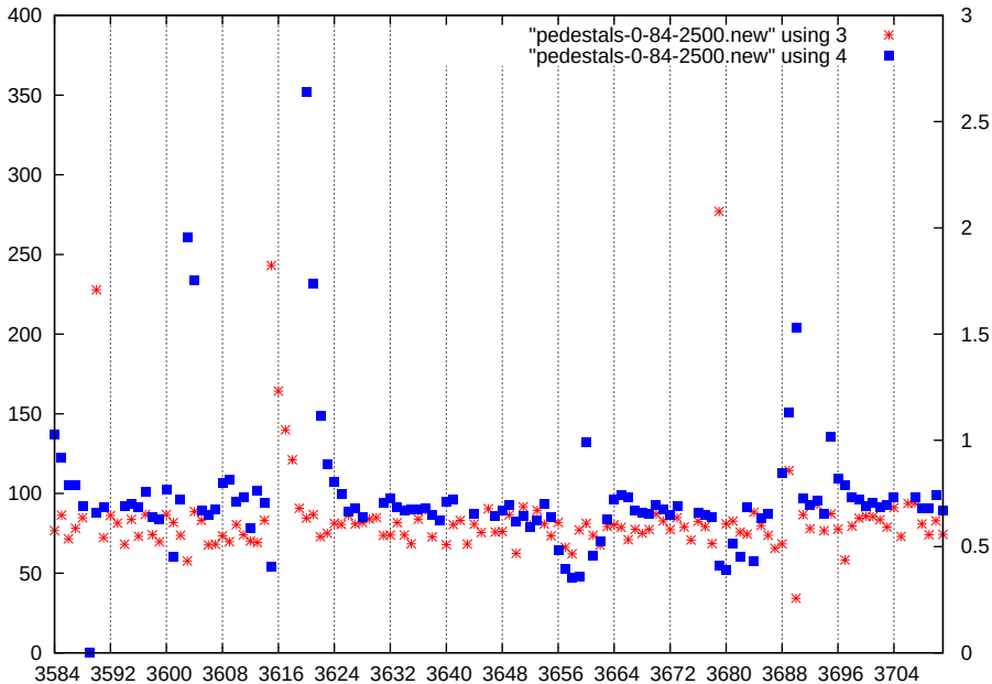
p1-gain2-shaper0-dac2500
