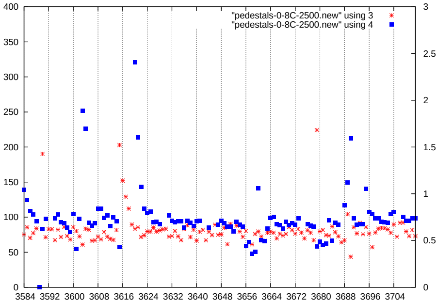
p1-gain2-shaper1-dac2500
