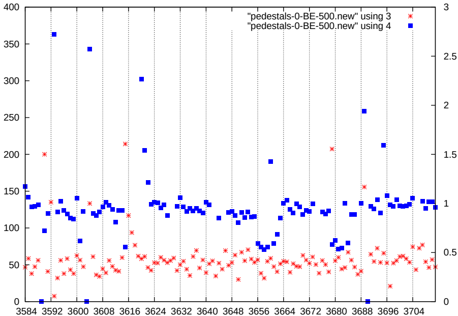
p1-gain3-shaper7-dac500
