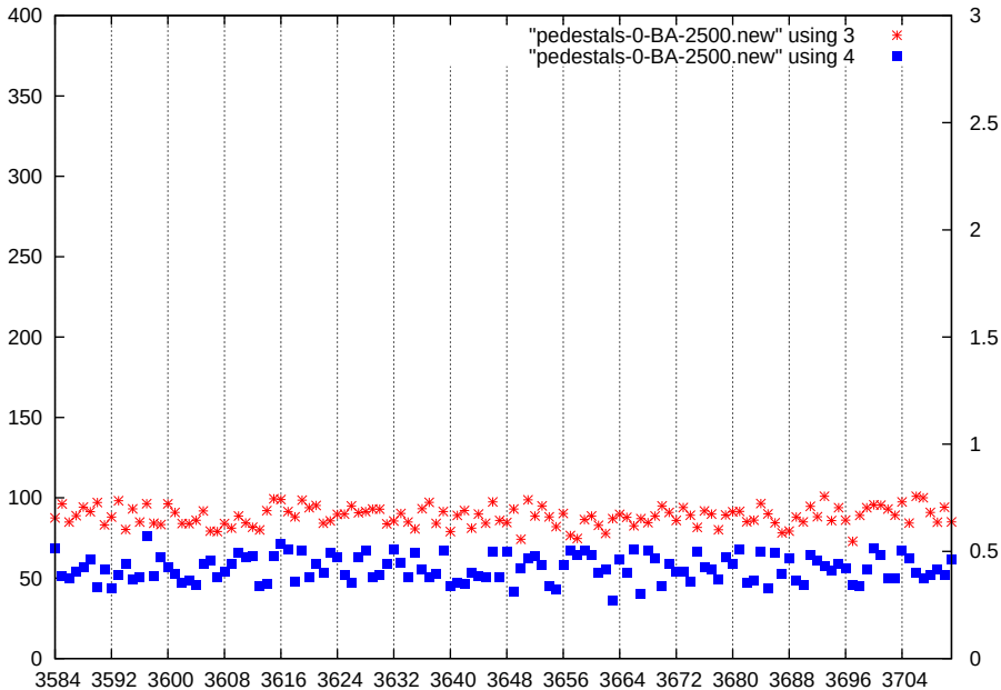
p1-gain1-shaper7-dac2500
