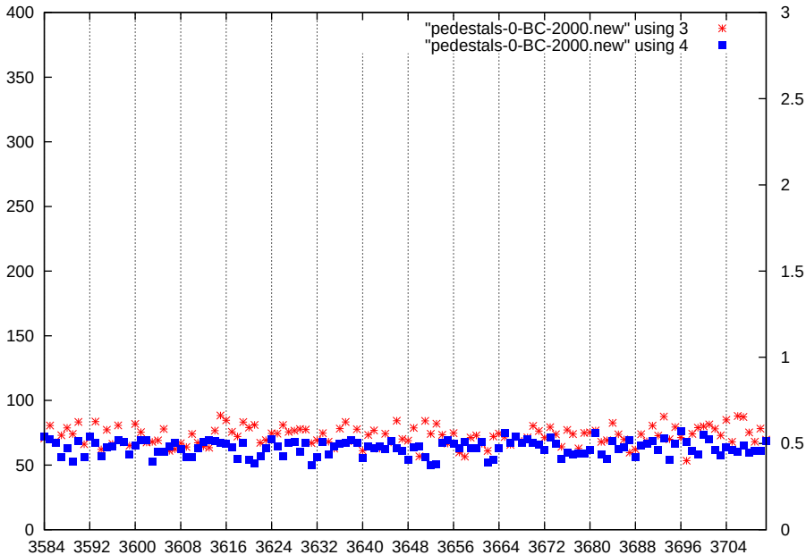
p1-gain2-shaper7-dac2000
