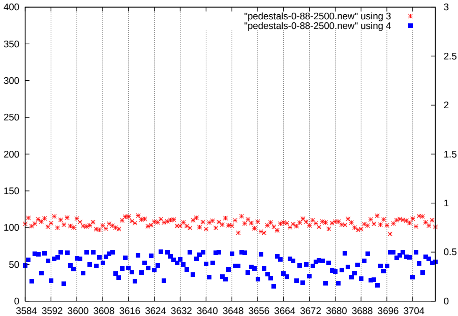
p1-gain0-shaper1-dac2500
