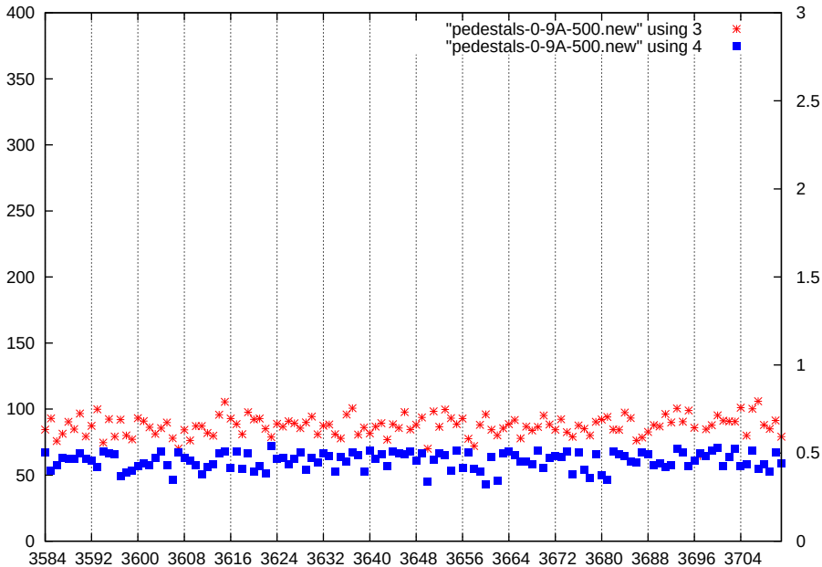
p1-gain1-shaper3-dac500
