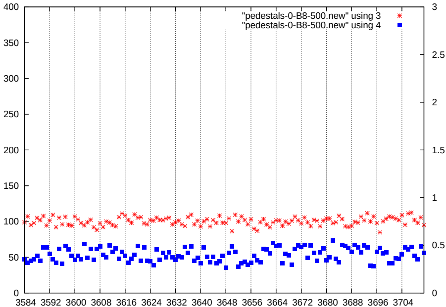
p1-gain0-shaper7-dac500
