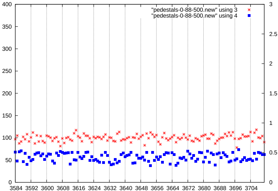
p1-gain0-shaper1-dac500
