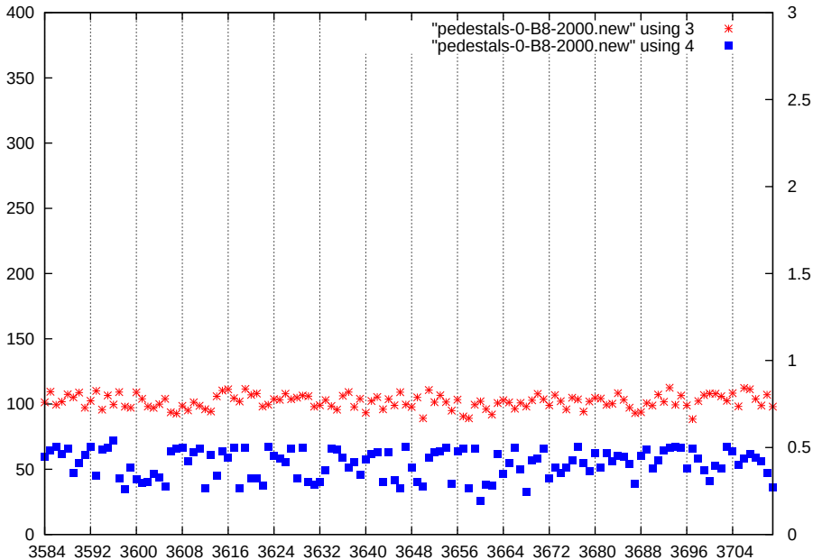
p1-gain0-shaper7-dac2000
