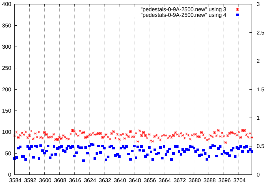
p1-gain1-shaper3-dac2500
