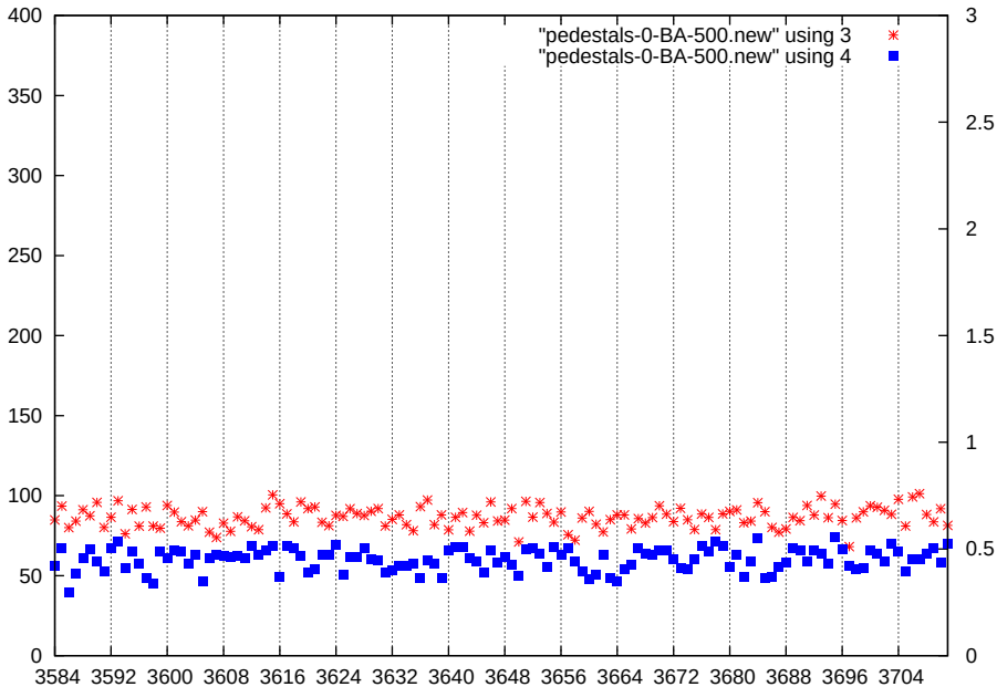
p1-gain1-shaper7-dac500
