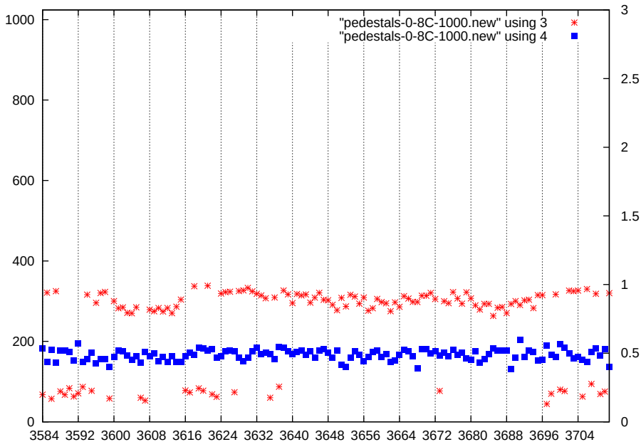
p1-gain2-shaper1-dac1000
