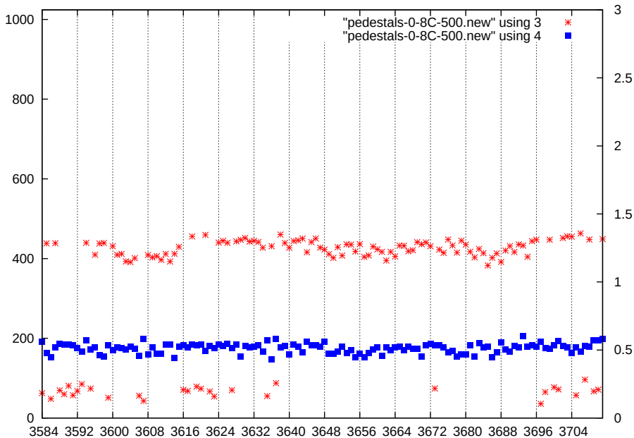
p1-gain2-shaper1-dac500
