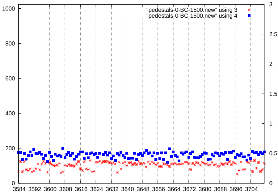
p1-gain2-shaper7-dac1500
