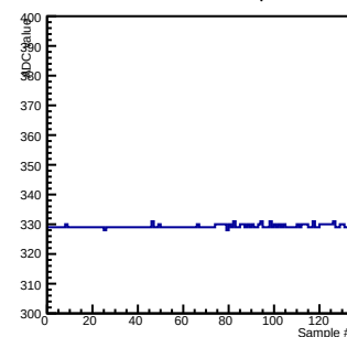
Run 33696 Event 3 Chip 1005
