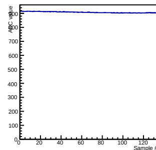
Run 33785 Event 9 Chip 10063
