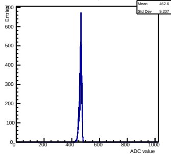
Pedestals ch 0 chip 2007 test
