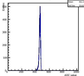
Pedestals ch 10 chip 2007 test
