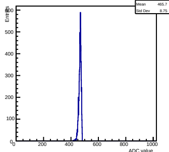
Pedestals ch 12 chip 2007 test
