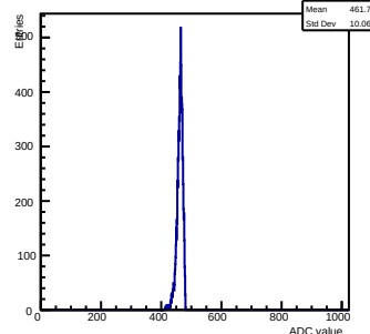
Pedestals ch 7 chip 2007 test
