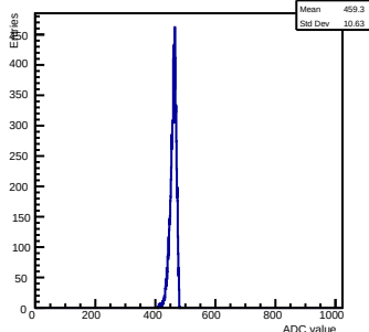
Pedestals ch 13 chip 2007 test
