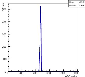
Pedestals ch 5 chip 2007 test
