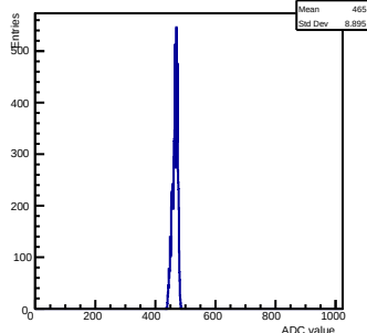
Pedestals ch 14 chip 2007 test
