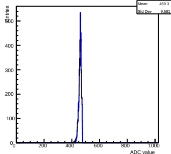
Pedestals ch 8 chip 2007 test
