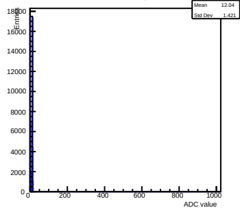
Pedestals ch 11 chip 2000 test
