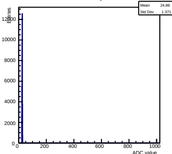
Pedestals ch 5 chip 2000 test
