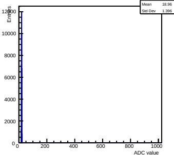
Pedestals ch 13 chip 2000 test
