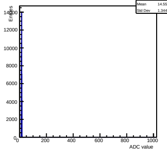
Pedestals ch 14 chip 2000 test
