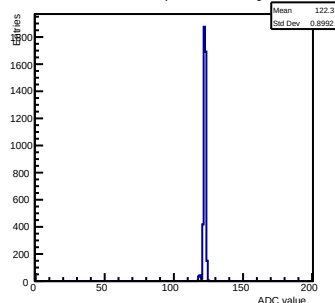
Pedestals ch 14 chip 2000 nominal-gain1
