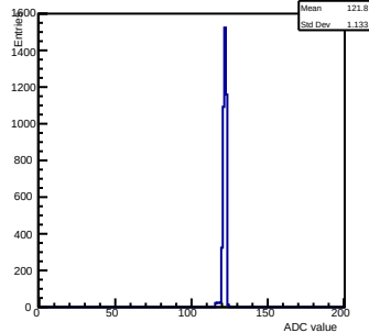
Pedestals ch 2 chip 2000 nominal-gain1
