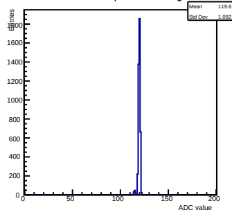
Pedestals ch 10 chip 2000 nominal-gain1
