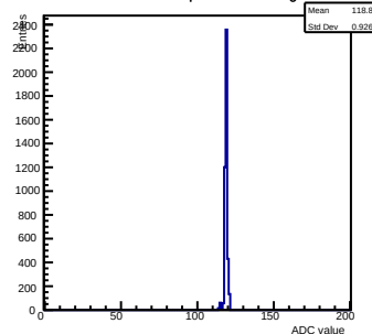
Pedestals ch 11 chip 2000 nominal-gain1
