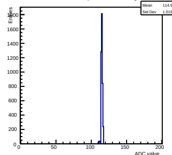
Pedestals ch 15 chip 2000 nominal-gain1
