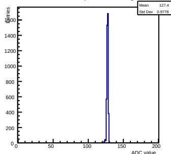
Pedestals ch 13 chip 2000 nominal-gain1
