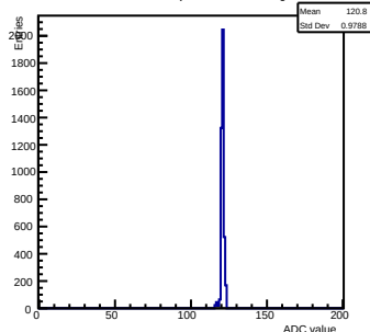
Pedestals ch 4 chip 2000 nominal-gain1
