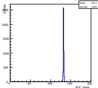
Pedestals ch 5 chip 2000 nominal-gain1
