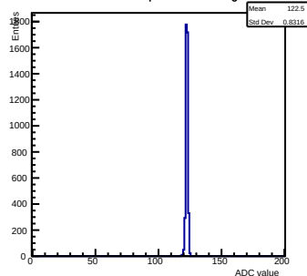
Pedestals ch 8 chip 2000 nominal-gain1
