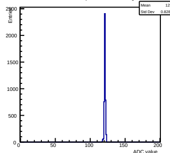
Pedestals ch 7 chip 2000 nominal-gain1
