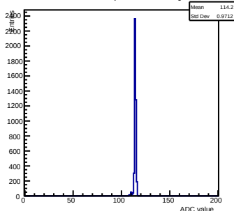
Pedestals ch 6 chip 2000 nominal-gain1
