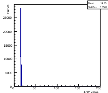
Pedestals ch 7 chip 2000 nominal-gain0
