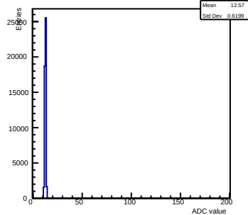
Pedestals ch 3 chip 2000 nominal-gain0
