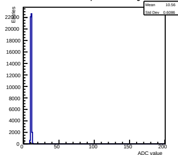
Pedestals ch 11 chip 2000 nominal-gain0
