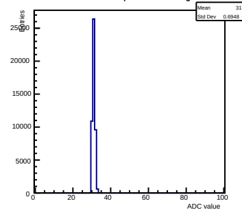
Pedestals ch 12 chip 2000 nominal-gain0
