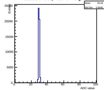
Pedestals ch 8 chip 2000 nominal-gain0
