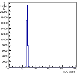
Pedestals ch 11 chip 2001 nominal-gain0
