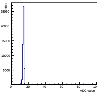
Pedestals ch 14 chip 2001 nominal-gain0
