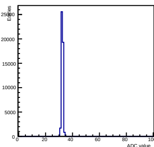
Pedestals ch 6 chip 2001 nominal-gain0
