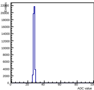
Pedestals ch 10 chip 2001 nominal-gain0
