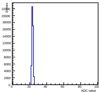
Pedestals ch 12 chip 2001 nominal-gain0
