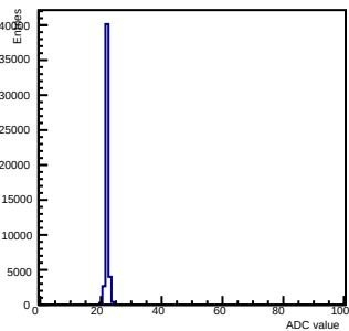
Pedestals ch 9 chip 2001 nominal-gain0
