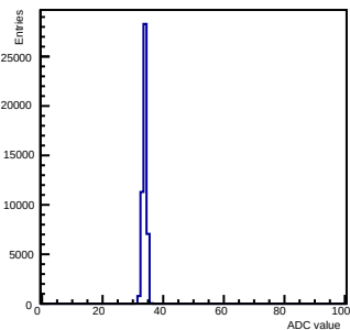
Pedestals ch 15 chip 2001 nominal-gain0
