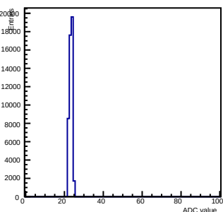
Pedestals ch 5 chip 2001 nominal-gain0
