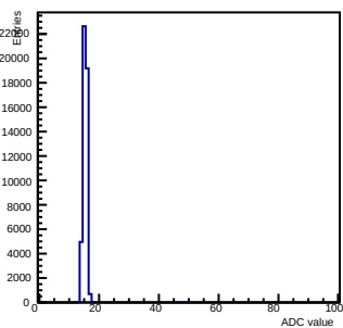
Pedestals ch 1 chip 2001 nominal-gain0
