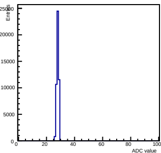
Pedestals ch 13 chip 2001 nominal-gain0
