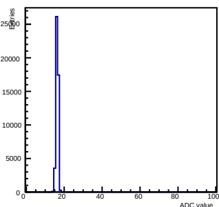
Pedestals ch 7 chip 2001 nominal-gain0
