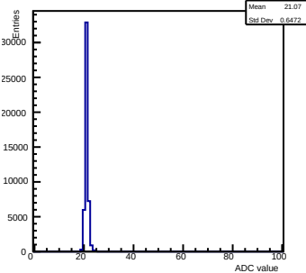
Pedestals ch 9 chip 2001 nominal-gain0
