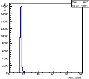
Pedestals ch 1 chip 2001 nominal-gain0
