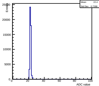
Pedestals ch 11 chip 2001 nominal-gain0
