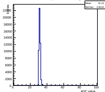
Pedestals ch 4 chip 2001 nominal-gain0
