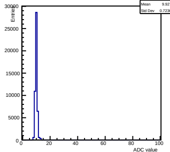
Pedestals ch 14 chip 2001 nominal-gain0
