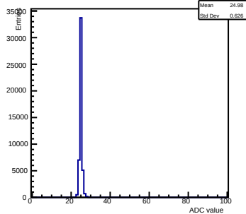
Pedestals ch 0 chip 2001 nominal-gain0
