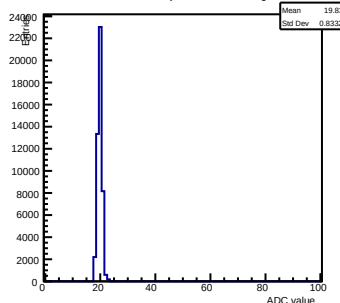
Pedestals ch 6 chip 2001 nominal-gain0
