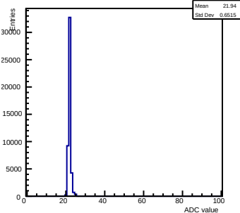
Pedestals ch 13 chip 2001 nominal-gain0
