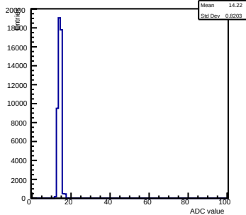
Pedestals ch 3 chip 2001 nominal-gain0
