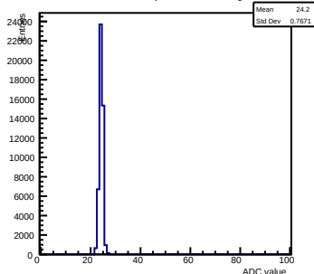
Pedestals ch 7 chip 2001 nominal-gain0
