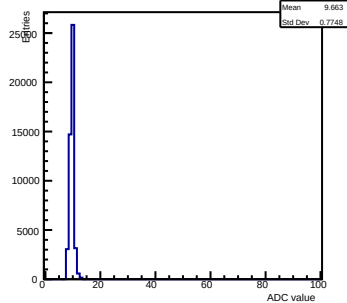
Pedestals ch 8 chip 2001 nominal-gain0
