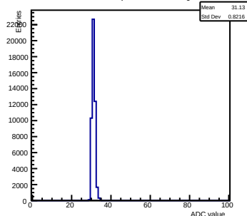
Pedestals ch 4 chip 2002 nominal-gain0
