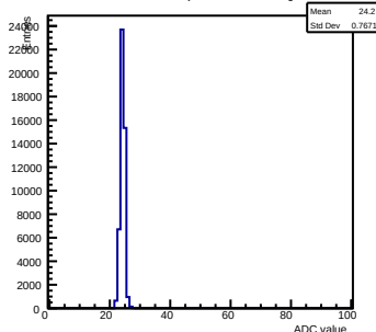
Pedestals ch 7 chip 2002 nominal-gain0
