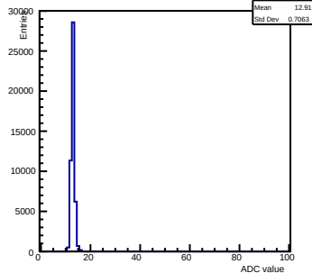
Pedestals ch 12 chip 2002 nominal-gain0
