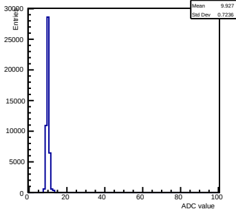
Pedestals ch 14 chip 2002 nominal-gain0
