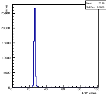
Pedestals ch 5 chip 2002 nominal-gain0
