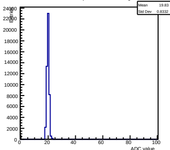
Pedestals ch 6 chip 2002 nominal-gain0
