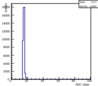
Pedestals ch 1 chip 2002 nominal-gain0
