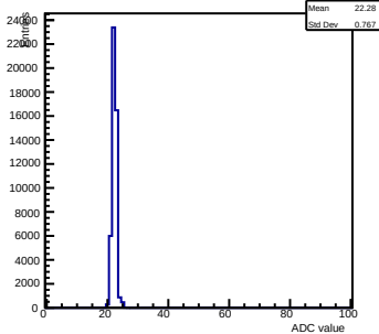
Pedestals ch 10 chip 2002 nominal-gain0
