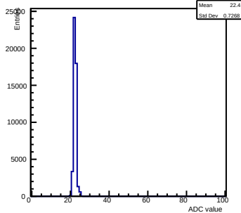
Pedestals ch 11 chip 2002 nominal-gain0
