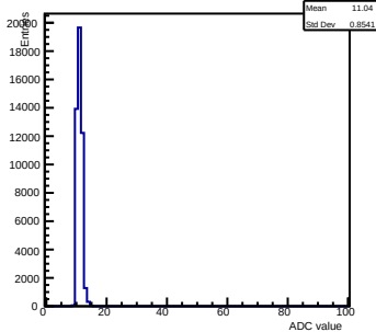
Pedestals ch 2 chip 2002 nominal-gain0
