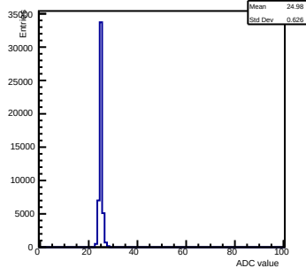
Pedestals ch 0 chip 2002 nominal-gain0
