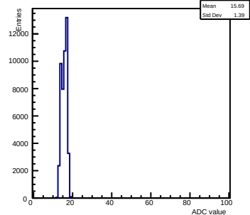
Pedestals ch 15 chip 2002 nominal-gain0
