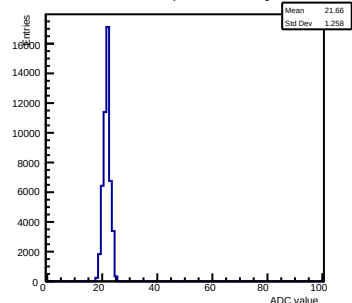
Pedestals ch 7 chip 2002 nominal-gain0
