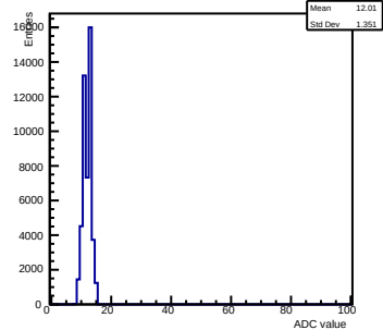
Pedestals ch 3 chip 2002 nominal-gain0
