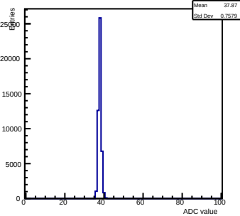
Pedestals ch 0 chip 2006 nominal-gain0
