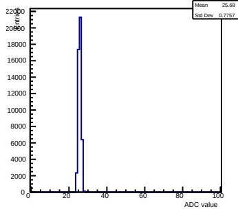
Pedestals ch 1 chip 2006 nominal-gain0
