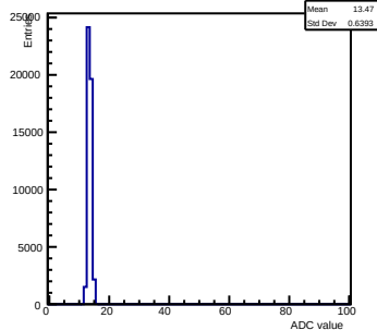
Pedestals ch 6 chip 2006 nominal-gain0
