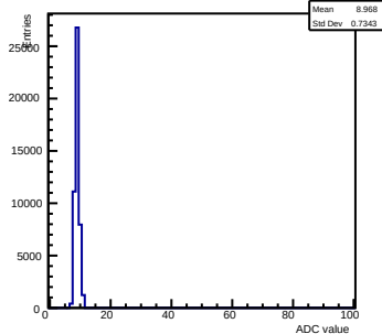
Pedestals ch 7 chip 2006 nominal-gain0
