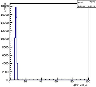
Pedestals ch 8 chip 2006 nominal-gain0
