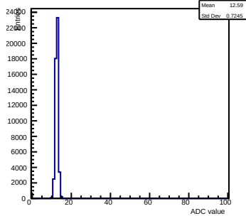
Pedestals ch 9 chip 2006 nominal-gain0
