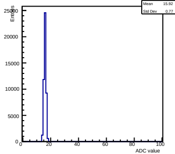
Pedestals ch 3 chip 2006 nominal-gain0
