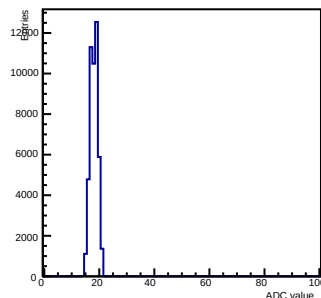
Pedestals ch 6 chip 2000 nominal-gain0
