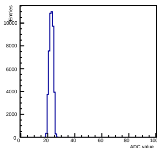
Pedestals ch 13 chip 2000 nominal-gain
