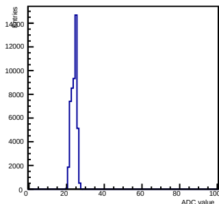
Pedestals ch 5 chip 2000 nominal-gain0
