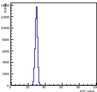
Pedestals ch 4 chip 2000 nominal-gain0
