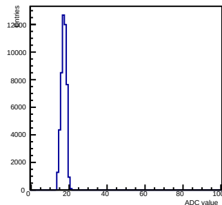
Pedestals ch 11 chip 2000 nominal-gain
