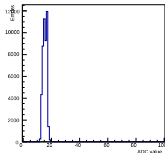
Pedestals ch 7 chip 2000 nominal-gain0
