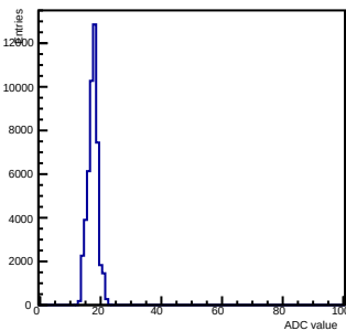
Pedestals ch 0 chip 2000 nominal-gain0
