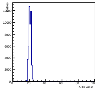
Pedestals ch 10 chip 2000 nominal-gain
