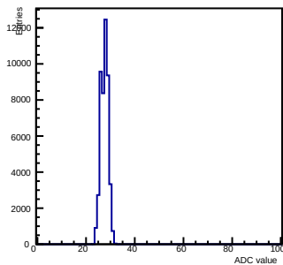
Pedestals ch 1 chip 2000 nominal-gain0
